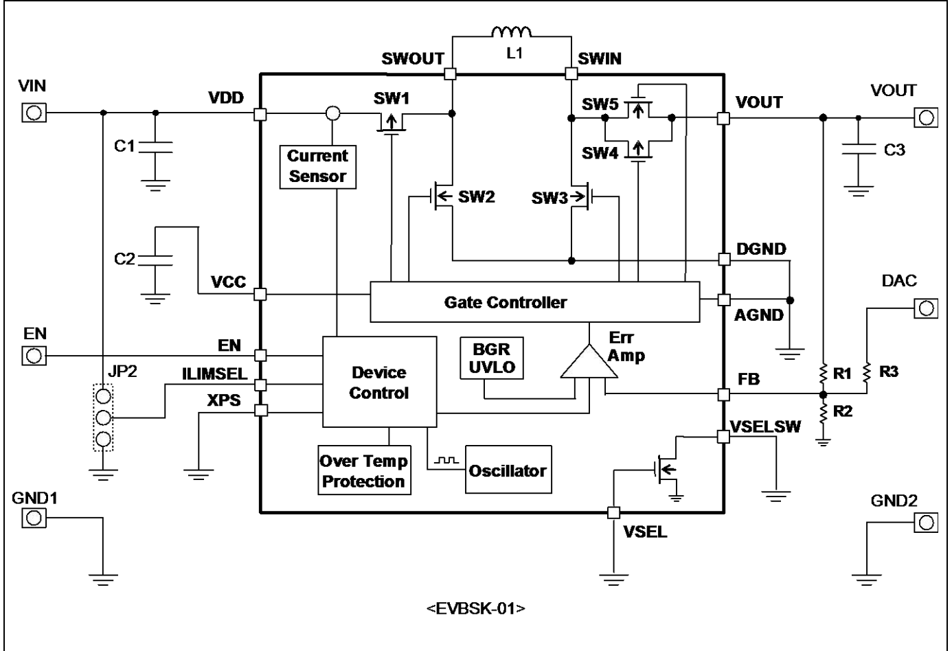
Figure 3-1 Block Diagram for EVBSK-01
