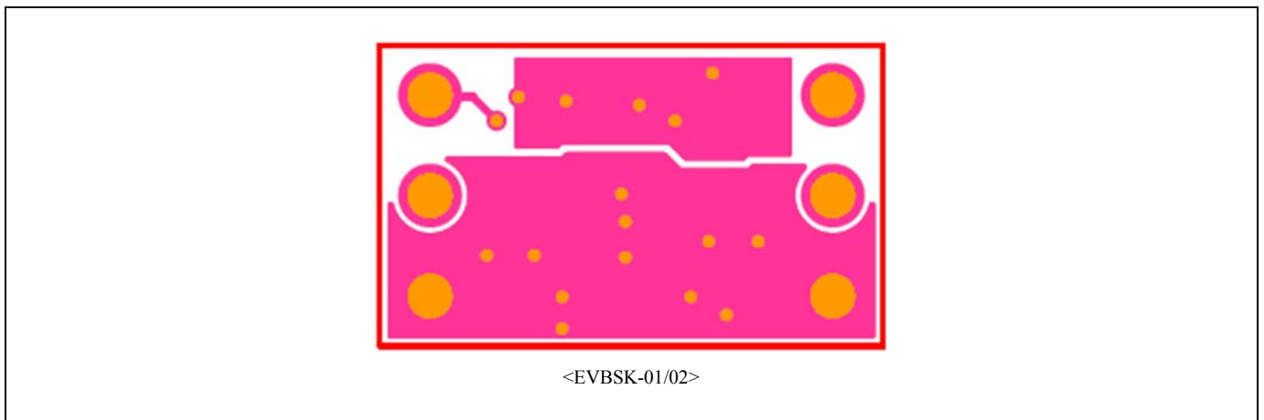
Figure 5-4 Wiring Layout (Layer 2, Top View)
