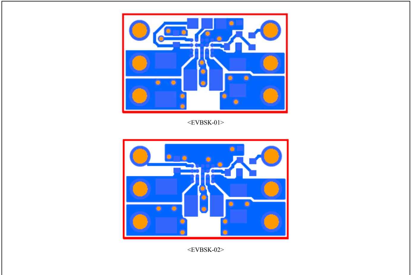
Figure 5-3 Wiring Layout (Layer 1)
