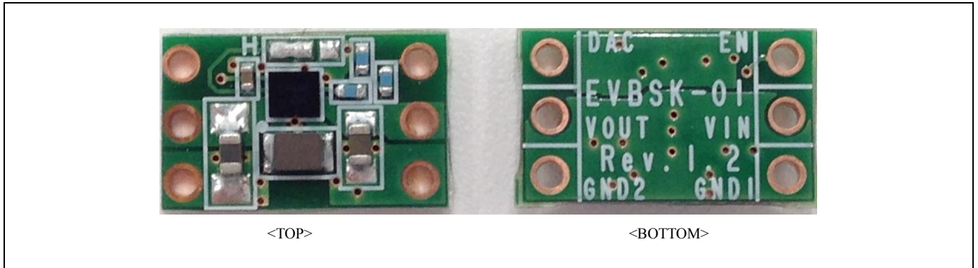
Figure 8-1 Picture of MB39C326-EVBSK-01
