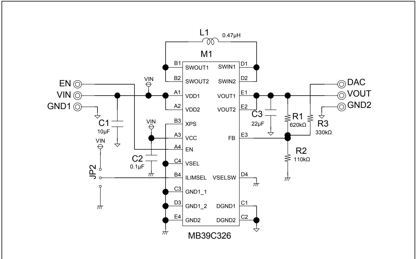
Figure 6-1 Schematic Circuit for Power Save Mode
