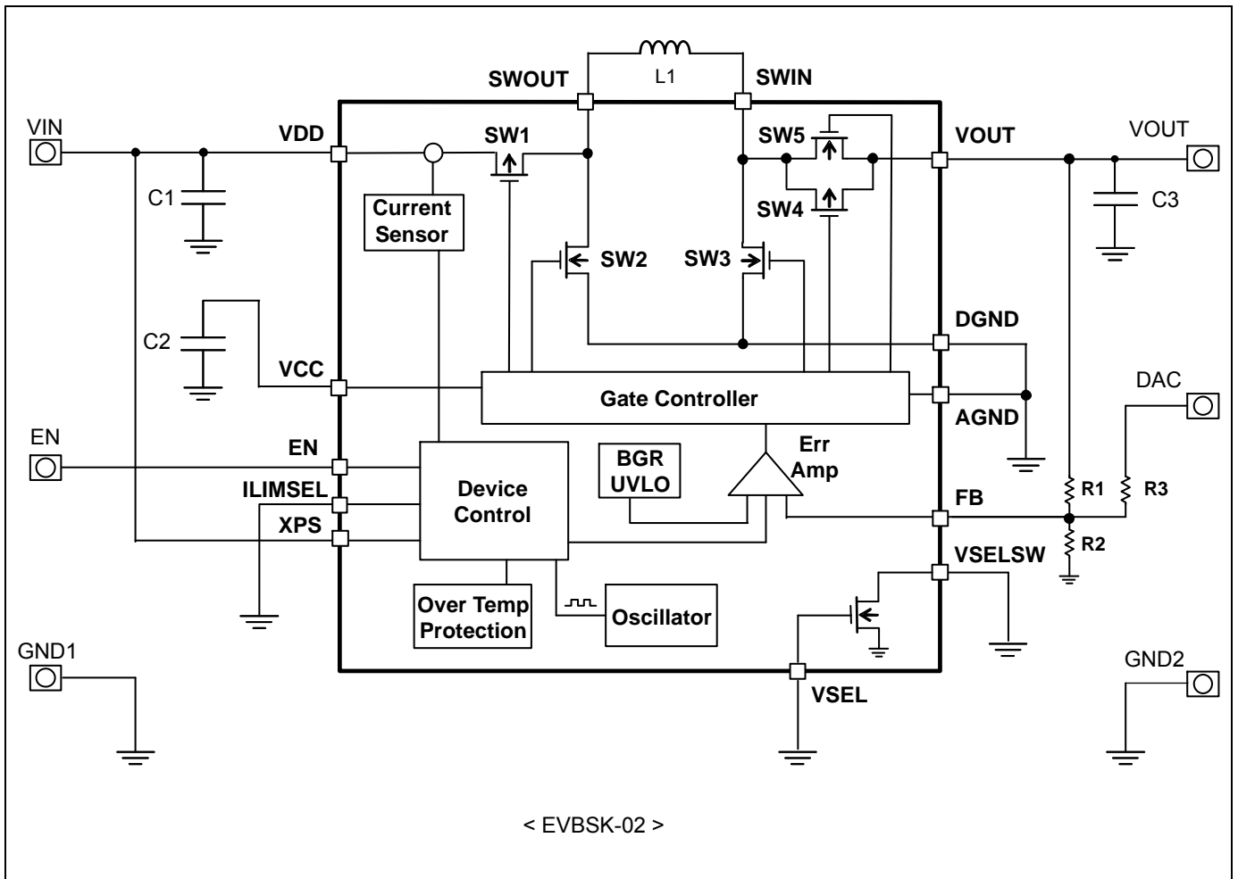
Figure 3-2 Block Diagram for EVBSK-02
