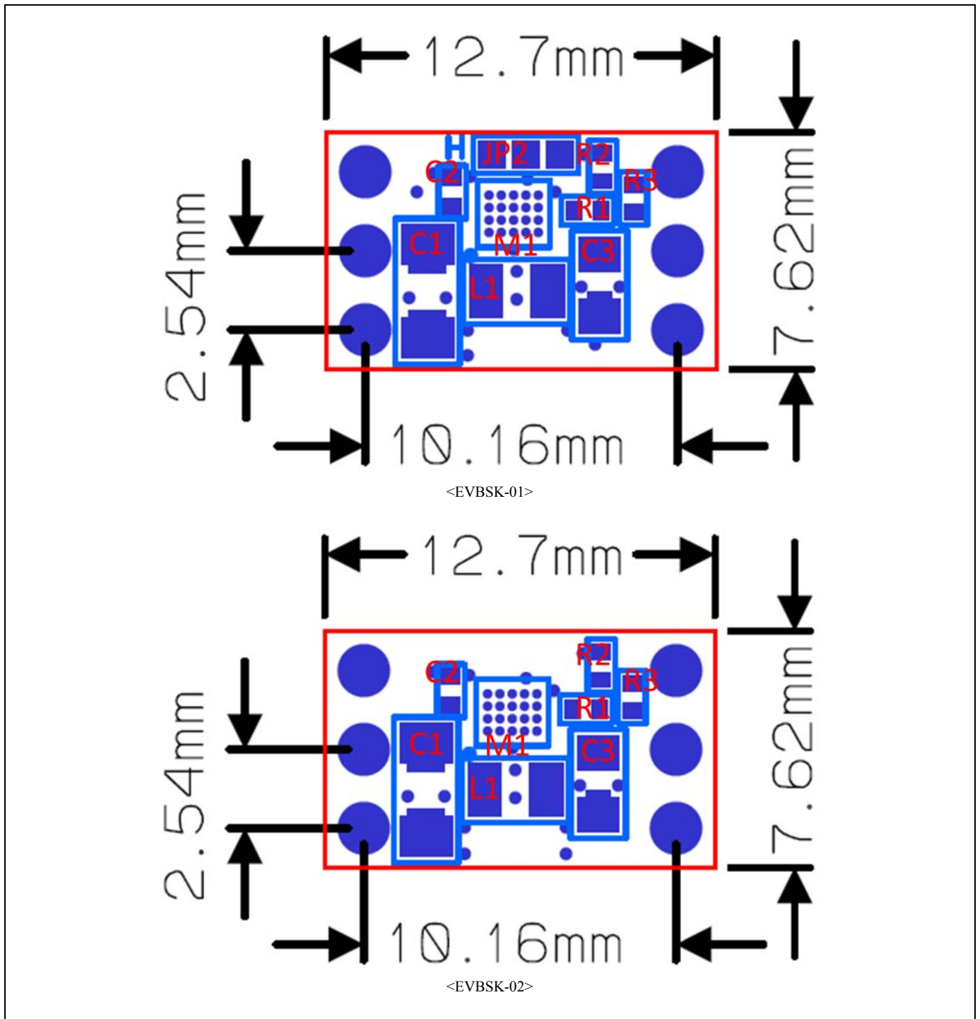
Figure 5-1 Component Layout (Layer 1)
