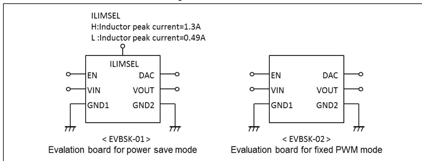
Figure 1-1 Board Outline
