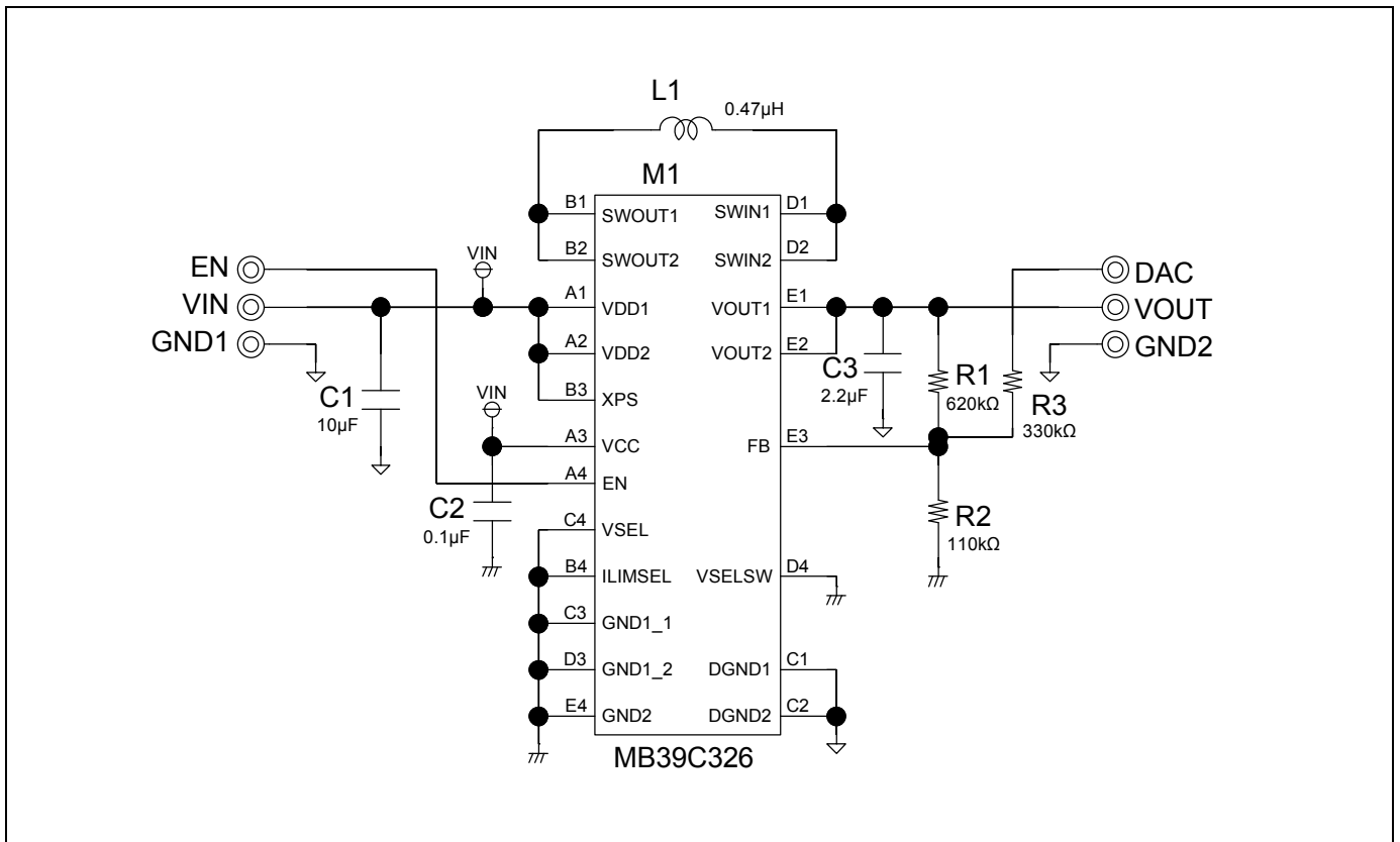
Figure 6-2 Schematic Circuit for Fixed PWM Mode
