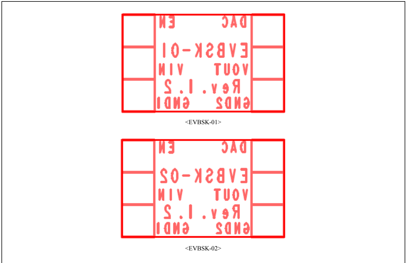
Figure 5-2 Component Layout (Layer 2, Top View)
