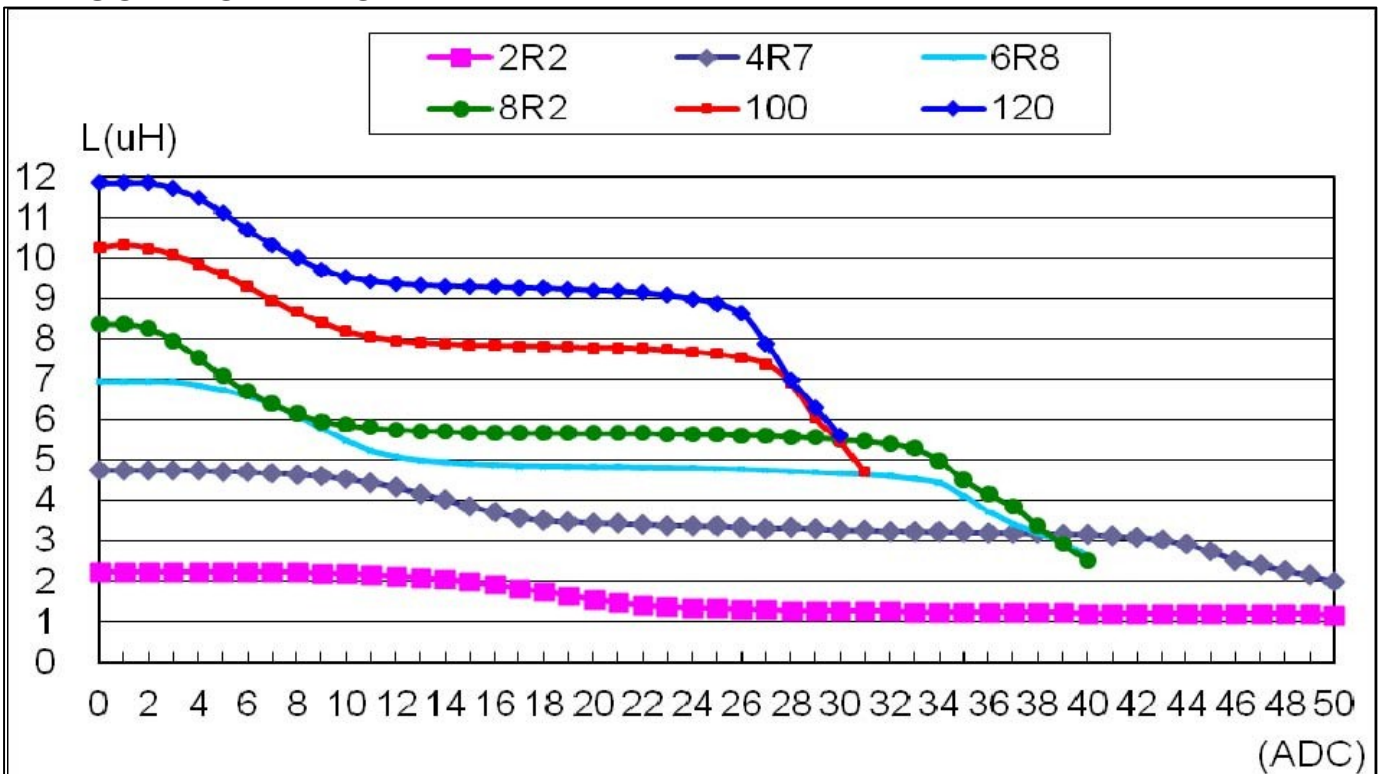
INDUCTANCE vs DC BIAS :
