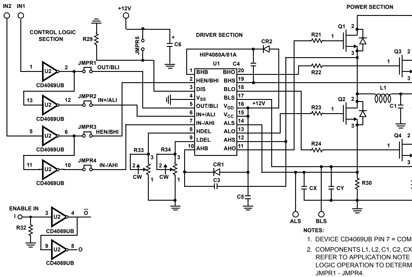
FIGURE 31. HIP4081A EVALUATION PC BOARD SCHEMATIC
