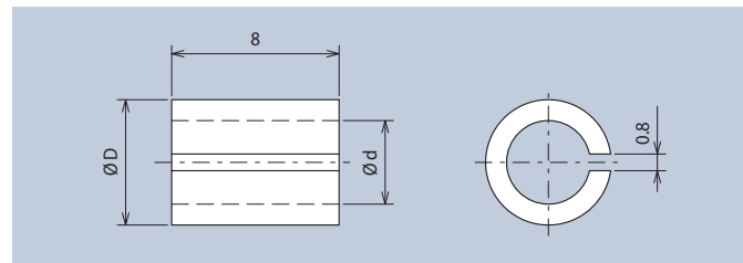
Reducing Sleeve Brass zinc plated
