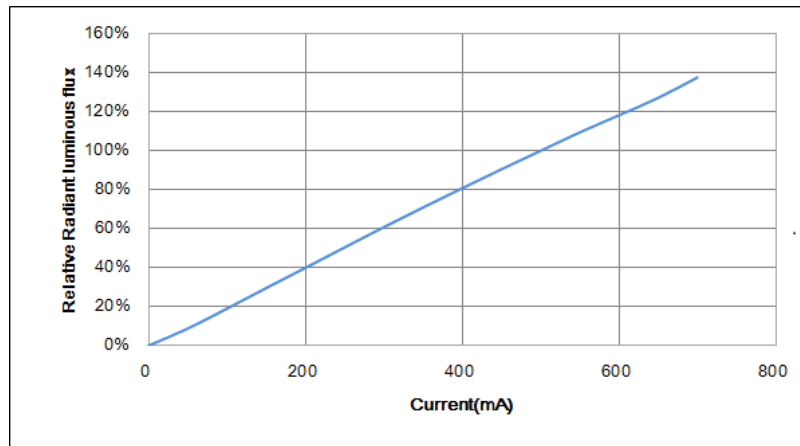
Fig 1. Typical relative Radiant flux vs. forward current of LTPL-U034UVH365
