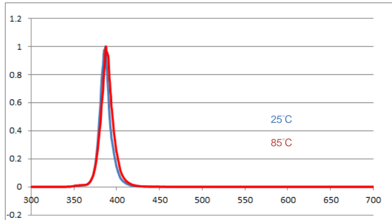
Fig 2. Relative Spectral Distribution at Tj = 25°C & 85°C
