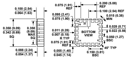
Figure 47. 20-Terminal Ceramic Leadless Chip Carrier [LCC] RC-Suffix (E-20-1) Dimensions shown in inches and (millimeters)
