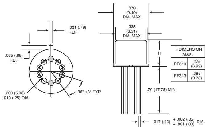
EXTERNAL DIMENSIONS
