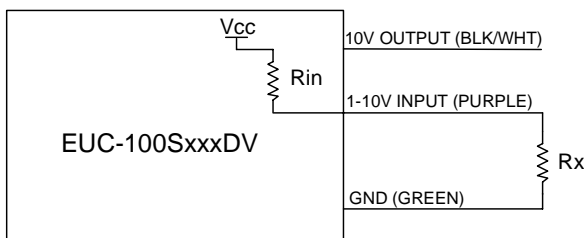
Implementation 2: External resistor (Vcc=12V) [EUC-100S315DV & EUC-100S420DV]
