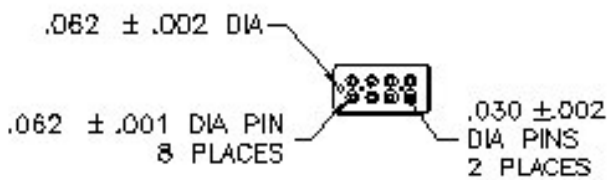
TERMINAL TYPE 4 FINISH CASE: TIN/LEAD PLATE TERMINALS: GOLD PLATED POLARIZING PIN: TIN/LEAD PLATE
