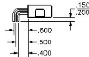
TERMINAL TYPE 7 FINISH CASE: TIN/LEAD PLATE TERMINALS: TIN/LEAD PLATE
