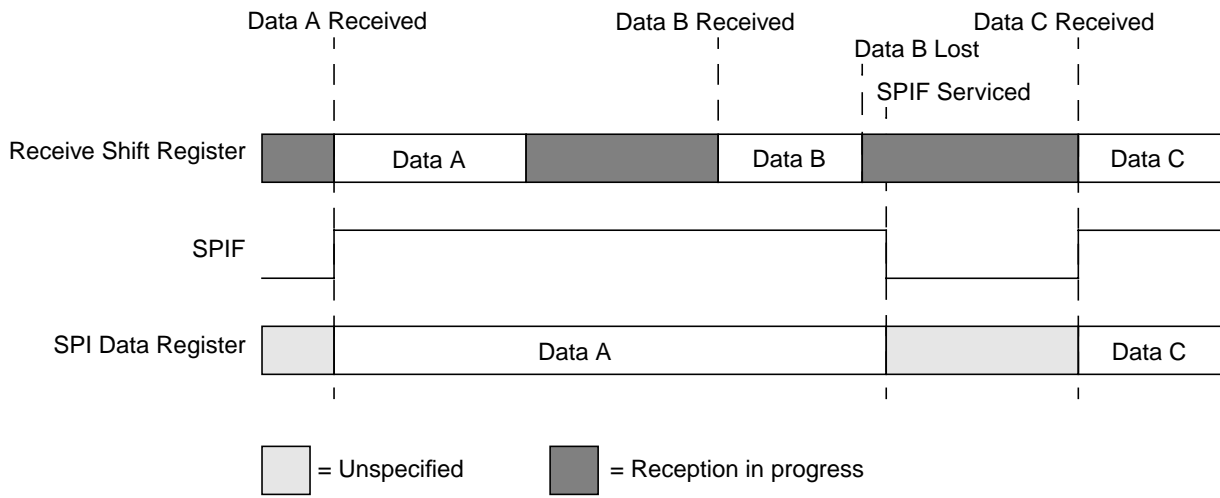
Figure 12-9. Reception with SPIF Serviced too Late
