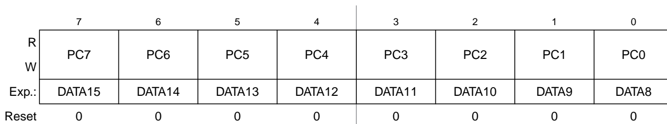
Figure 22-7. Port C Data Register (PORTC)
