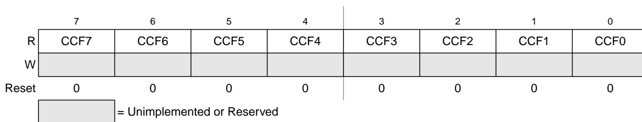
Figure 4-13. ATD Status Register 1 (ATDSTAT1)
