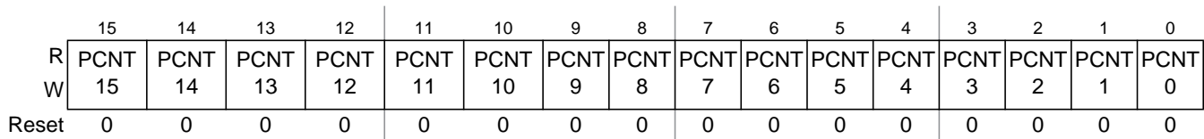
Figure 13-16. PIT Count Register 1 (PITCNT1)
