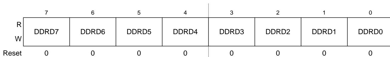
Figure 22-10. Port D Data Direction Register (DDR)
