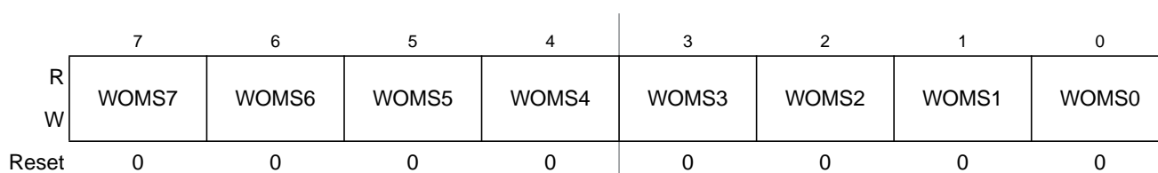
Figure 23-31. Port S Wired-OR Mode Register (WOMS)
