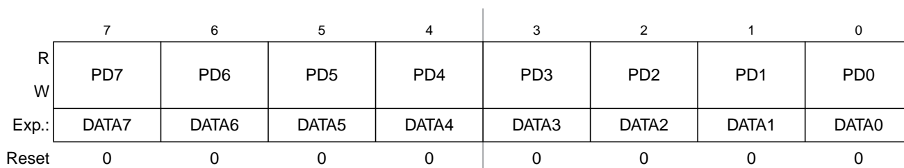
Figure 22-8. Port D Data Register (PORTD)
