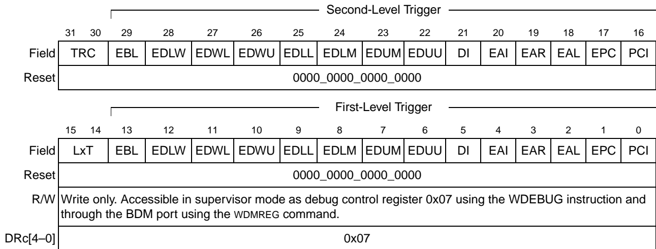
Figure 30-11. Trigger Definition Register (TDR)
