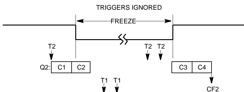
Figure 28-37. . CCW Freeze Situation 15
