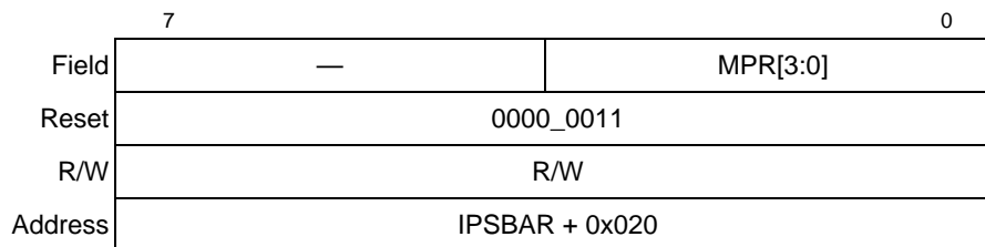
Figure 8-8. Master Privilege Register (MPR)
