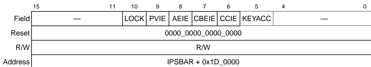
Figure 6-4. CFM Module Configuration Register (CFMCR)
