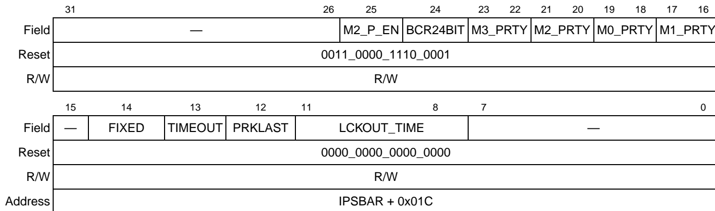
Figure 8-7. Default Bus Master Park Register (MPARK)
