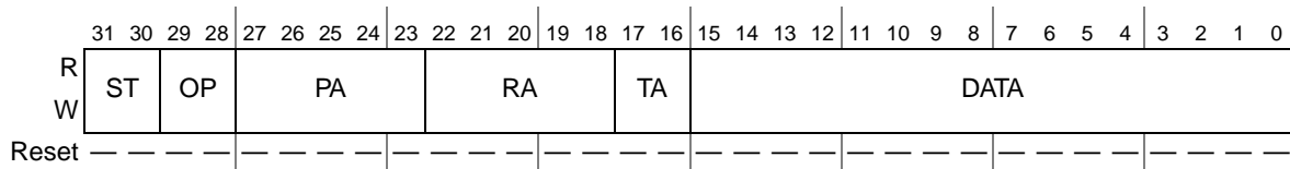
Figure 17-7. MII Management Frame Register (MMFR)
