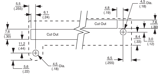
RIGHT ANGLE VERTICAL PRINTED CIRCUIT BOARD LAYOUT
