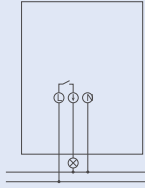
Switching diagram
