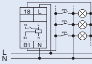
e.g. 3 wire circuit TLE
