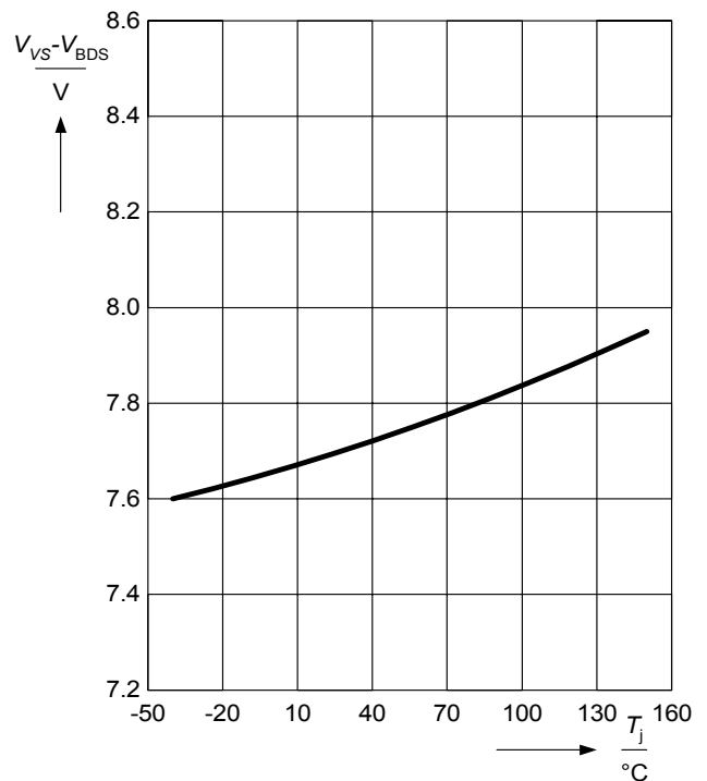
Gate driver supply V_{VS} - V_{BDS} vs. temperature T_i
