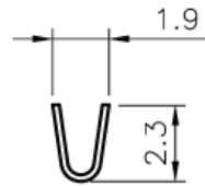
B-B SEC
