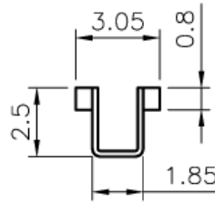
C-C SEC
