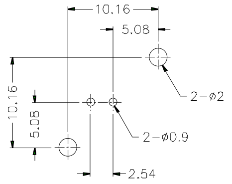
PCB MOUNTING HOLES
