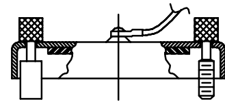
Sym. F Turnable Male and Female Jackscrews
