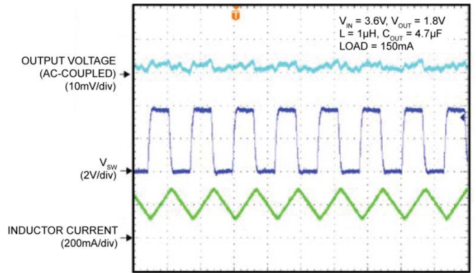
Switching Waveform Continuous Mode – 150mA
