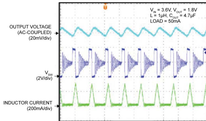
Switching Waveform Discontinuous Mode – 50mA
