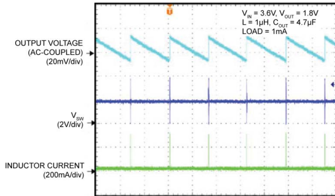
Switching Waveform Discontinuous Mode – 1mA
