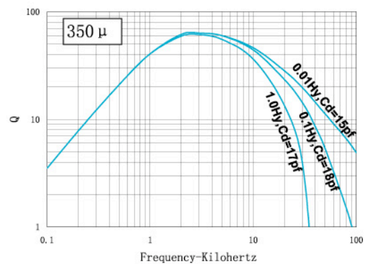
Typical Molypermalloy Q vs. frequency curves at indicated inductance and distributed capacitance.
