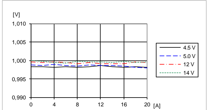
Load regulation at V_O = 1.0\text{ V} , T_{P1} = +25\text{ }^\circ\text{C} , C_O = 470\text{ }\mu\text{F}/10\text{ m}\Omega
