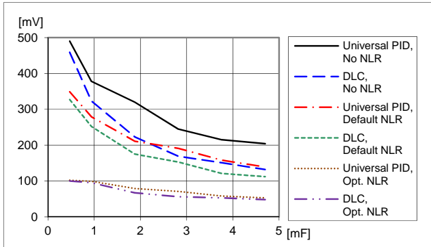
Load transient peak voltage deviation vs. external capacitance. Step (12.5-37.5-12.5 A). Parallel coupling of capacitors with 470 \mu F /10 m \Omega , T_{P1} = +25^\circ C , V_I = 12 V , V_O = 3.3 V , f_{sw} = 320 kHz , di/dt = 2 A/\mu s
