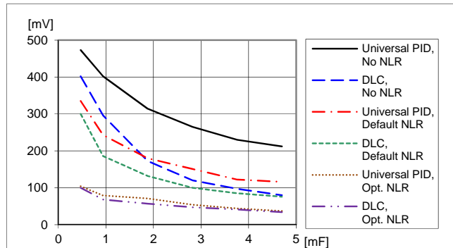
Load transient peak voltage deviation vs. external capacitance. Step (12.5-37.5-12.5 A). Parallel coupling of capacitors with 470 \mu F/10 m \Omega , T_{P1} = +25 °C. V_I = 12 V, V_O = 1.0 V, f_{sw} = 320 kHz, di/dt = 2 A/ \mu s
