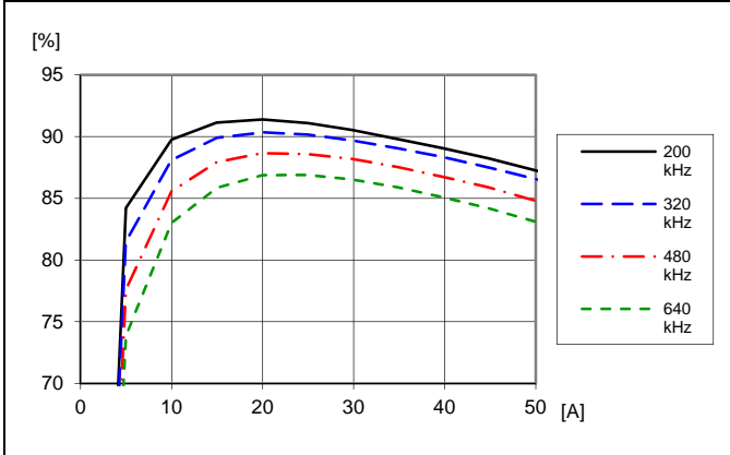
Efficiency vs. load current and switching frequency at T_{P1} = +25\text{ }^{\circ}\text{C} , V_I = 12\text{ V} , V_O = 1.0\text{ V} , C_O = 470\text{ }\mu\text{F}/10\text{ m}\Omega . Default configuration except changed frequency
