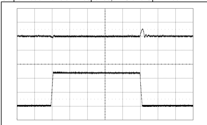
Output voltage response to load current step-change (12.5-37.5-12.5 A) at: T_{P1} = +25\text{ }^\circ\text{C} , V_I = 12\text{ V} , V_O = 1.0\text{ V} di/dt = 2\text{ A}/\mu\text{s} , f_{sw} = 320\text{ kHz} , C_O = 470\text{ }\mu\text{F}/10\text{ m}\Omega DLC and optimized NLR Top trace: output voltage (200 mV/div.). Bottom trace: load current (10 A/div.). Time scale: (0.1 ms/div.).
