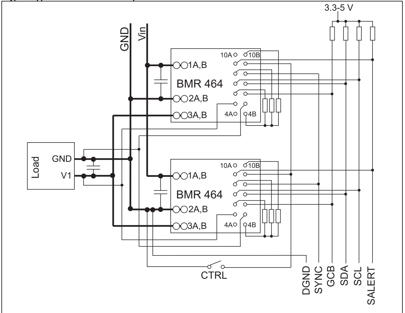
Parallel operation.
