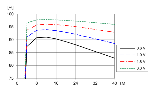
Efficiency vs. load current and output voltage: T_{P1} = +25^\circ\text{C} , V_I = 5\text{ V} , f_{sw} = 320\text{ kHz} , C_O = 470\text{ }\mu\text{F}/10\text{ m}\Omega .
