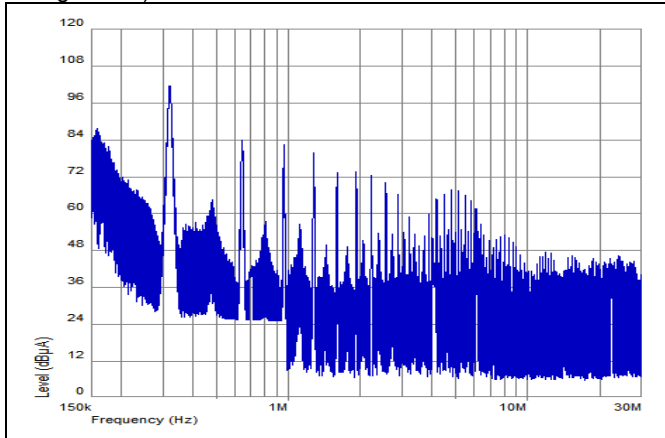
EMI without filter for BMR 464 2008
