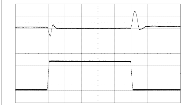
Output voltage response to load current Step-change (12.5-37.5-12.5 A) at: T_{P1} = +25^\circ C , V_I = 12 V , V_O = 1.0 V di/dt = 2 A/\mu s , f_{sw} = 320 kHz C_O = 470 \mu F /10 m \Omega
