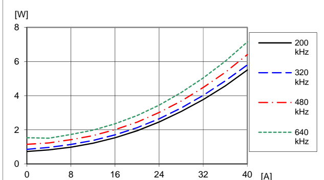
Dissipated power vs. load current and switch frequency at T_{P1} = +25^\circ\text{C} , V_I = 12\text{ V} , V_O = 1.0\text{ V} , C_O = 470\text{ }\mu\text{F}/10\text{ m}\Omega Default configuration except changed frequency
