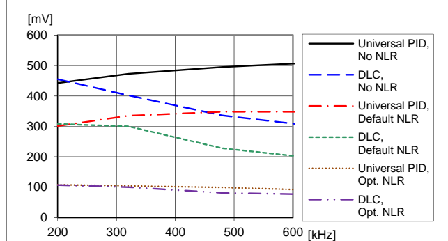
Load transient peak voltage deviation vs. frequency. Step-change (12.5-37.5-12.5 A). T_{P1} = +25 °C. V_I = 12 V, V_O = 1.0 V, C_O = 470 \mu F/10 m \Omega
