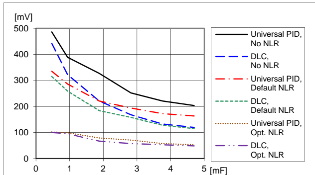
Load transient peak voltage deviation vs. external capacitance. Step (12.5-37.5-12.5 A). Parallel coupling of capacitors with 470 \mu F/10 m \Omega , T_{P1} = +25 °C. V_I = 12 V, V_O = 3.3 V, f_{sw} = 320 kHz, di/dt = 2 A/ \mu s
