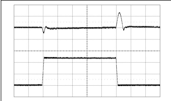
Output voltage response to load current step-change (12.5-37.5-12.5 A) at: T_{P1} = +25\text{ }^\circ\text{C} , V_I = 12\text{ V} , V_O = 1.0\text{ V} di/dt = 2\text{ A}/\mu\text{s} , f_{sw} = 320\text{ kHz} , C_O = 470\text{ }\mu\text{F}/10\text{ m}\Omega Default configuration (DLC and default NLR) Top trace: output voltage (200 mV/div.). Bottom trace: load current (10 A/div.). Time scale: (0.1 ms/div.).
