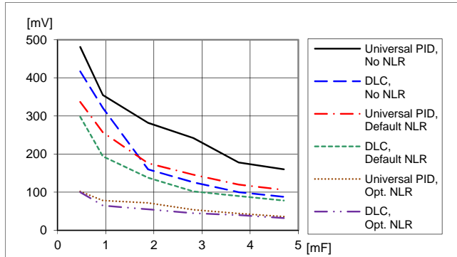
Load transient peak voltage deviation vs. external capacitance. Step (12.5-37.5-12.5 A). Parallel coupling of capacitors with 470 \mu F /10 m \Omega , T_{P1} = +25^\circ C , V_I = 12 V , V_O = 1.0 V , f_{sw} = 320 kHz , di/dt = 2 A/\mu s
