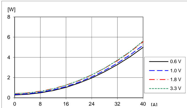
Dissipated power vs. load current and output voltage: T_{P1} = +25^\circ\text{C} , V_I = 5\text{ V} , f_{sw} = 320\text{ kHz} , C_O = 470\text{ }\mu\text{F}/10\text{ m}\Omega .
