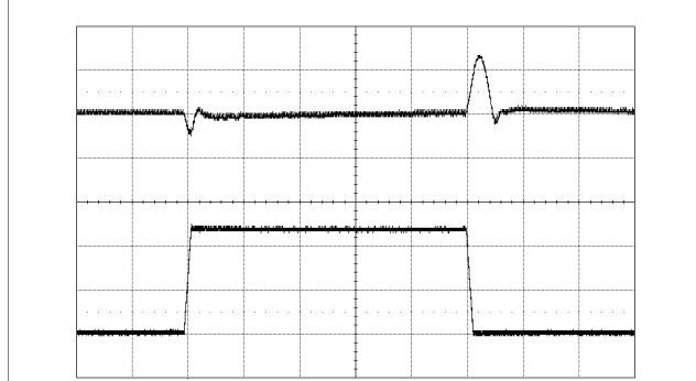
Output voltage response to load Step-change (12.5-37.5-12.5 A) at: T_{P1} = +25 °C, V_I = 12 V, V_O = 1.0 V di/dt = 2 A/ \mu s, f_{sw} = 320 kHz C_O = 470 \mu F/10 m \Omega Top trace: output voltage (200 mV/div.). Bottom trace: load current (10 A/div.). Time scale: (0.1 ms/div.).
