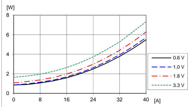
Dissipated power vs. load current and output voltage: T_{P1} = +25^\circ\text{C} , V_I = 12\text{ V} , f_{sw} = 320\text{ kHz} , C_O = 470\text{ }\mu\text{F}/10\text{ m}\Omega .
