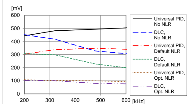
Load transient peak voltage deviation vs. frequency. Step-change (12.5-37.5-12.5 A). T_{P1} = +25^\circ C , V_I = 12 V , V_O = 1.0 V , C_O = 470 \mu F /10 m \Omega
