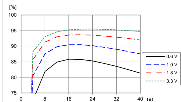
Efficiency vs. load current and output voltage at T_{P1} = +25^\circ\text{C} , V_I = 12\text{ V} , f_{sw} = 320\text{ kHz} , C_O = 470\text{ }\mu\text{F}/10\text{ m}\Omega .
