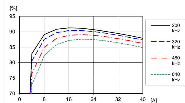
Efficiency vs. load current and switch frequency at T_{P1} = +25^\circ\text{C} , V_I = 12\text{ V} , V_O = 1.0\text{ V} , C_O = 470\text{ }\mu\text{F}/10\text{ m}\Omega Default configuration except changed frequency
