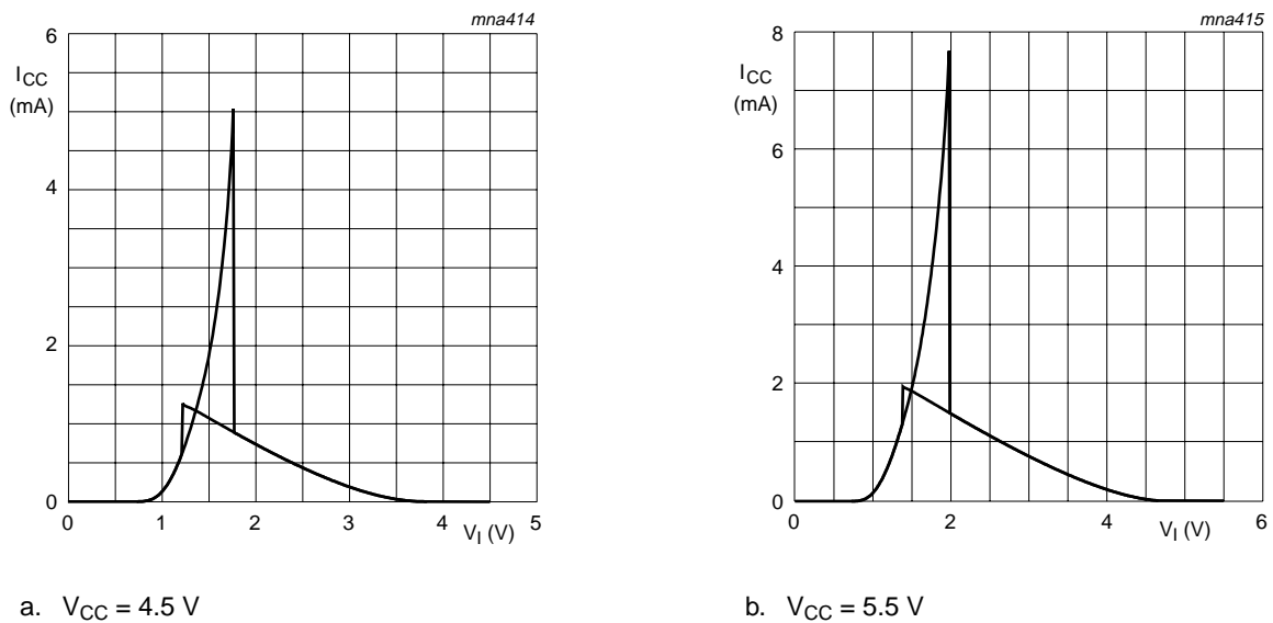
Fig 11. Typical 74VHCT transfer characteristics
