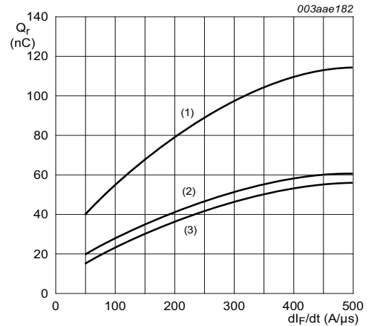
Fig. 5. Recovered charge as a function of rate of change of forward current; T_j = 125\text{ °C} ; typical values
