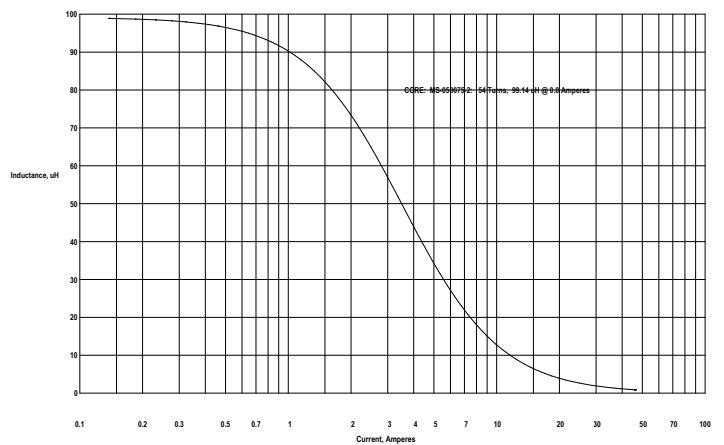
CREATED IN MICROMETALS ARNOLD POWDER CORES - DESIGN OF INDUCTORS FOR POWER FILTER APPLICATIONS Fri Nov 18 08:17:09 2011
