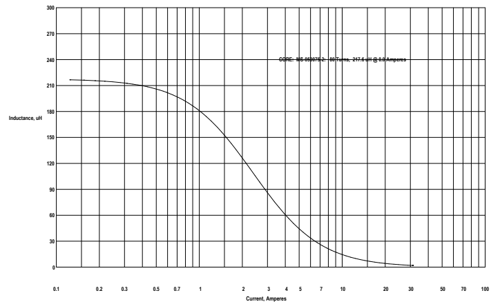
CREATED IN MICROMETALS ARNOLD POWDER CORES - DESIGN OF INDUCTORS FOR POWER FILTER APPLICATIONS Tue Nov 08 11:22:53 2011
