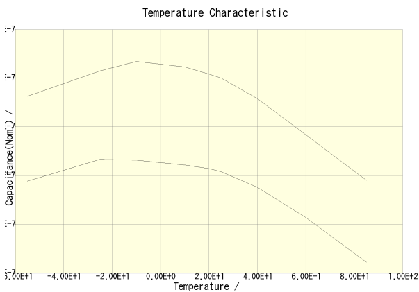
C0816X5R1A224M050AC(DC Bias = 0V) C0816X5R1A224M050AC(DC Bias = 5V)
