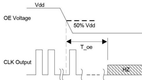
Figure 12: OE Disable Timing (OE Mode Only)
