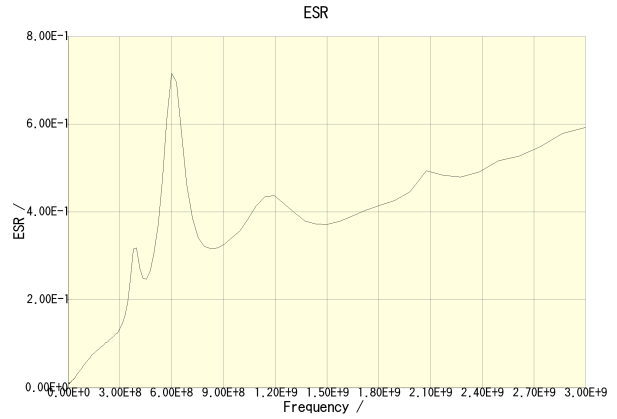
C2012C0G2E152J085AA
