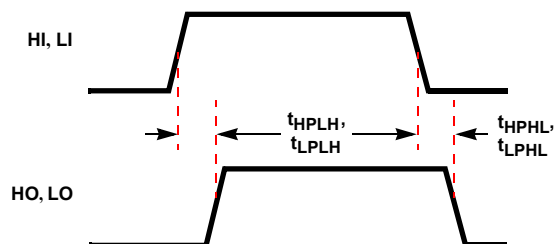
FIGURE 5. PROPAGATION DELAYS
