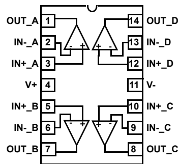
ISL28433 (14 LD TDFN) TOP VIEW
