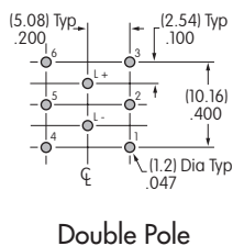
Double Pole
