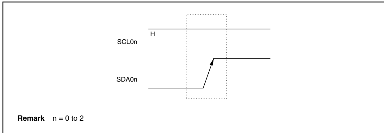
Figure 17-9. Stop Condition
