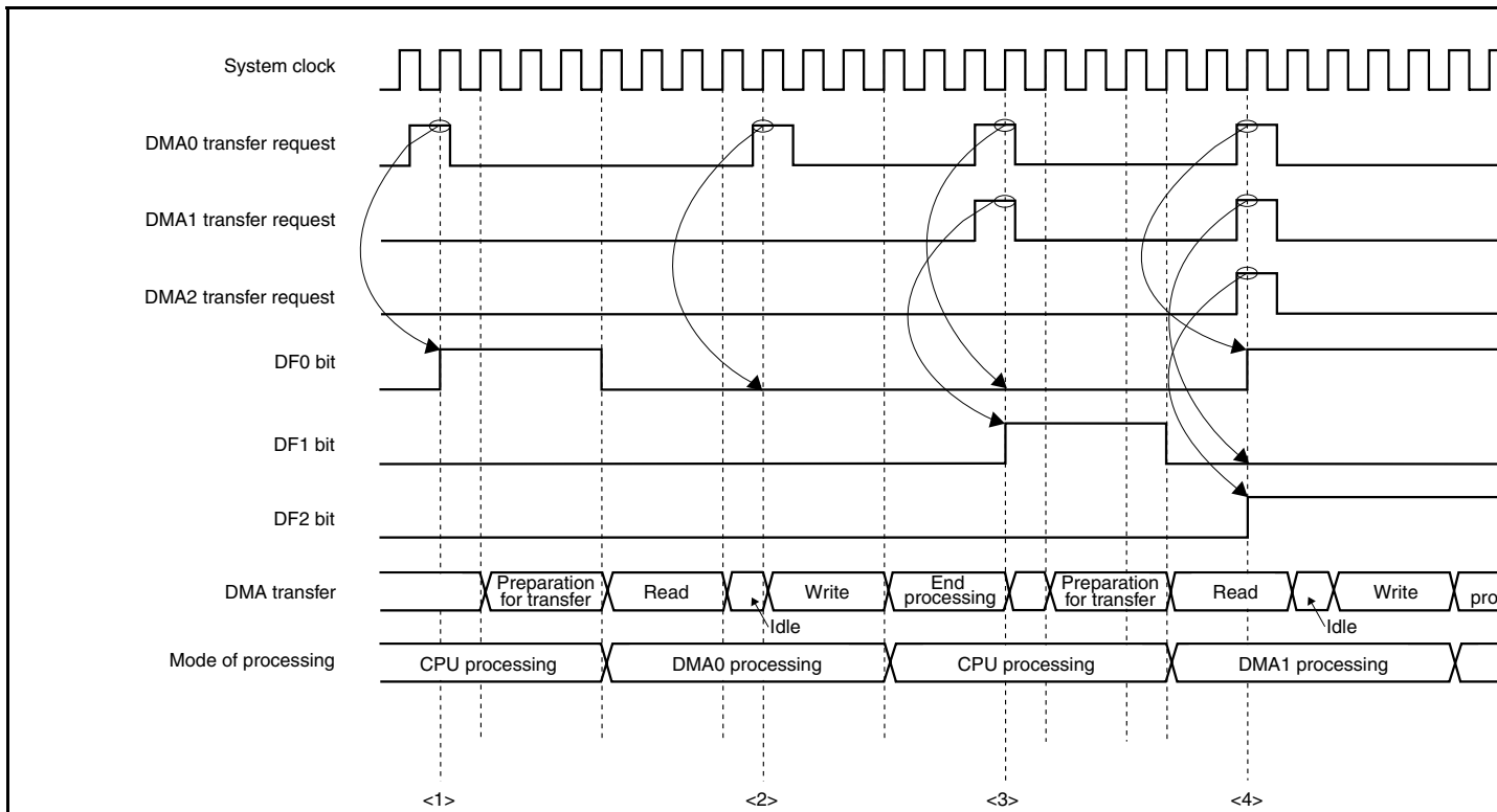
Figure 20-5. Period in Which DMA Transfer Request Is Ignored (2)
