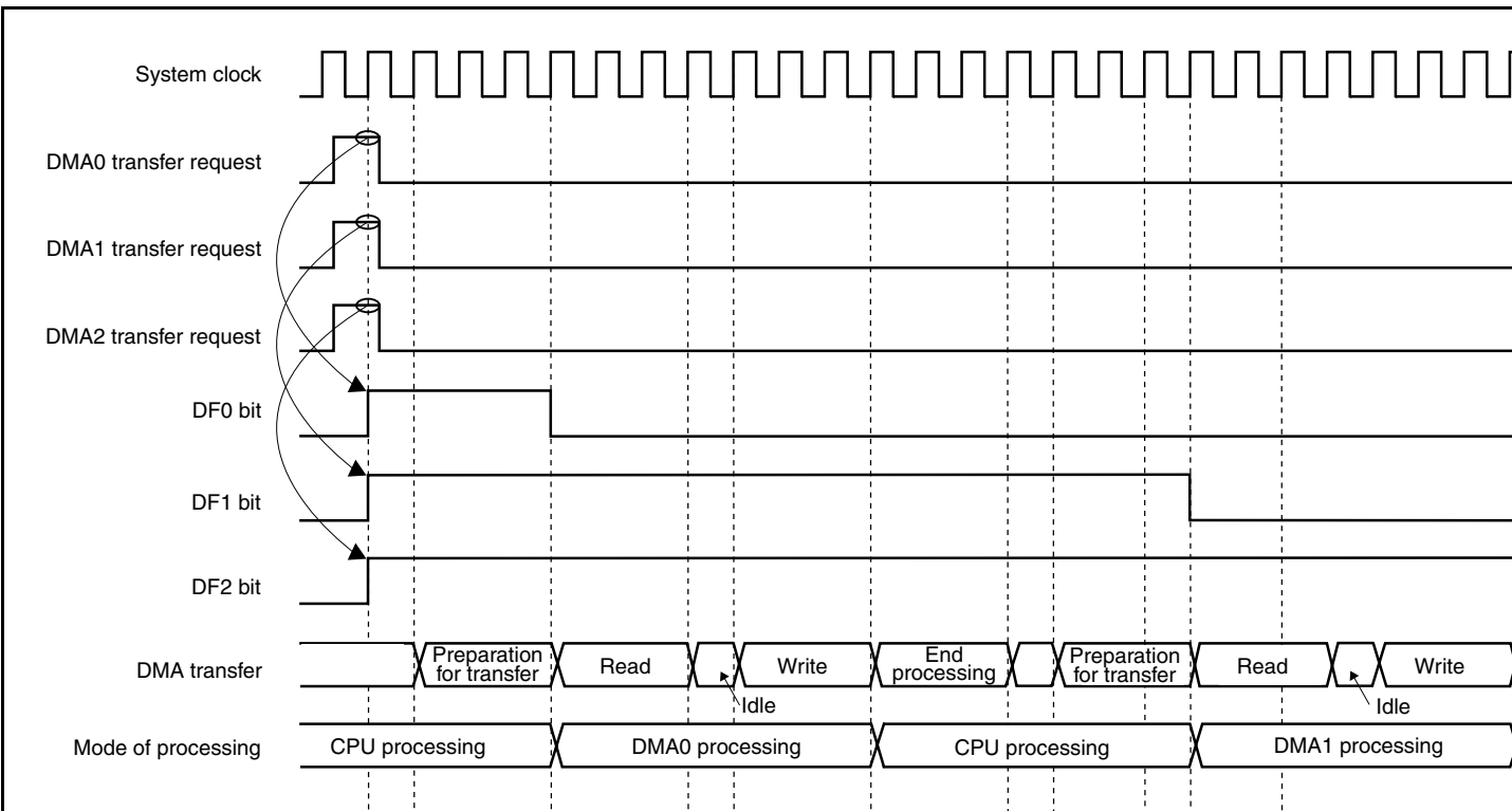
Figure 20-2. Priority of DMA (1)
