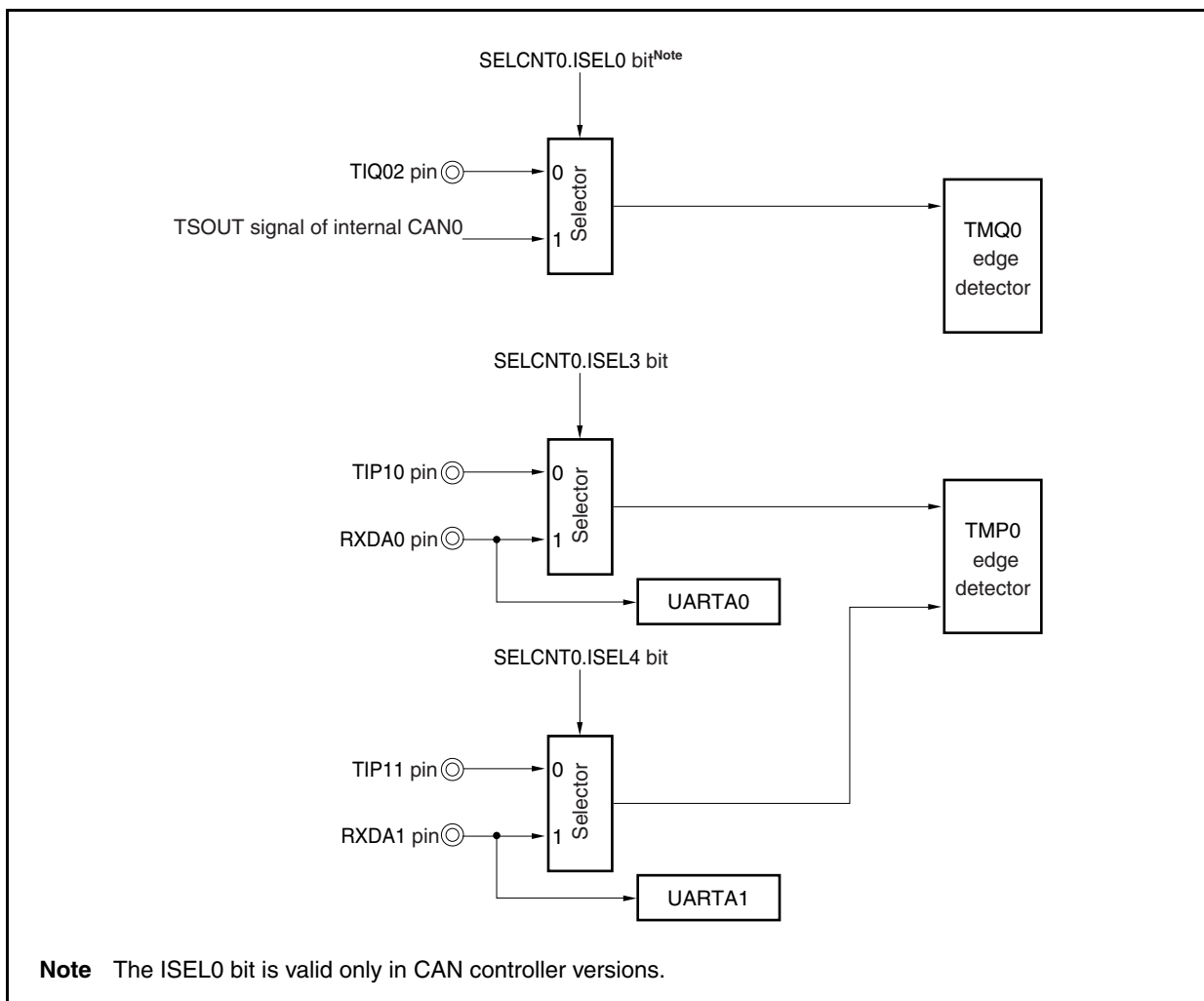
Figure 7-42. Block Diagram of Selector Function
