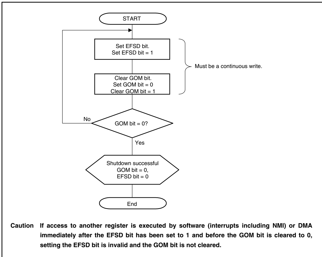
Figure 19-57. Forced Shutdown Process
