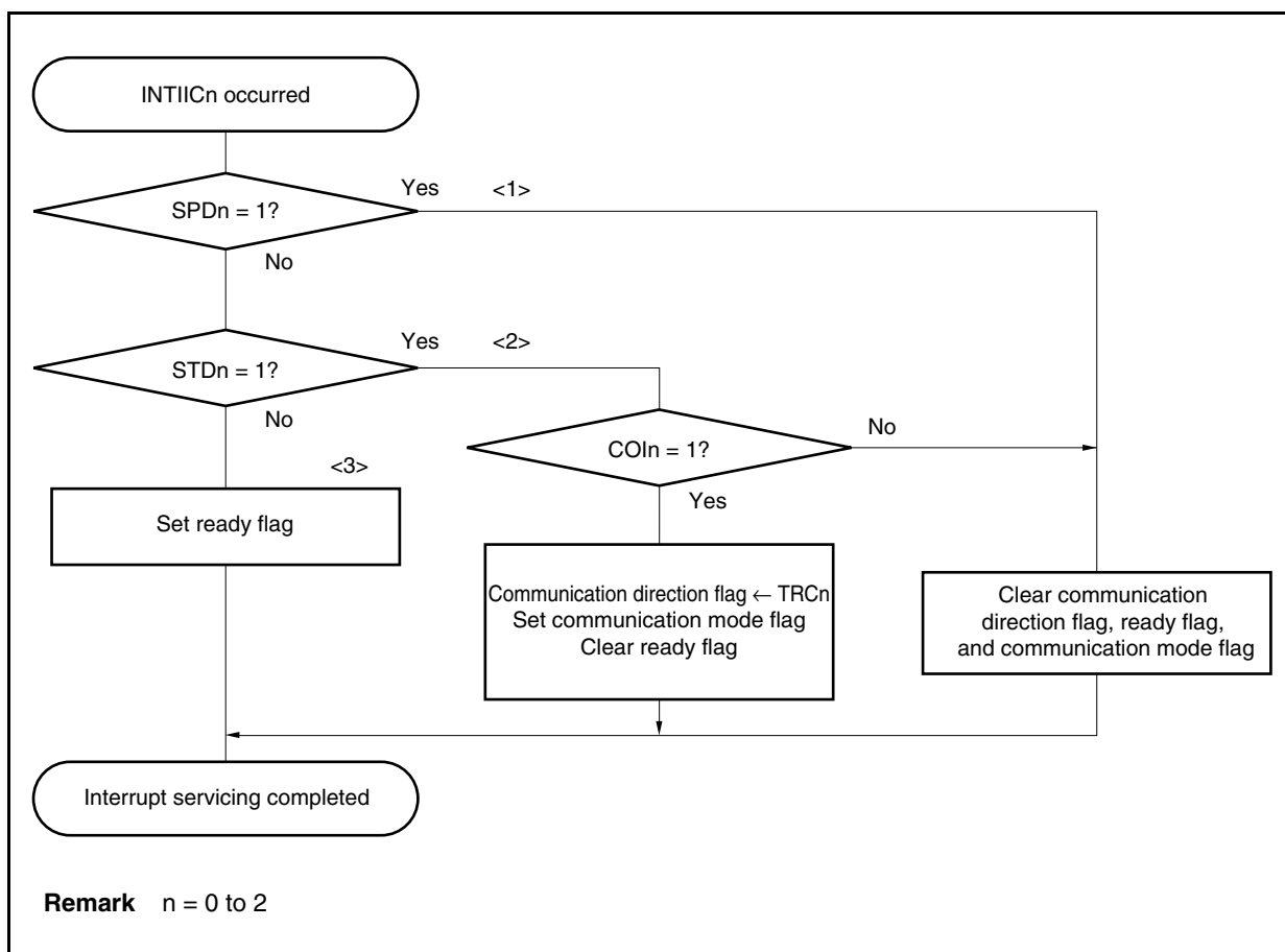
Figure 17-19. Slave Operation Flowchart (2)
