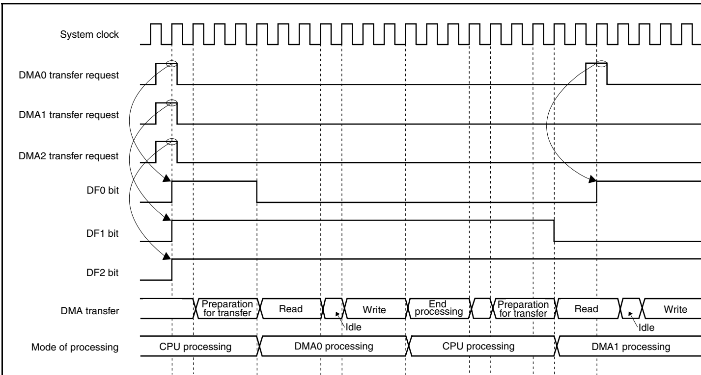
Figure 20-3. Priority of DMA (2)
