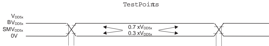
Figure 7-1: AC Test Input/Output Waveform
