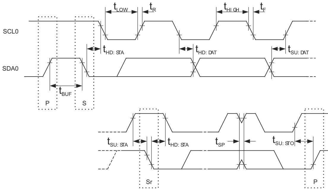
Figure 7-8: I 2 C Timing
