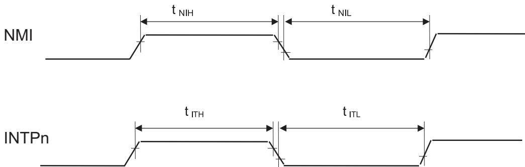
Figure 7-4: Interrupt Timing
