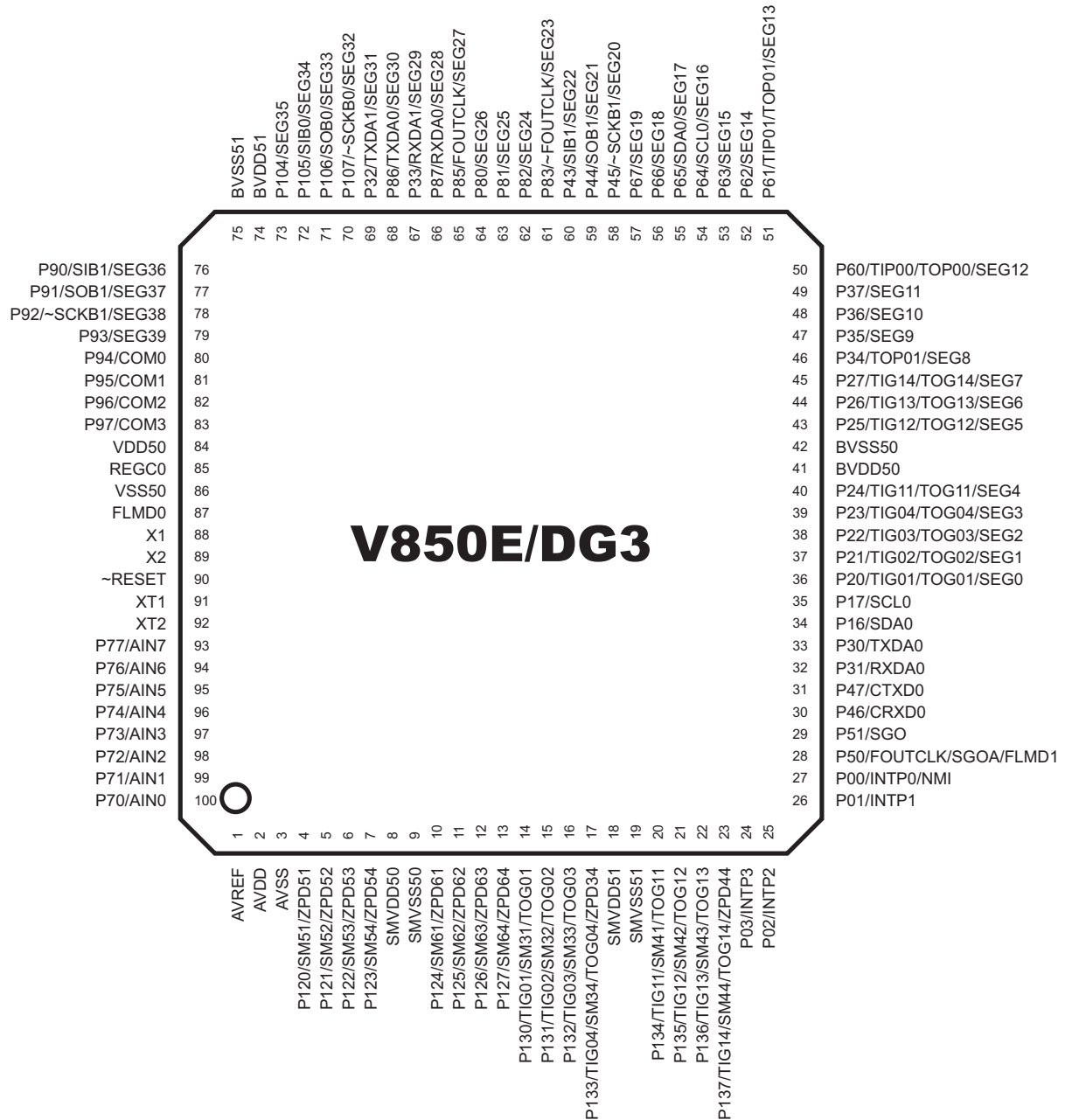
Figure 2-1: Pin Configuration \mu PD70F3417(A), \mu PD70F3416(A)
