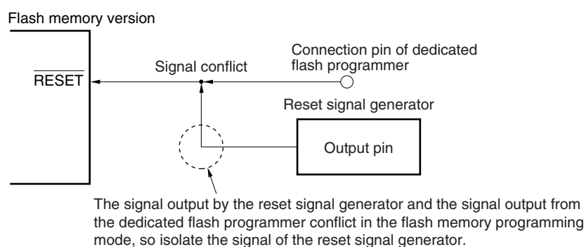
Figure 23-8. Signal Conflict ( \overline{\text{RESET}} Pin)
