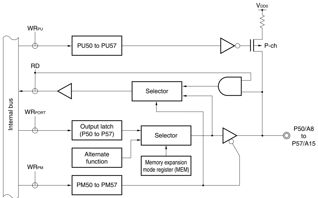
Figure 6-18. Block Diagram of P50 to P57
