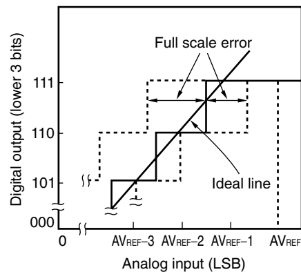
Figure 14-12. Full Scale Error
