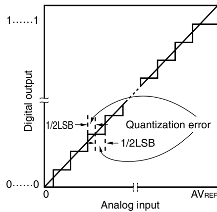
Figure 14-10. Quantization Error
