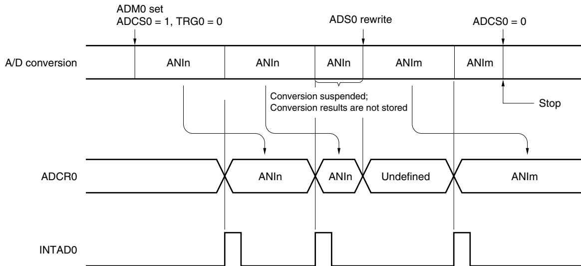
Figure 13-7. A/D Conversion by Software Start
