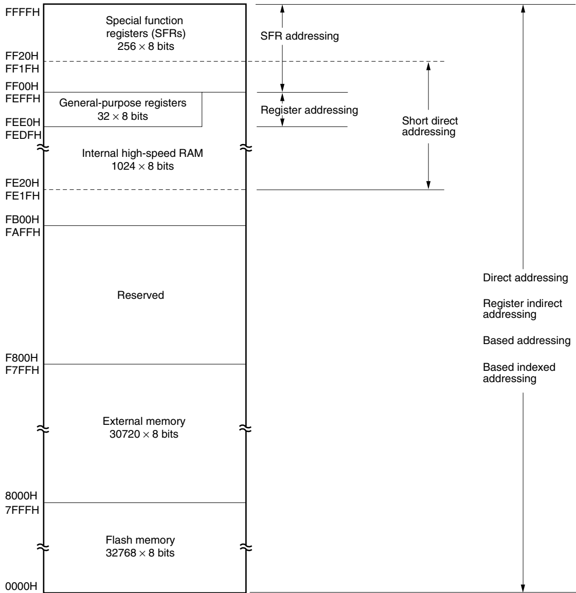
Figure 5-10. Correspondence Between Data Memory and Addressing ( \mu PD78F0034A, 78F0034B, 78F0034AY, 78F0034BY)
