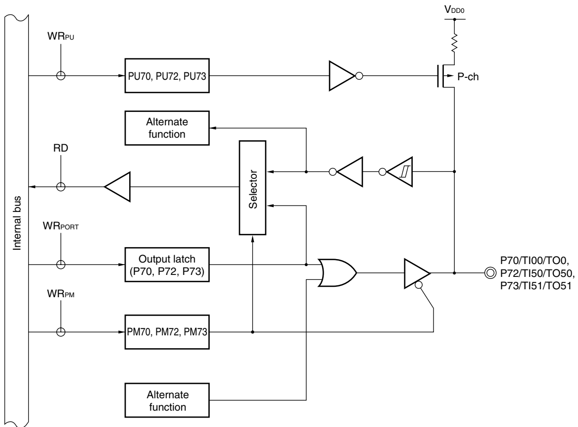
Figure 6-21. Block Diagram of P70, P72, and P73
