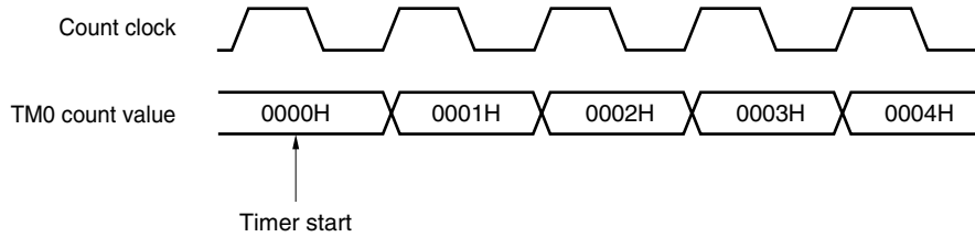
Figure 8-28. Start Timing of 16-Bit Timer Counter 0 (TM0)
