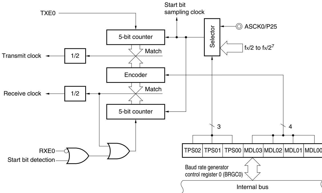
Figure 16-2. Block Diagram of Baud Rate Generator
