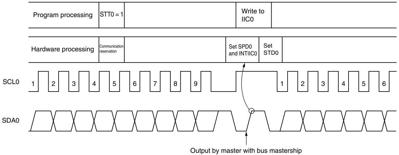
Figure 18-18. Communication Reservation Timing
