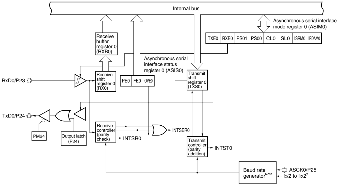
Figure 16-1. Block Diagram of Serial Interface UART0
