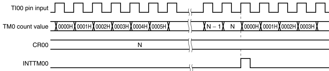
Figure 8-13. External Event Counter Operation Timing (with Rising Edge Specified)
