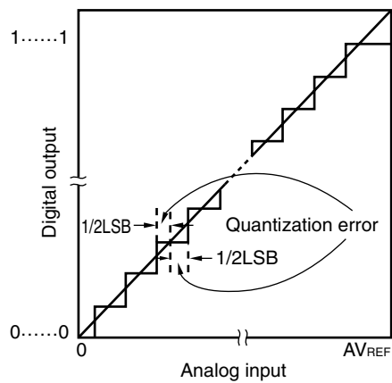
Figure 13-9. Quantization Error
