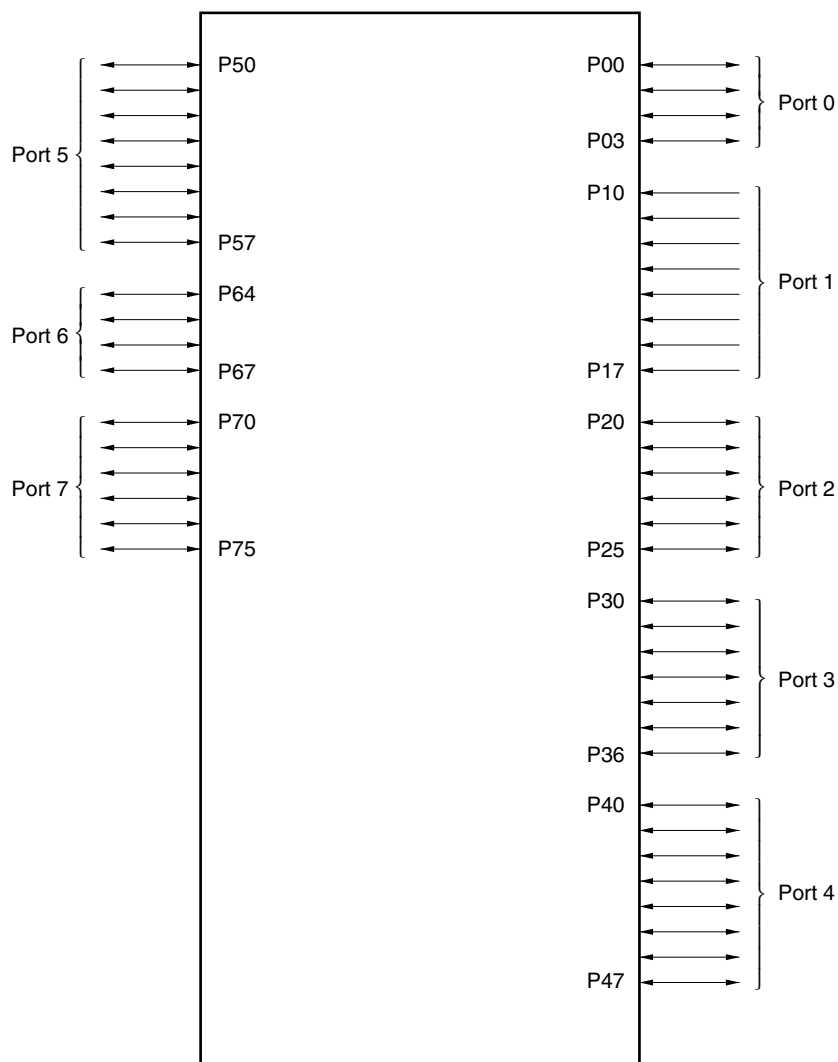
Figure 6-1. Port Types
