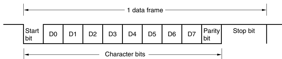
Figure 16-8. Example of Transmit/Receive Data Format in Asynchronous Serial Interface
