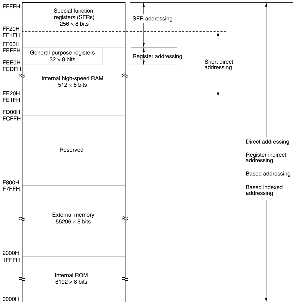
Figure 5-6. Correspondence Between Data Memory and Addressing ( \mu PD780021A, 780031A, 780021AY, 780031AY)
