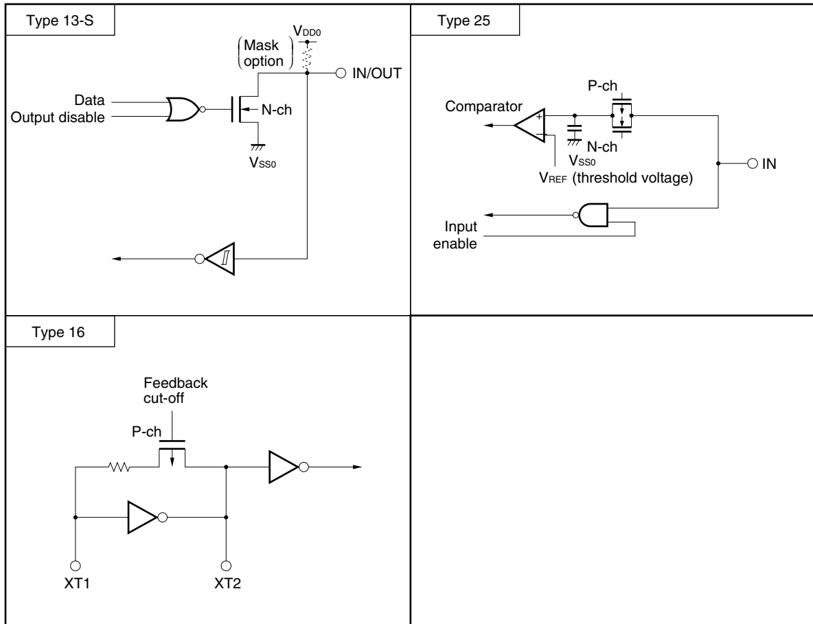
Figure 3-1. Pin I/O Circuit List (2/2)
