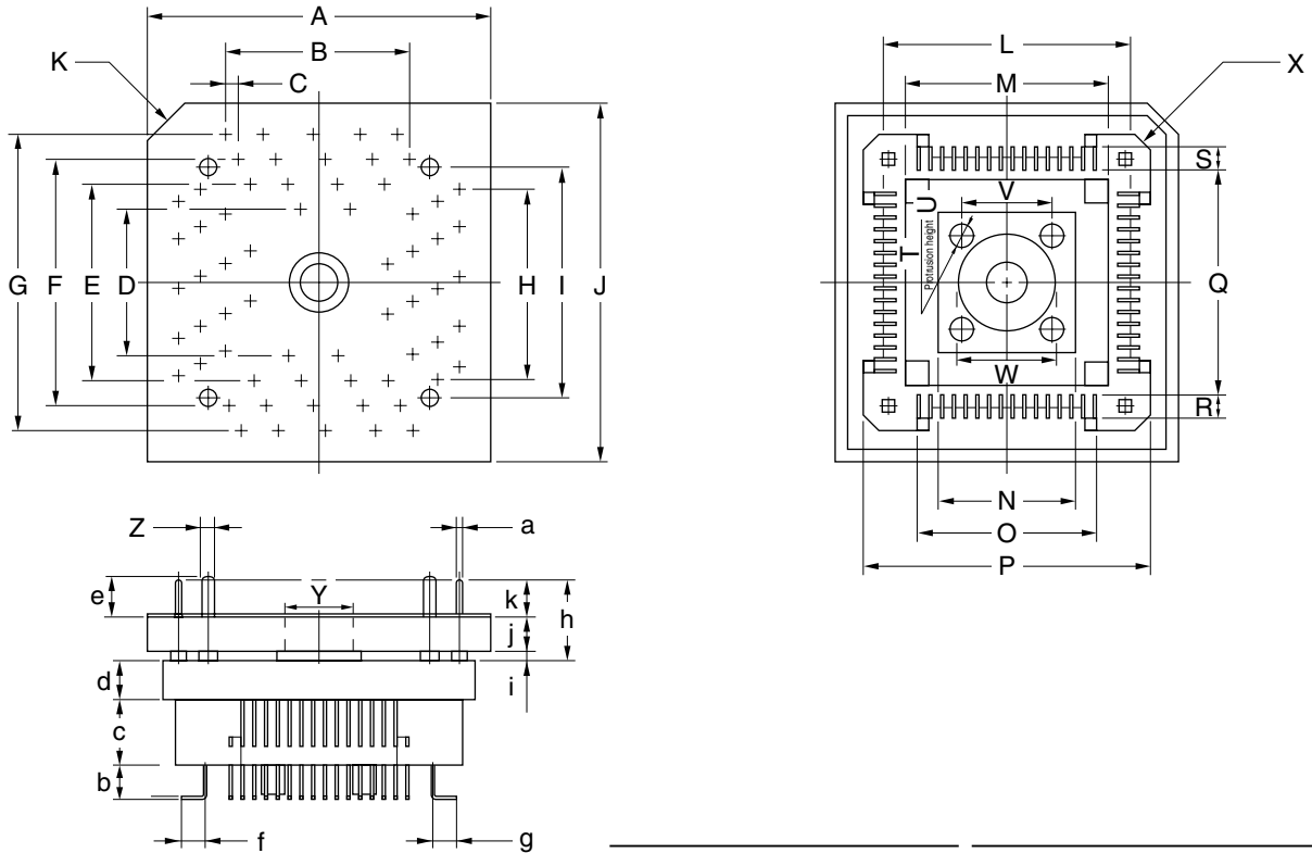
Figure B-5. TKG-064SBW Package Drawing (for Reference Only)
