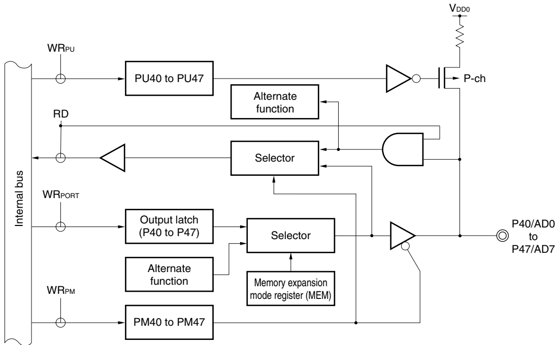
Figure 6-16. Block Diagram of P40 to P47
