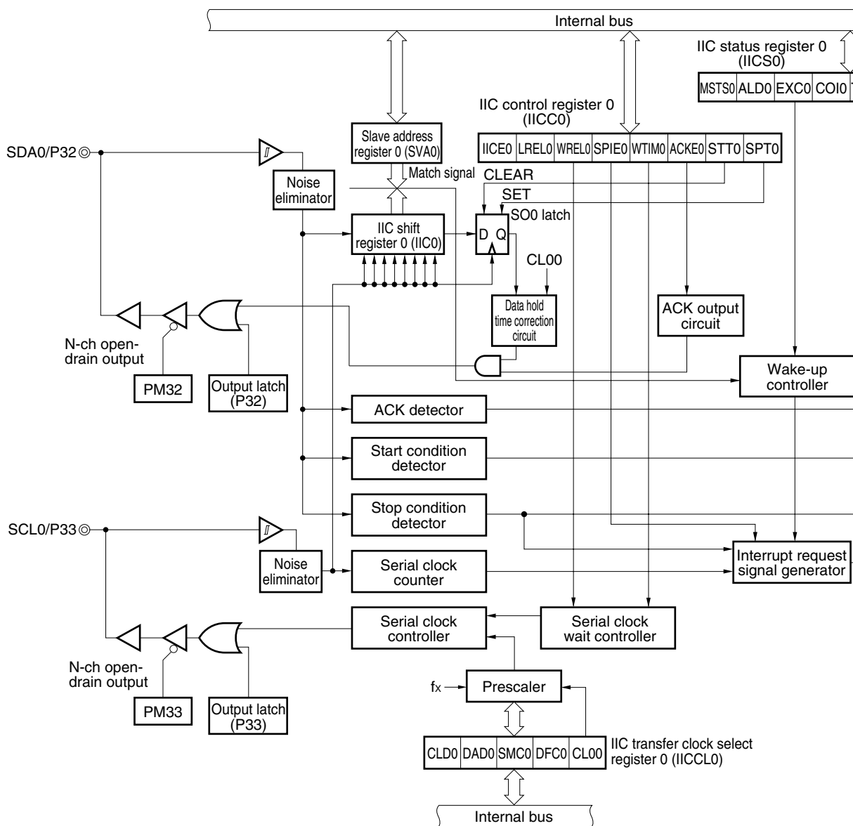
Figure 18-1. Block Diagram of Serial Interface IIC0
