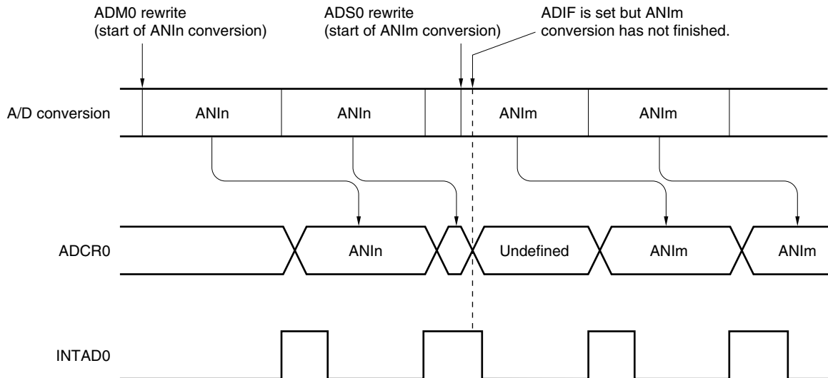
Figure 13-15. A/D Conversion End Interrupt Request Generation Timing
