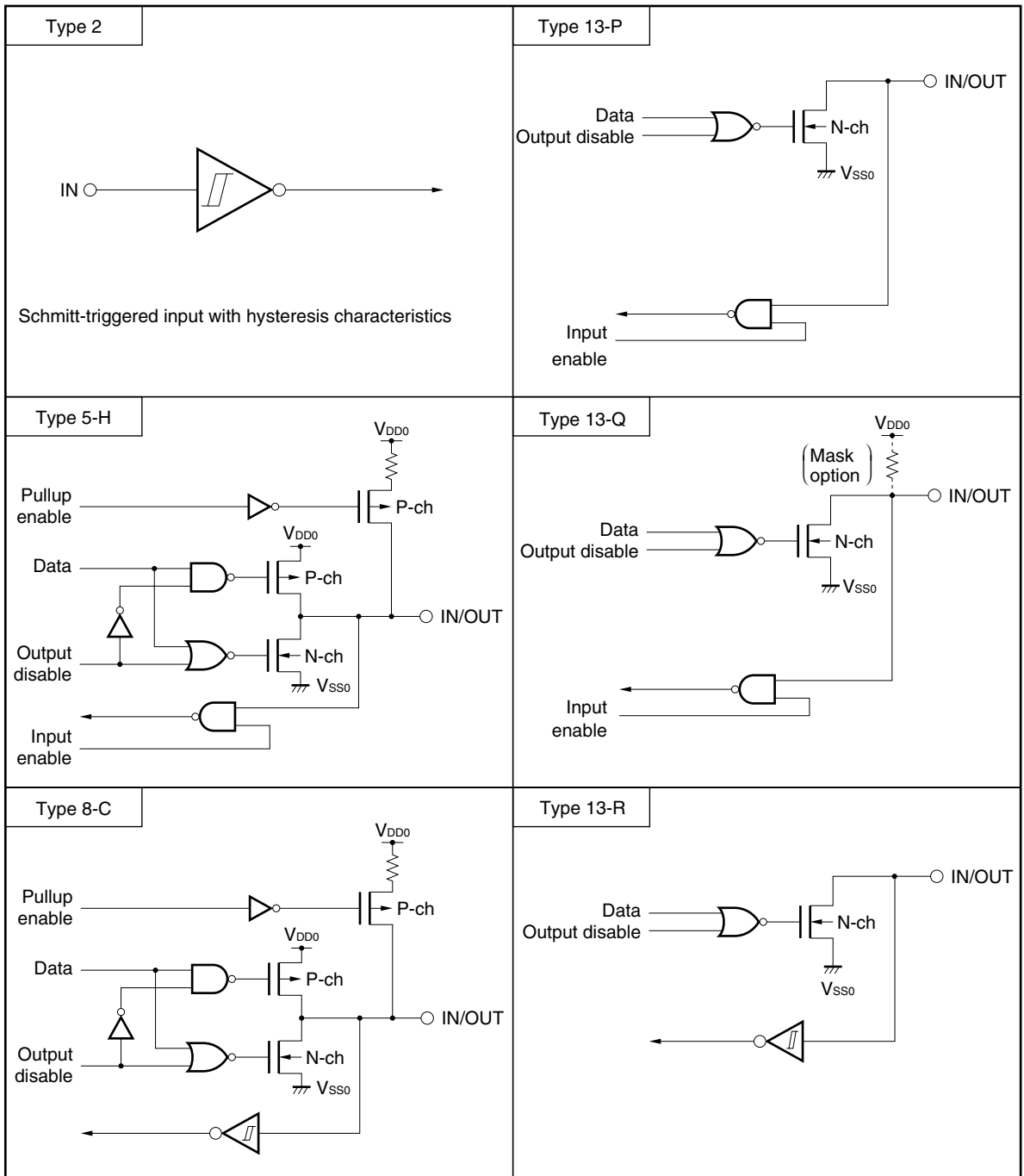
Figure 3-1. Pin I/O Circuit List (1/2)
