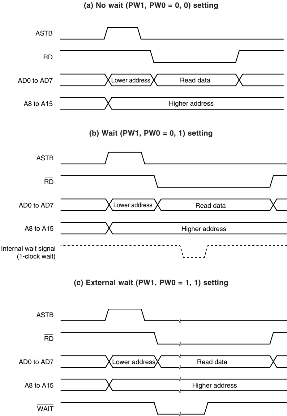
Figure 20-5. External Memory Read Timing
