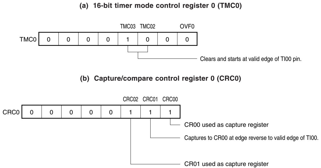
Figure 8-22. Timing of Pulse Width Measurement Operation by Means of Restart (with Rising Edge Specified)
