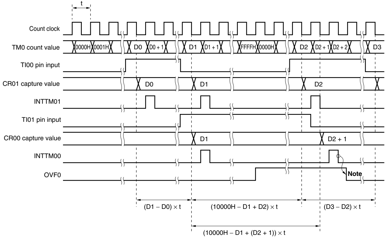
Figure 8-18. Timing of Pulse Width Measurement Operation with Free-Running Counter (with Both Edges Specified)
