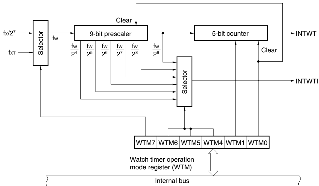
Figure 10-1. Watch Timer Block Diagram
