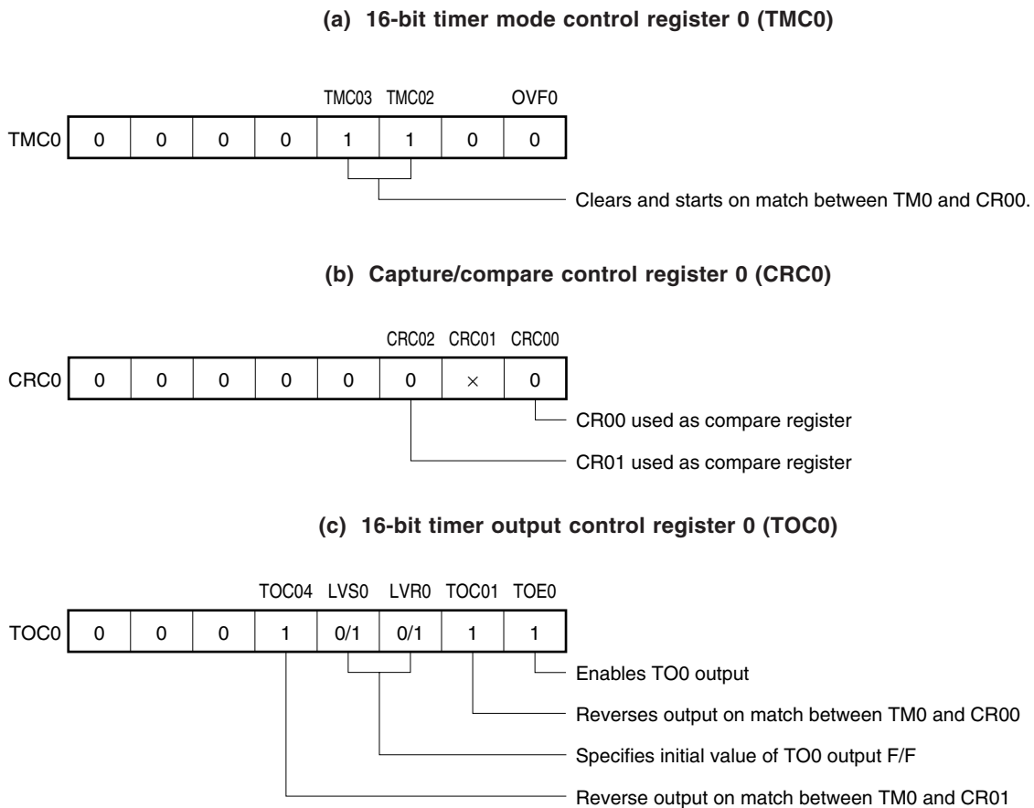
Figure 8-25. Control Register Settings for PPG Output Operation
