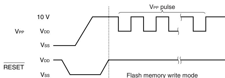
Figure 23-3. Communication Mode Selection Format
