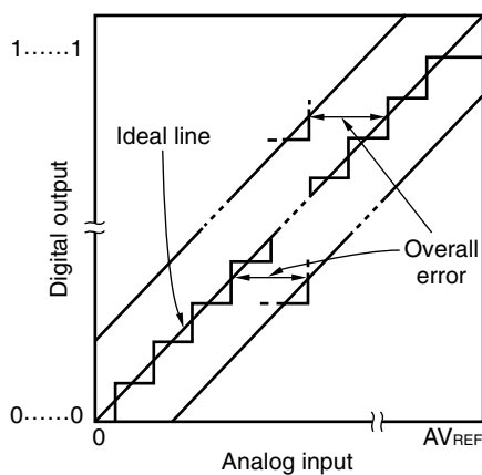
Figure 13-8. Overall Error
