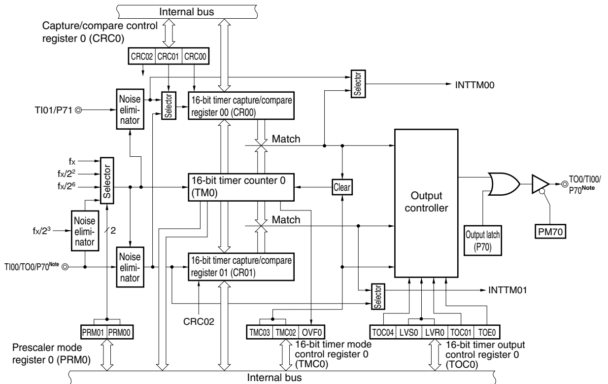
Figure 8-1. Block Diagram of 16-Bit Timer/Event Counter 0
