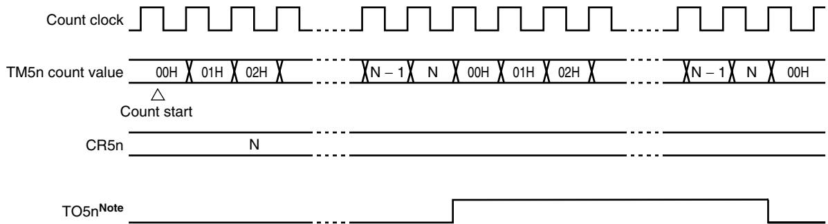
Figure 9-10. Square-Wave Output Operation Timing
