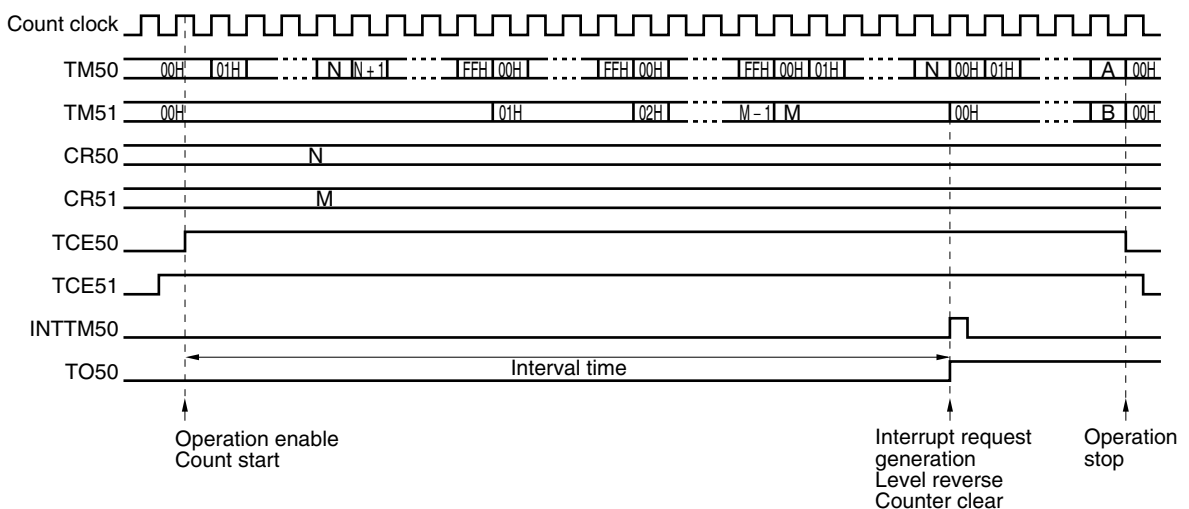
Figure 9-13. 16-Bit Resolution Cascade Connection Mode
