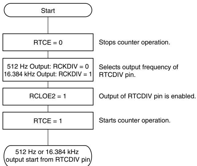
Figure 10-26. 512 Hz, 16.384 kHz output Setting Procedure
