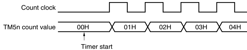
Figure 7-20. 8-Bit Timer Counter 5n (TM5n) Start Timing
