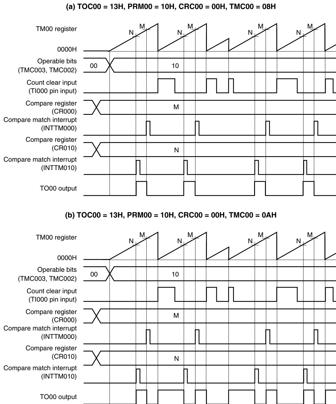
Figure 6-24. Timing Example of Clear & Start Mode Entered by TI000 Pin Valid Edge Input (CR000: Compare Register, CR010: Compare Register)
