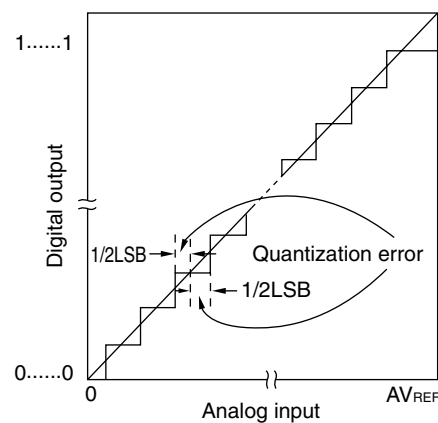
Figure 12-17. Quantization Error
