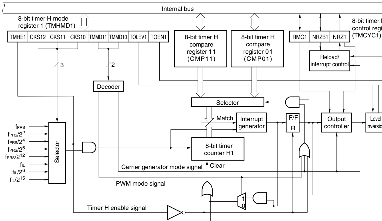
Figure 8-2. Block Diagram of 8-Bit Timer H1
