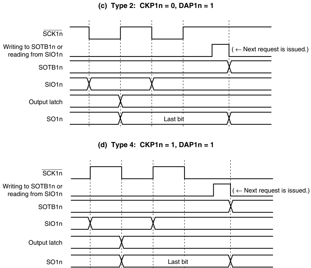
Figure 16-18. Output Value of SO1n Pin (Last Bit) (2/2)
