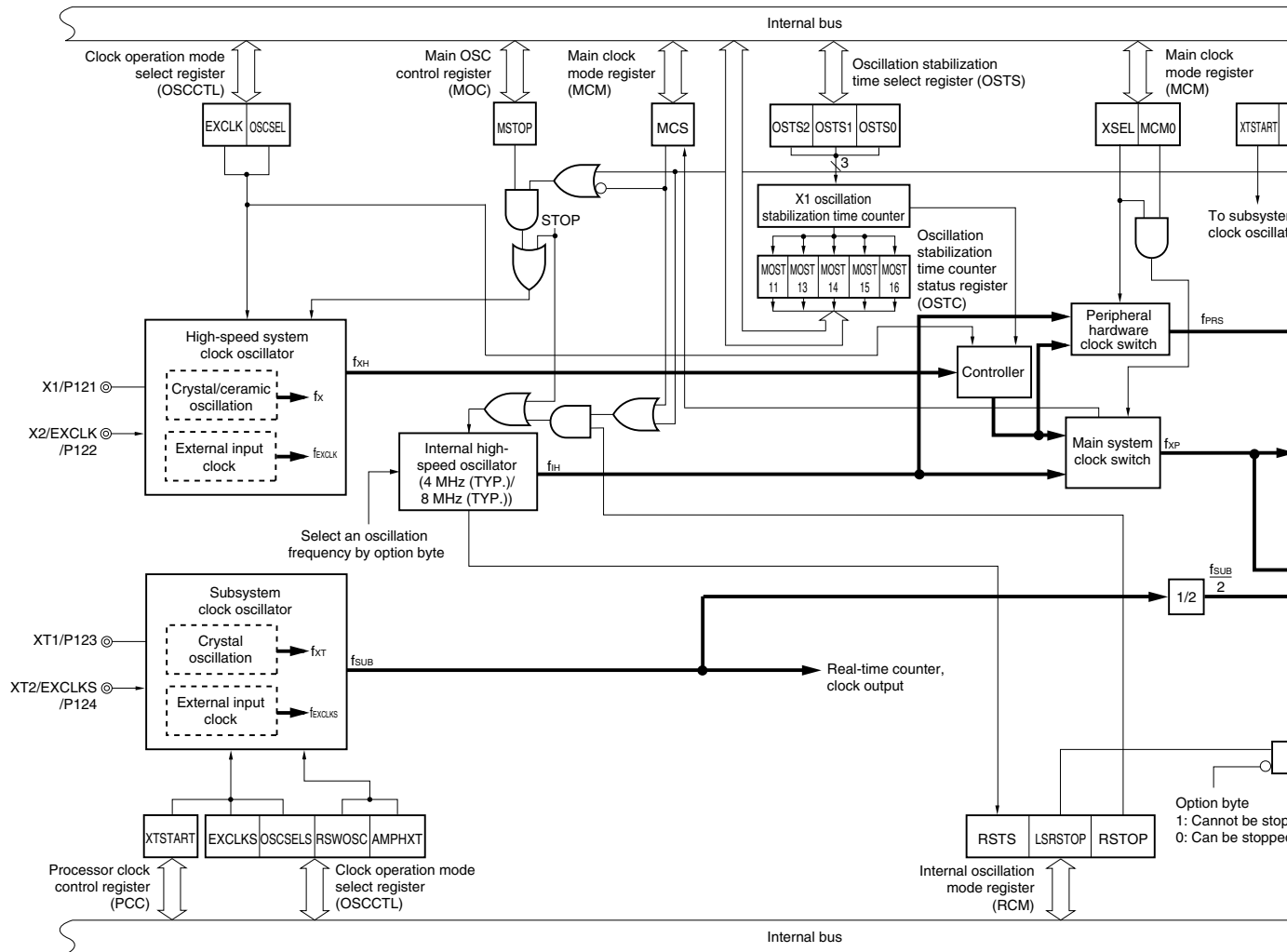
Figure 5-2. Block Diagram of Clock Generator (78K0/KC2-L)
