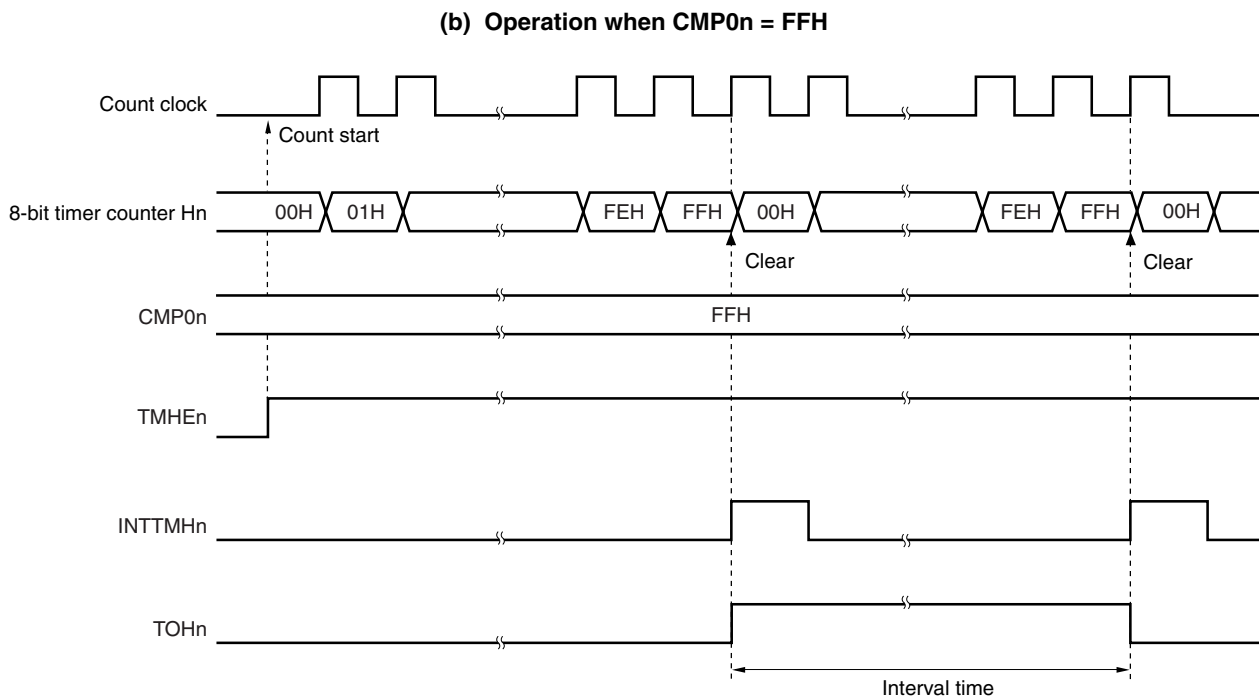
Figure 8-13. Timing of Interval Timer/Square-Wave Output Operation (2/2)
