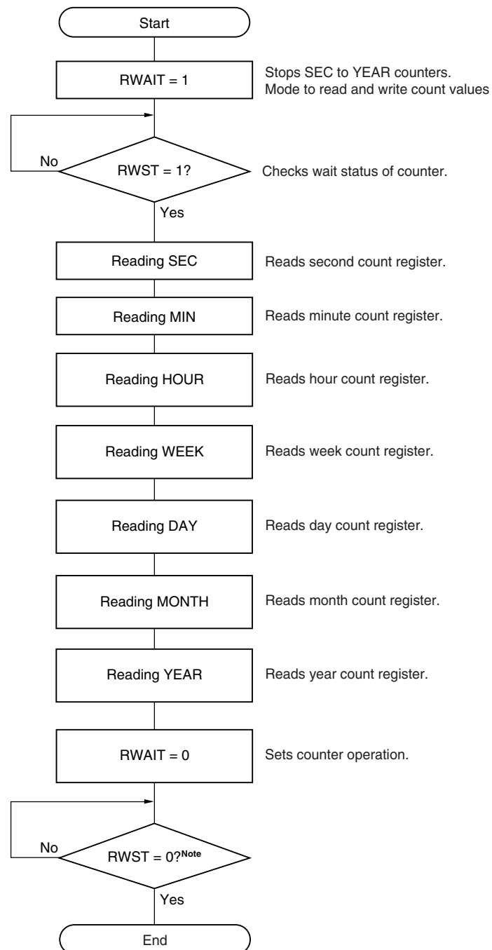
Figure 10-21. Procedure for Reading Real-Time Counter
