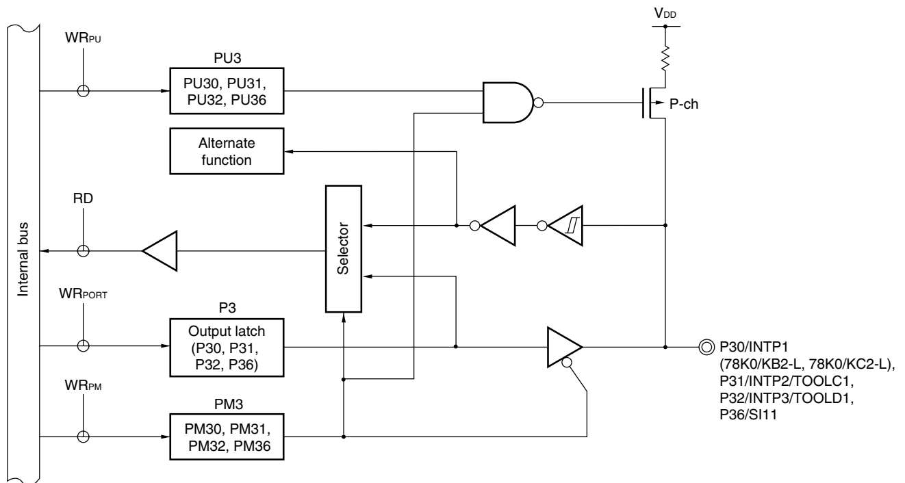
Figure 4-16. Block Diagram of P30 (78K0/KB2-L, 78K0/KC2-L), P31, P32, P36
