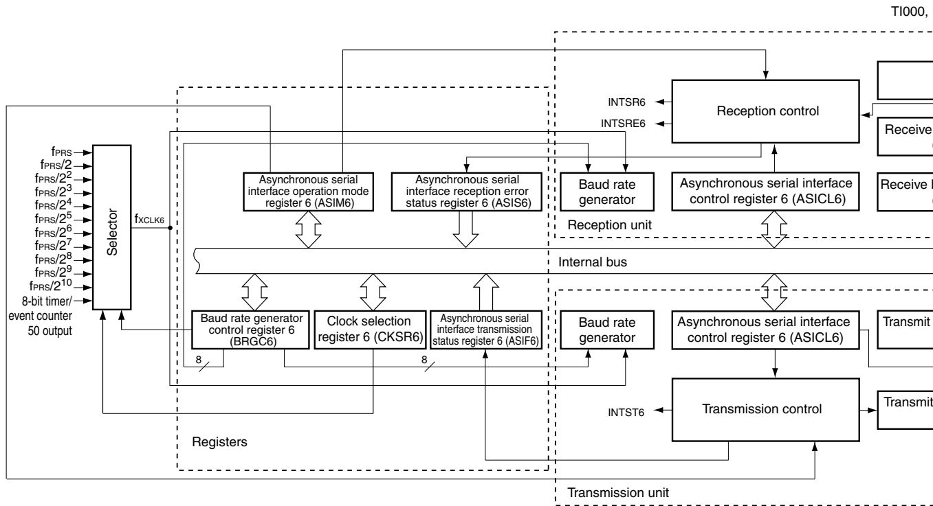
Figure 14-4. Block Diagram of Serial Interface UART6
