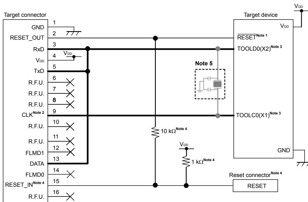
<R> Figure 26-1. Connection Example of QB-MINI2 and 78K0/lx2 Microcontrollers (2/3) (2) When using the TOOLC0 and TOOLD0 pins (with X1/X2 oscillator is used, both debugging and programming are performed)
