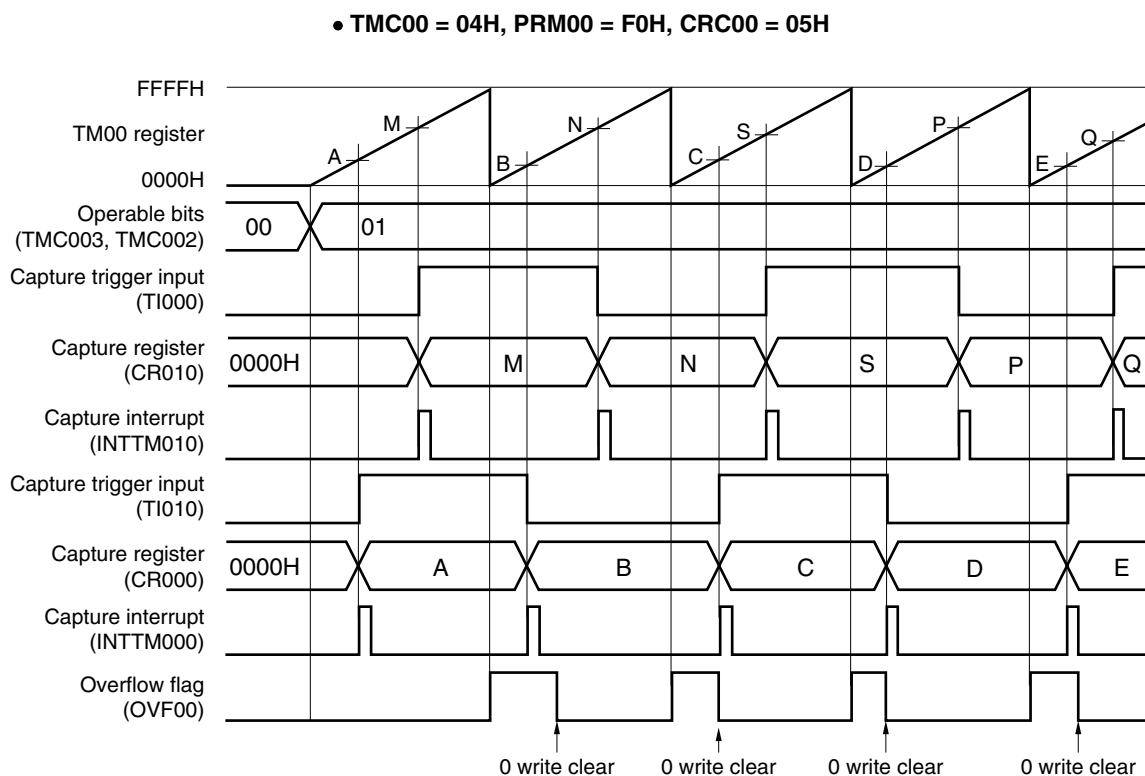
Figure 6-49. Timing Example of Pulse Width Measurement (1)
