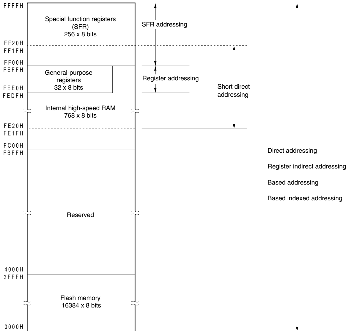
Figure 3-7. Correspondence Between Data Memory and Addressing ( \mu PD78F0552, 78F0557, 78F0562, 78F0567, 78F0572, 78F0577, 78F0582, 78F0587)
