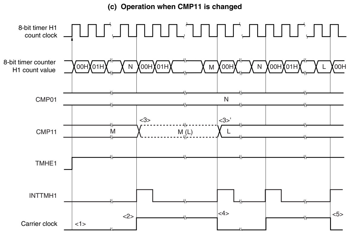
Figure 8-18. Carrier Generator Mode Operation Timing (3/3)
