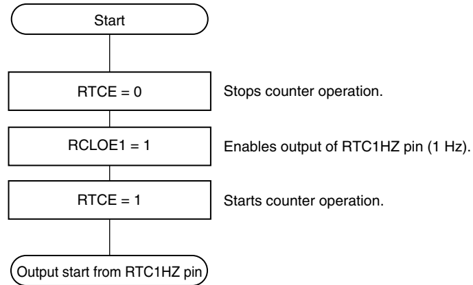
Figure 10-24. 1 Hz Output Setting Procedure
