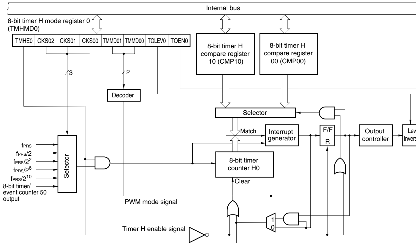
Figure 8-1. Block Diagram of 8-Bit Timer H0 (78K0/KB2-L, 78K0/KC2-L Only)
