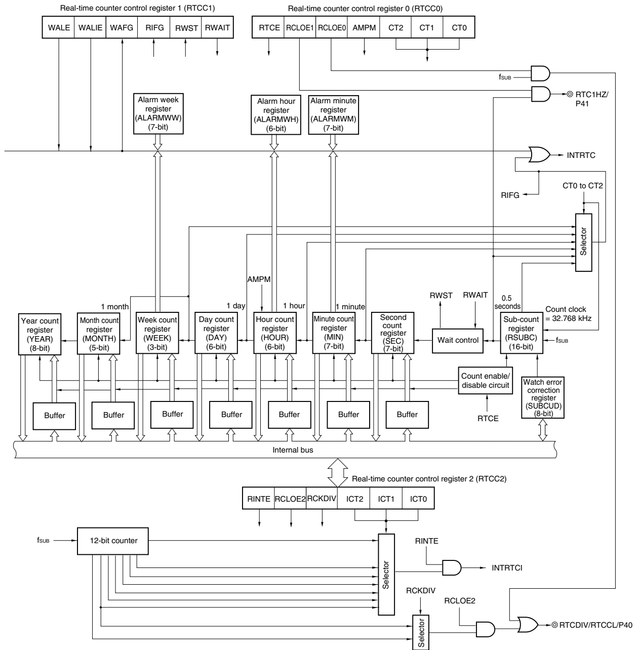
Figure 10-1. Block Diagram of Real-Time Counter
