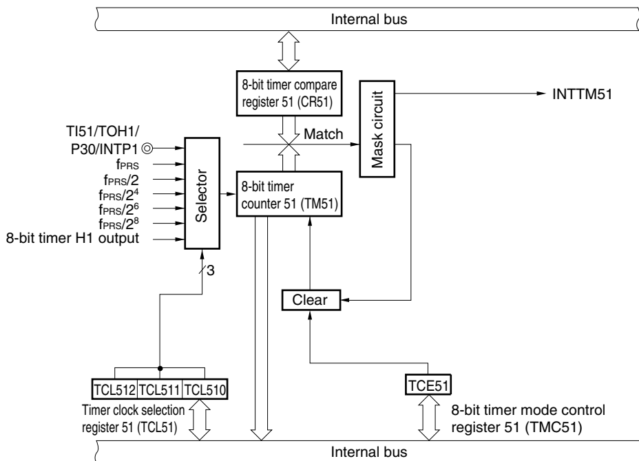
<R> Figure 7-2. Block Diagram of 8-Bit Timer 51 (78K0/KY2-L, 78K0/KA2-L (20-pin products))
