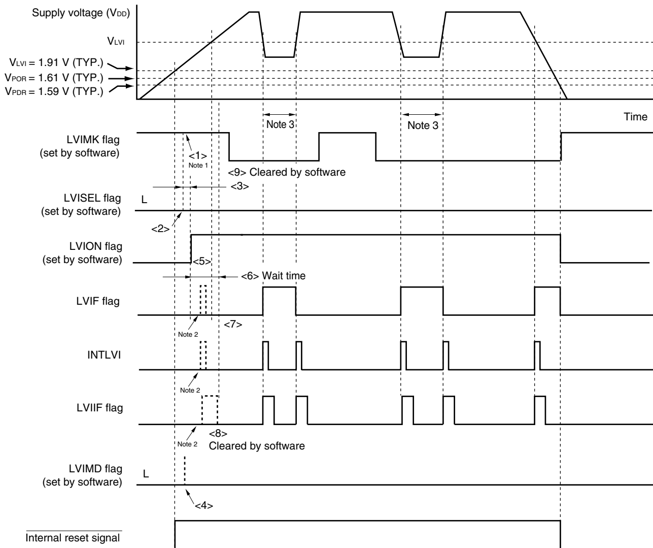
<R> Figure 22-9. Timing of Low-Voltage Detector Interrupt Signal Generation (Bit: LVISEL = 0, Option Byte: LVISTART = 1)
