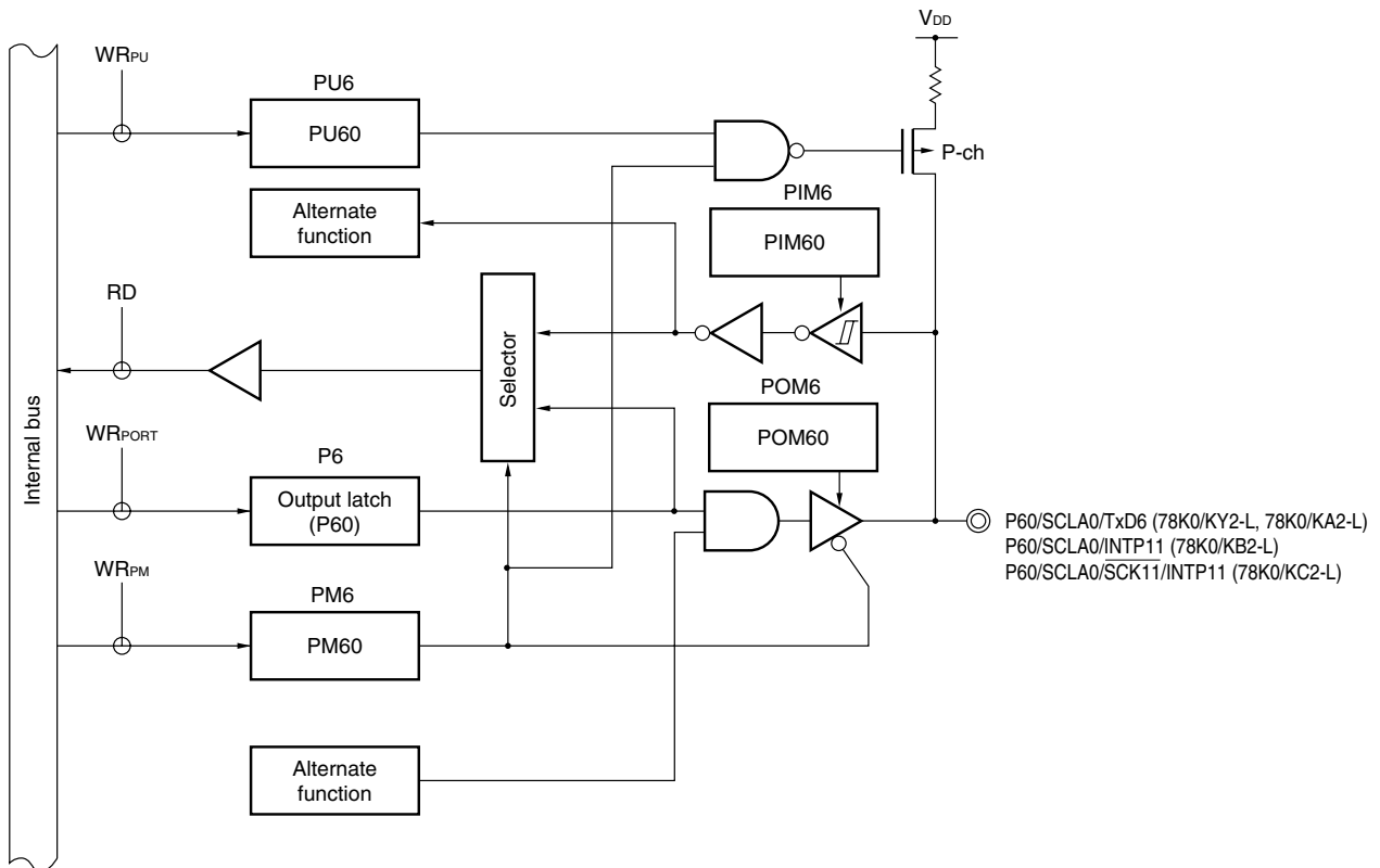
Figure 4-22. Block Diagram of P60
