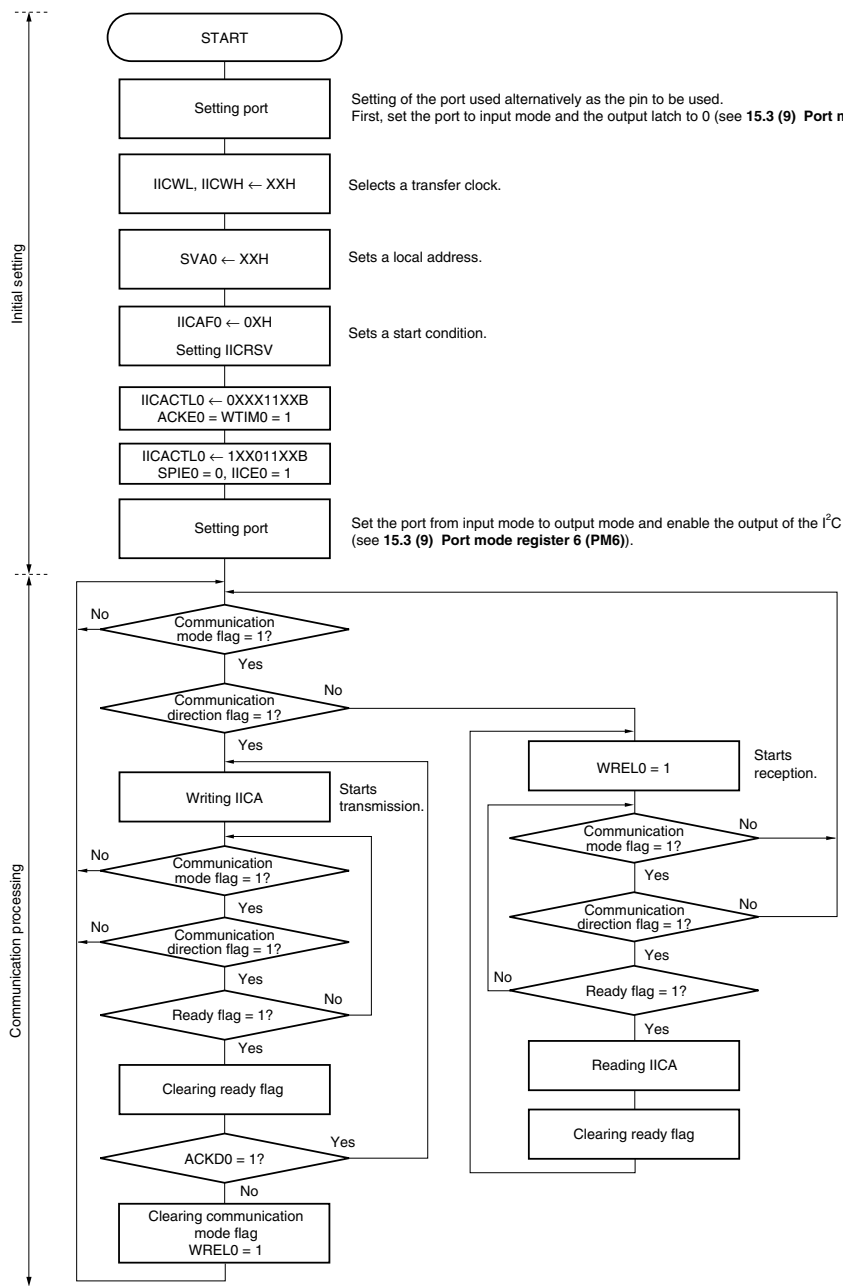
Figure 15-31. Slave Operation Flowchart (1)
