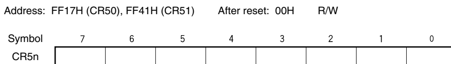
Figure 7-6. Format of 8-Bit Timer Compare Register 5n (CR5n)
