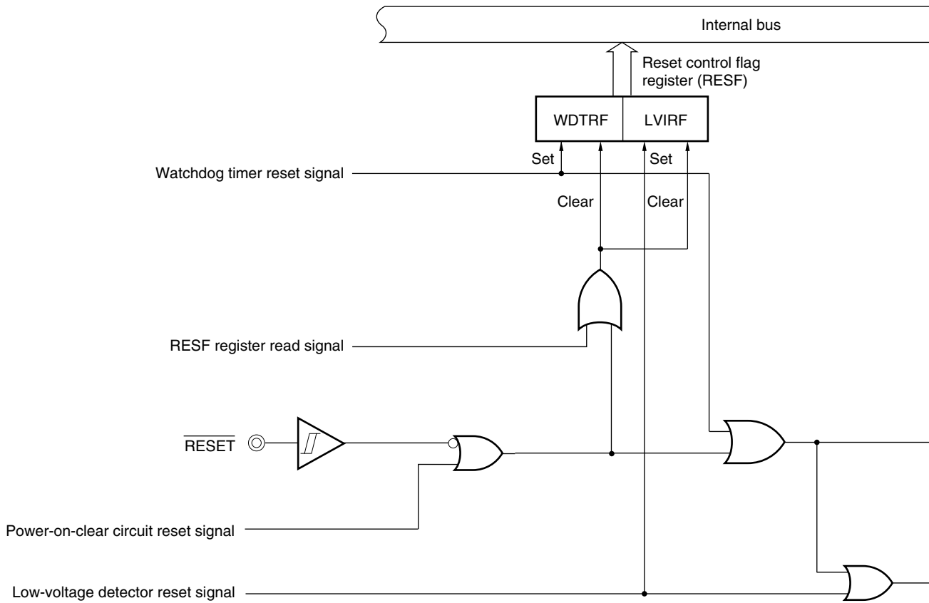
Figure 20-1. Block Diagram of Reset Function
