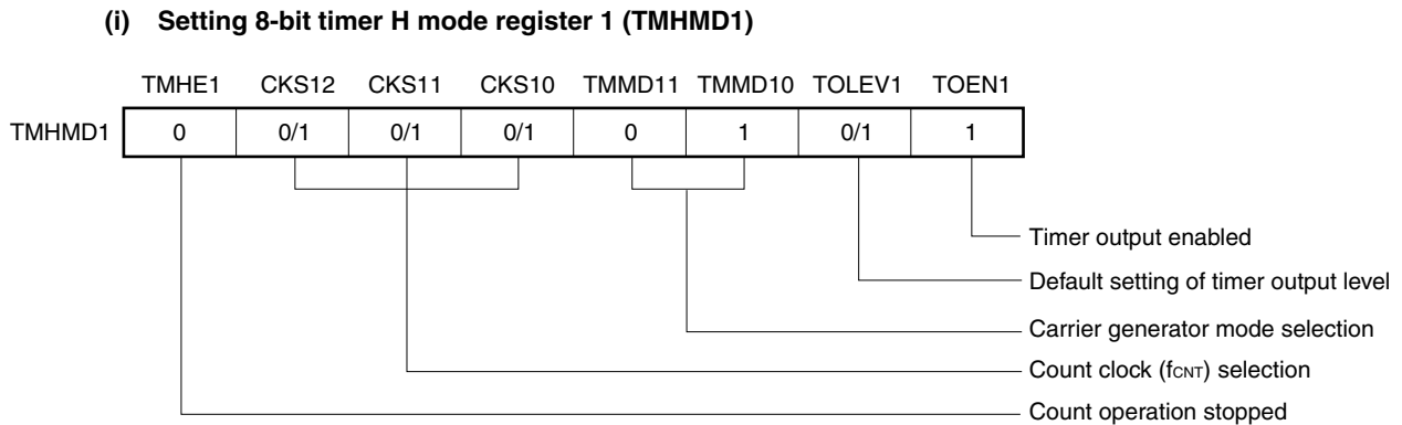
Figure 8-17. Register Setting in Carrier Generator Mode
