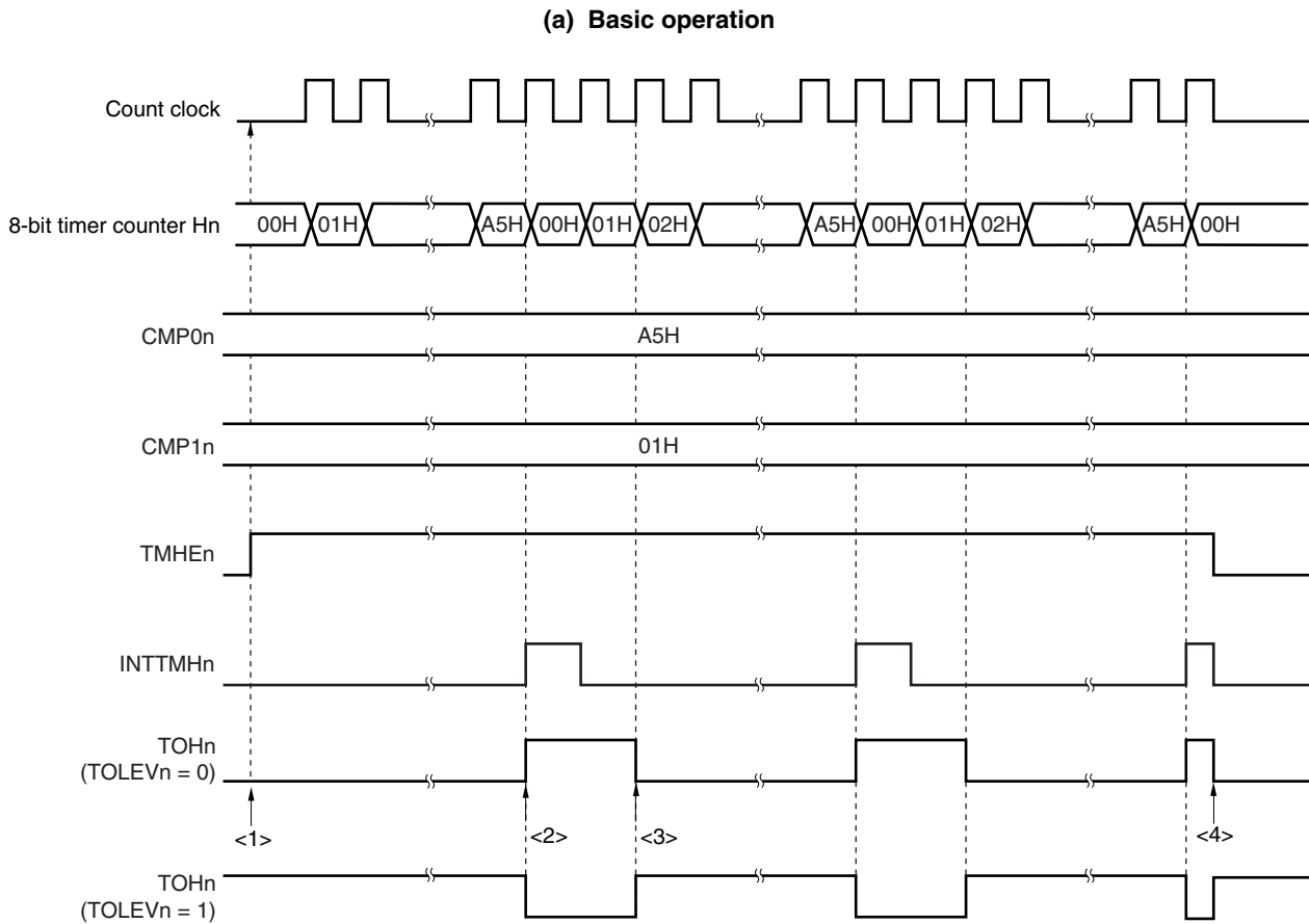
Figure 8-15. Operation Timing in PWM Output Mode (1/4)
