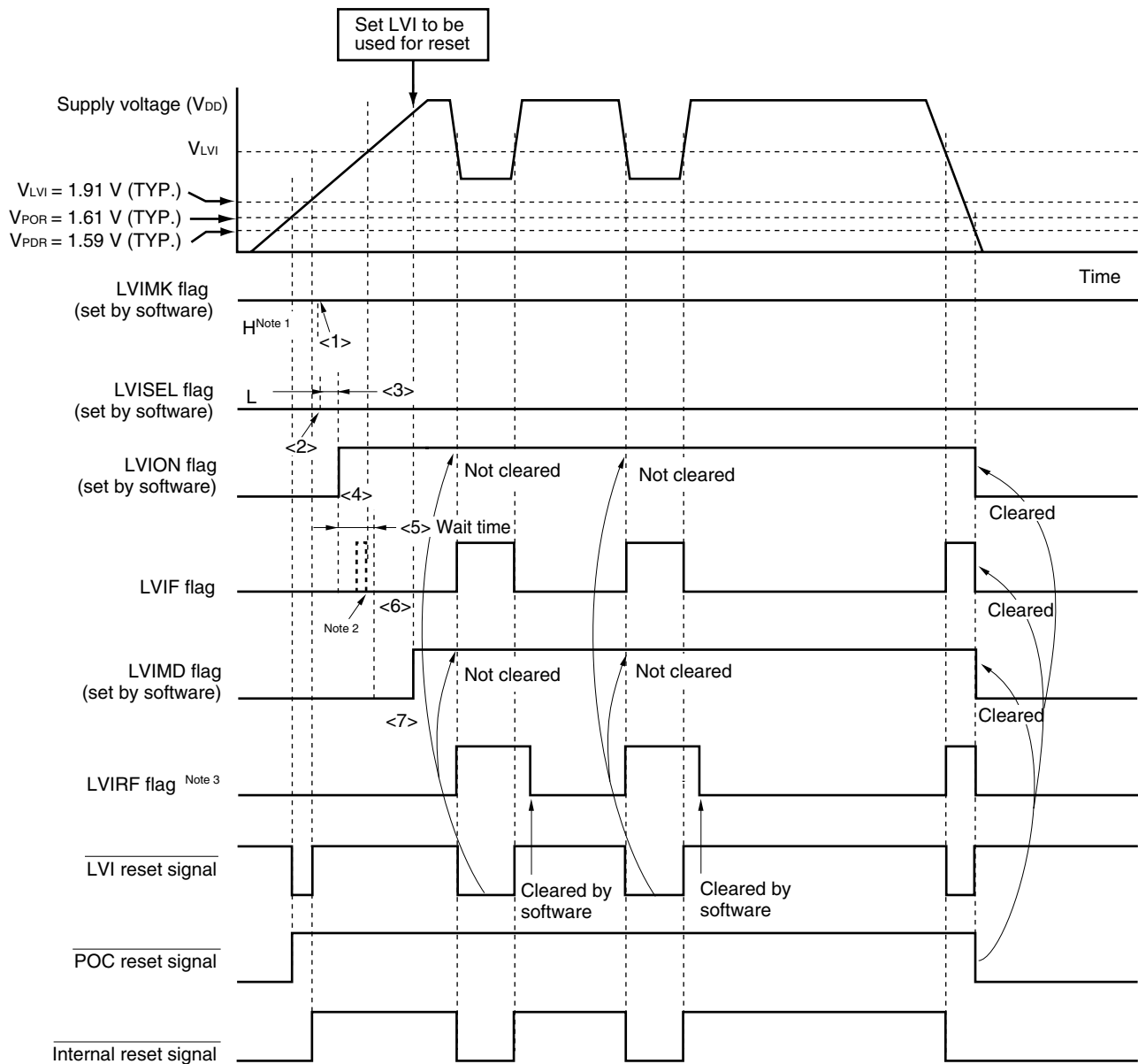
<R> Figure 22-6. Timing of Low-Voltage Detector Internal Reset Signal Generation (Bit: LVISEL = 0, Option Byte: LVISTART = 1)
