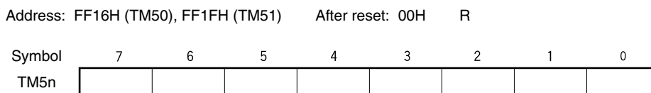
Figure 7-5. Format of 8-Bit Timer Counter 5n (TM5n)
