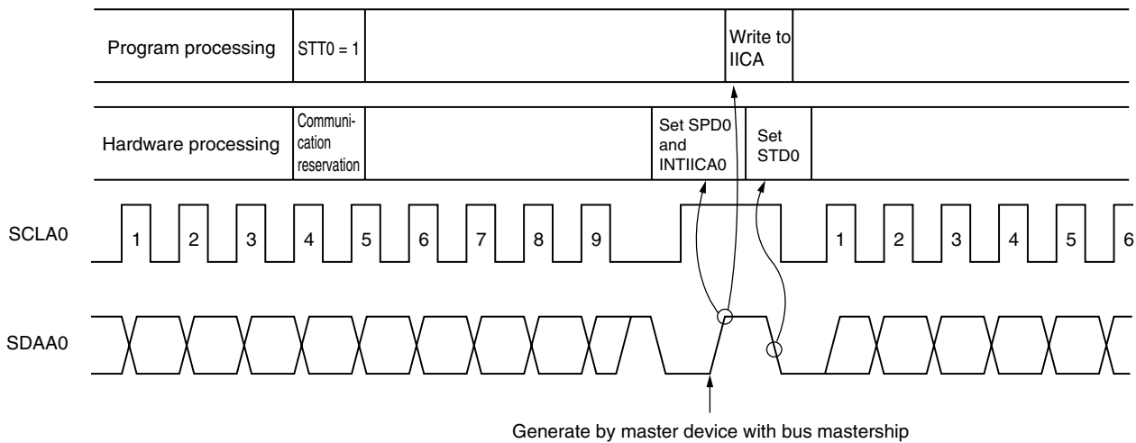
Figure 15-26. Communication Reservation Timing
