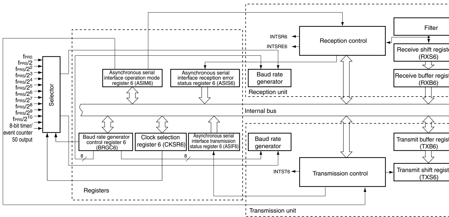
Figure 10-1. Block Diagram of Serial Interface UART6
