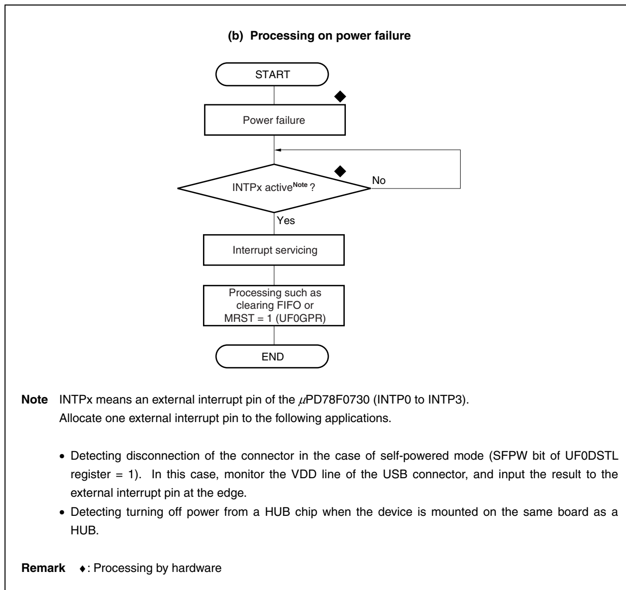
Figure 12-25. Example of Processing After Power Application/Power Failure (3/3)
