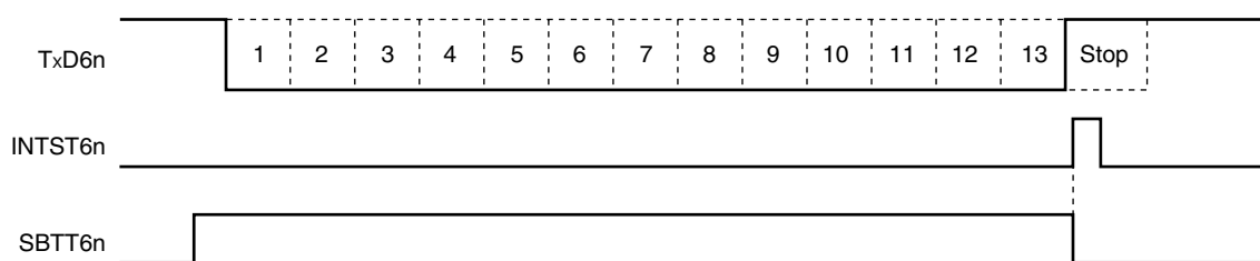
Figure 13-30. SBF Transmission
