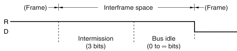
Figure 15-13. Interframe Space (Error Active Node)
