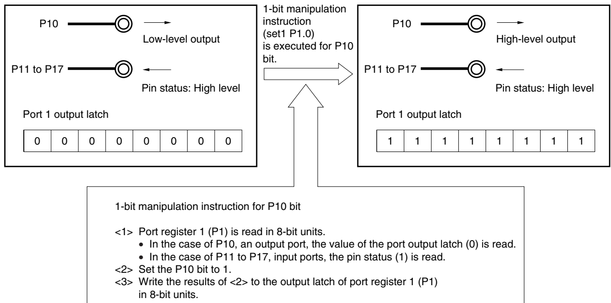
Figure 4-24. Bit Manipulation Instruction (P10)
