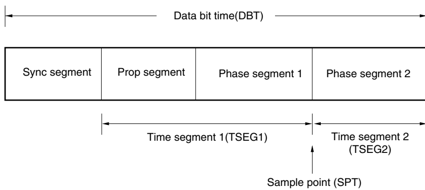
Figure 15-18. Segment Setting
