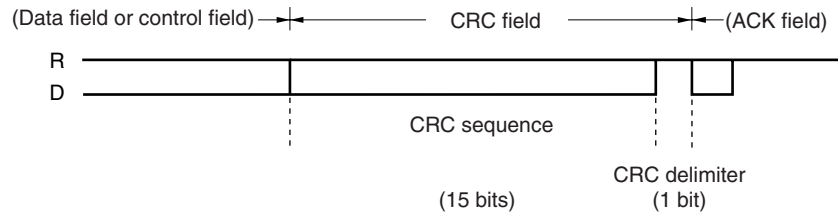
Figure 15-10. CRC Field
