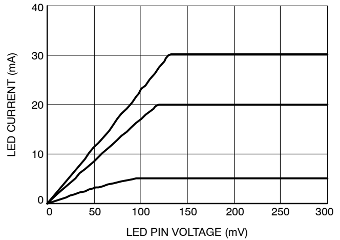
Figure 11. Dropout Characteristics
