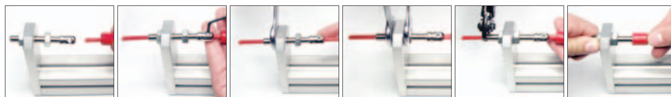
Rope insertion
