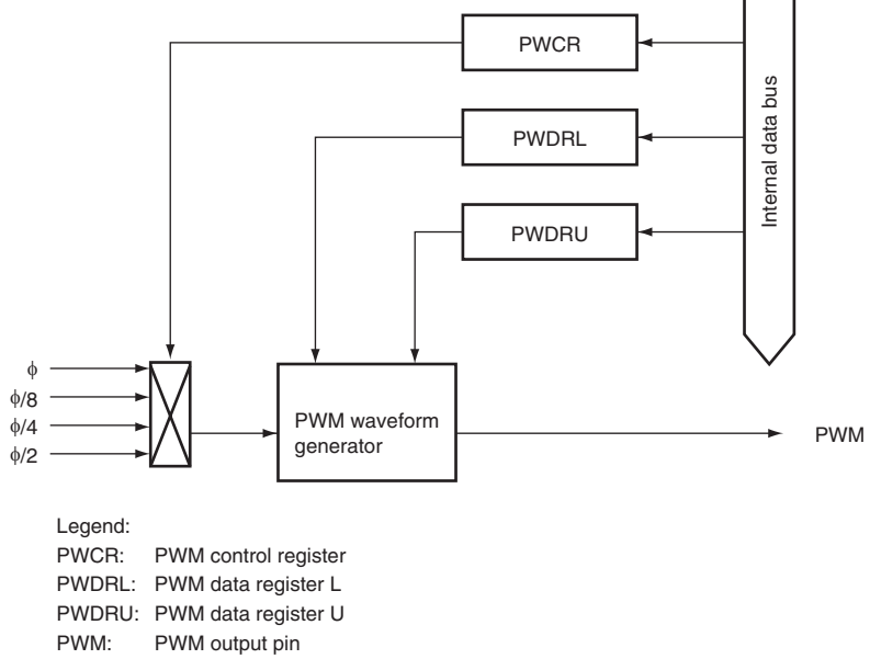
Figure 11.1(1) Block Diagram of 10-Bit PWM (H8/3802 Group, H8/38004 Group, H8/38002S Group)
