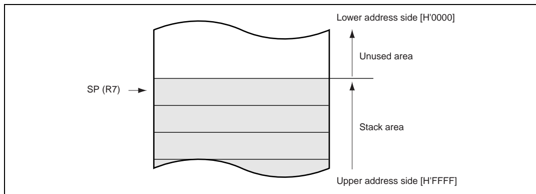
Figure 2.3 Stack Pointer
