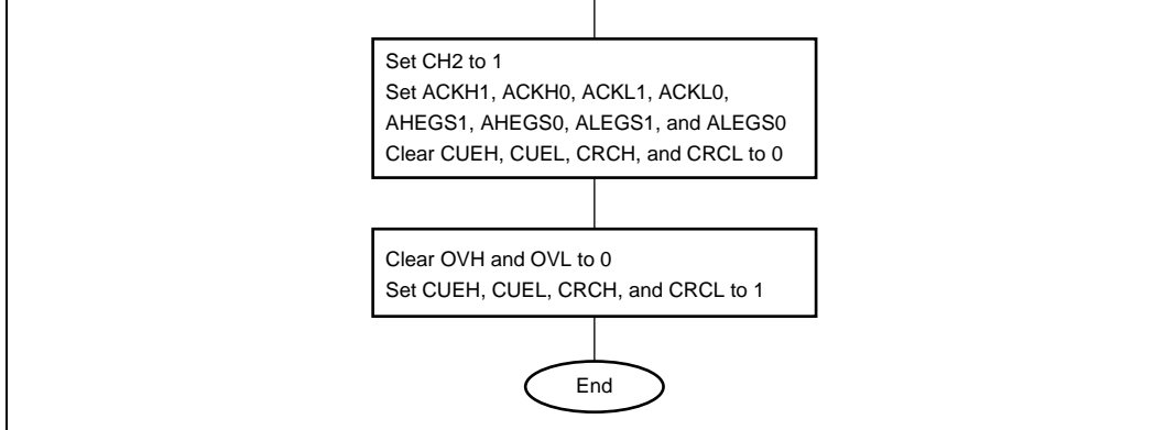
Figure 9.9 Example of Software Processing when Using ECH and ECL as 8-Bit Event Counters
