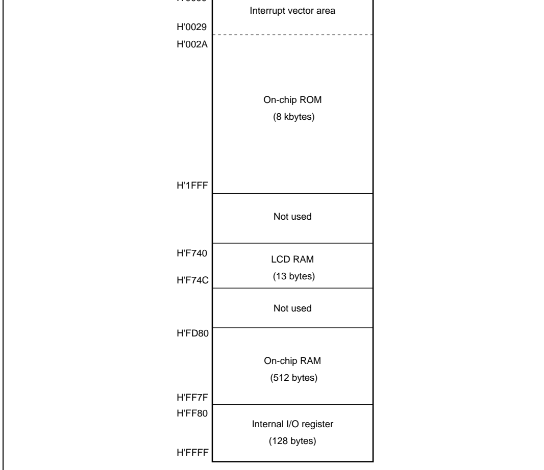
Figure 2.1(3) H8/3800 Memory Map
