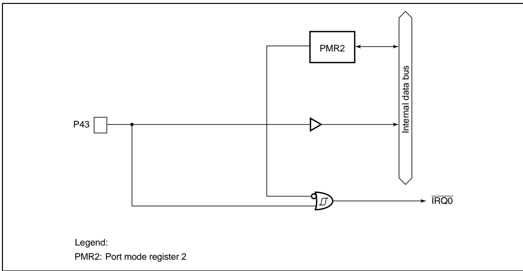
Figure B.2(a) Port 4 Block Diagram (Pin P43)
