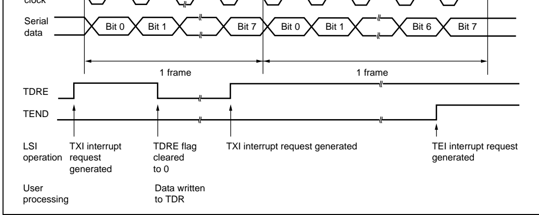
Figure 10.10 Example of SCI3 Operation in Transmission in Clocked Synchronous Mode
