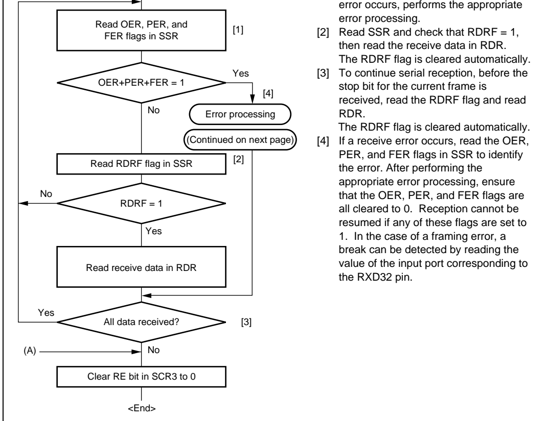
Figure 10.8 Sample Serial Data Reception Flowchart (Asynchronous Mode) (1)
