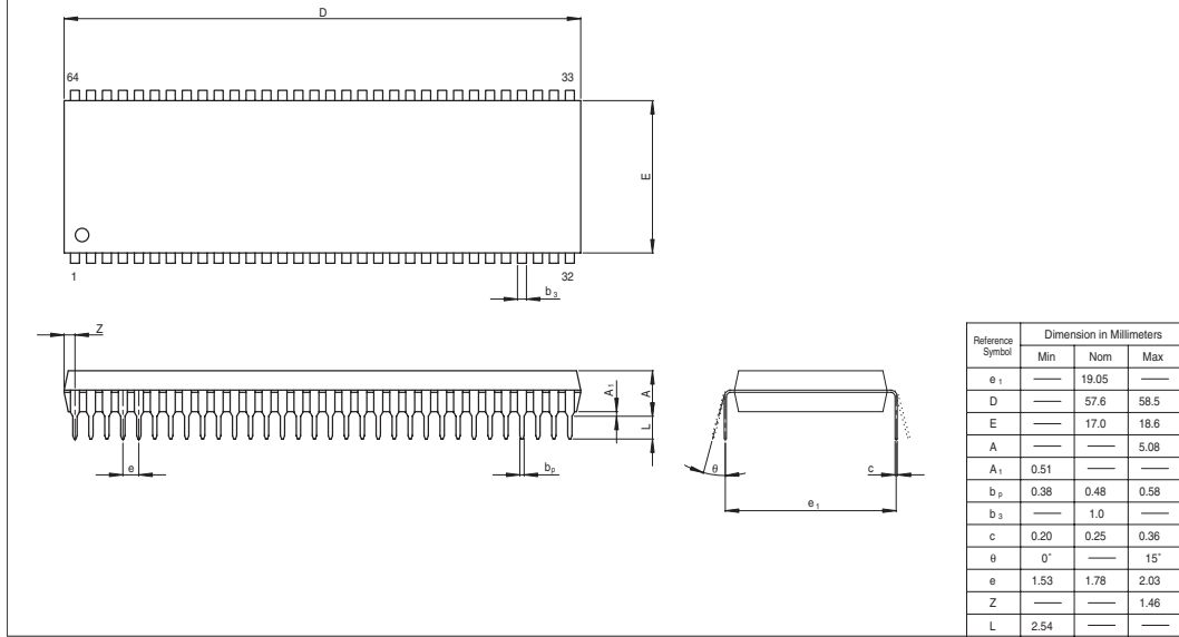
Figure E.4 Package Dimensions (DP-64S)
