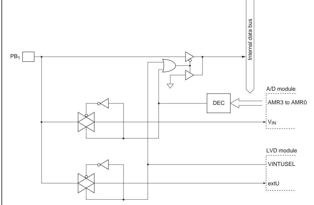
Figure B.9(c) Port B Block Diagram (Pin PB1, H8/38104 Group Only)
