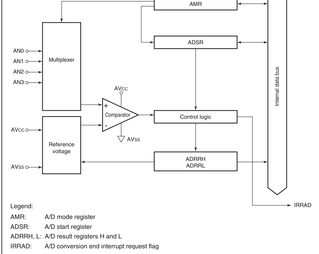
Figure 12.1 Block Diagram of A/D Converter
