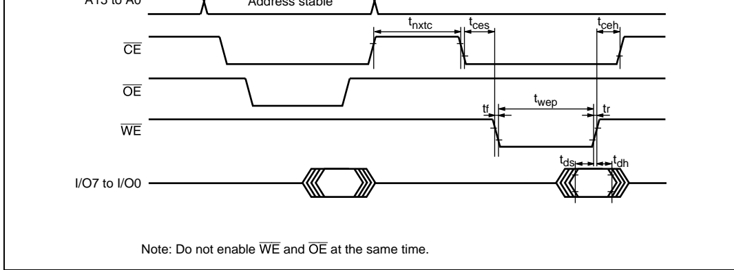
Figure 6.14 Timing Waveforms in Transition from Memory Read Mode to Another Mode
