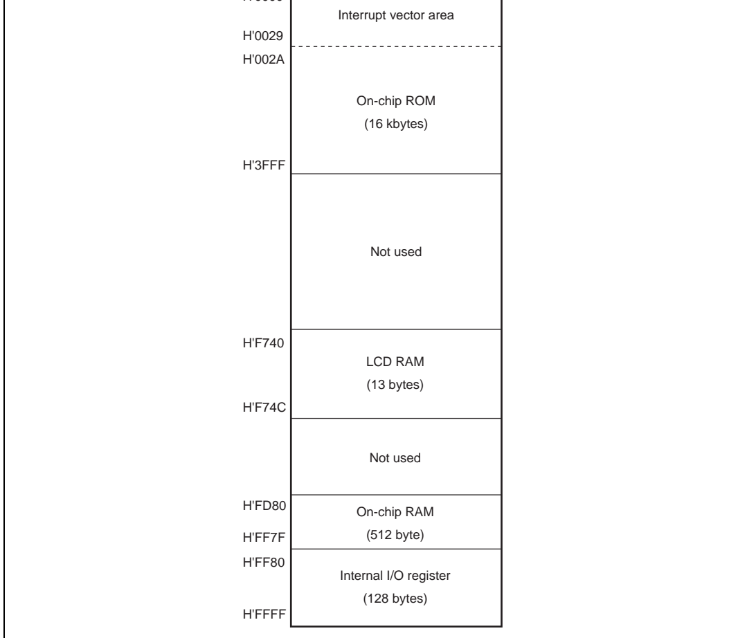
Figure 2.1(7) H8/38002S Memory Map
