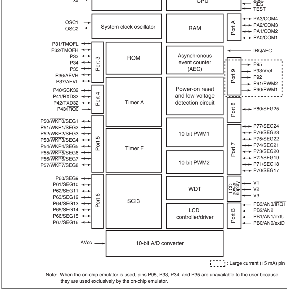
Figure 1.3 Internal Block Diagram of H8/38104 Group
