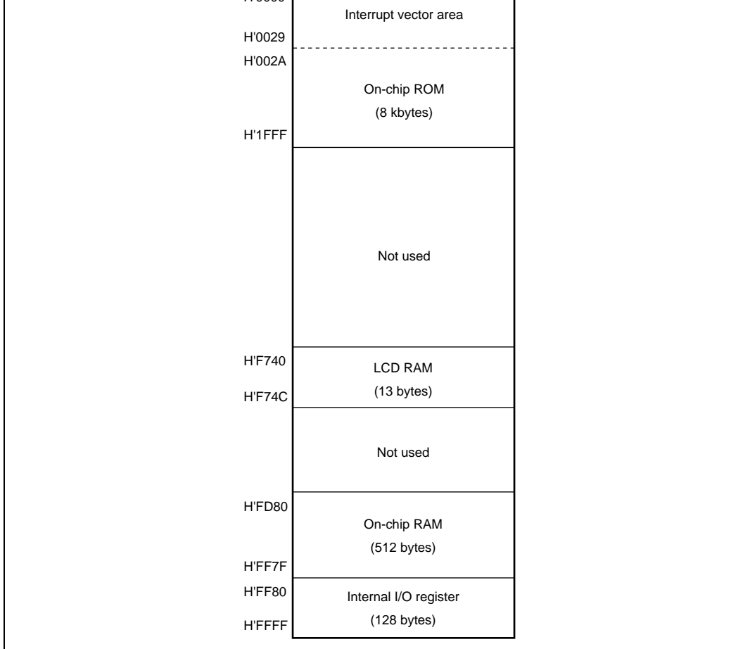
Figure 2.1(9) H8/38000, H8/38000S, H8/38100 Memory Map
