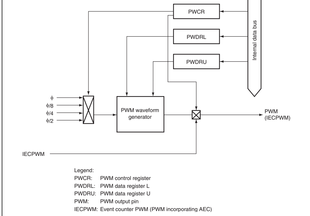
Figure 11.1(2) Block Diagram of 10-Bit PWM (H8/38104 Group)
