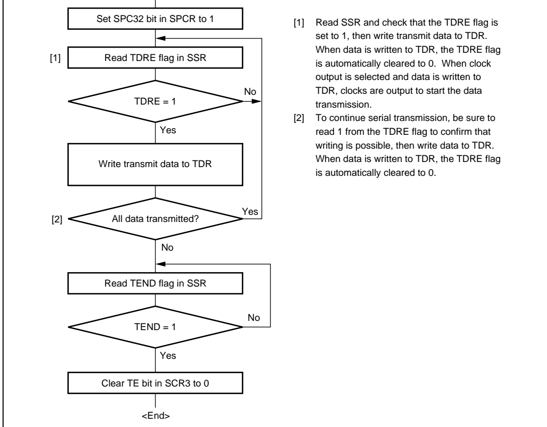
Figure 10.11 Sample Serial Transmission Flowchart (Clocked Synchronous Mode)
