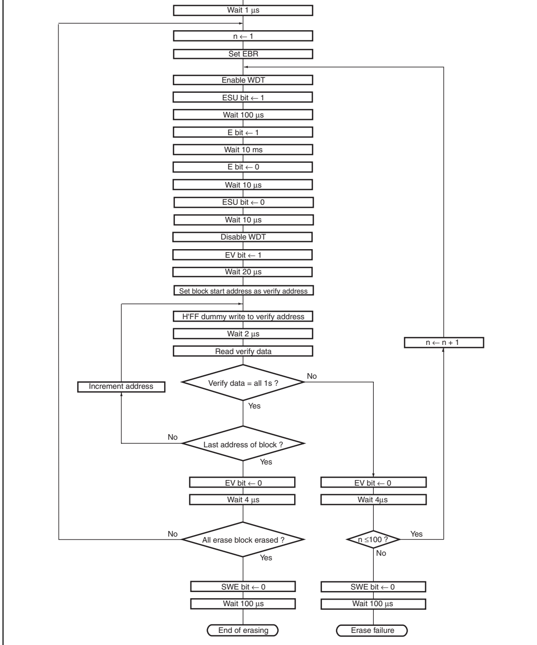
Figure 6.11 Erase/Erase-Verify Flowchart
