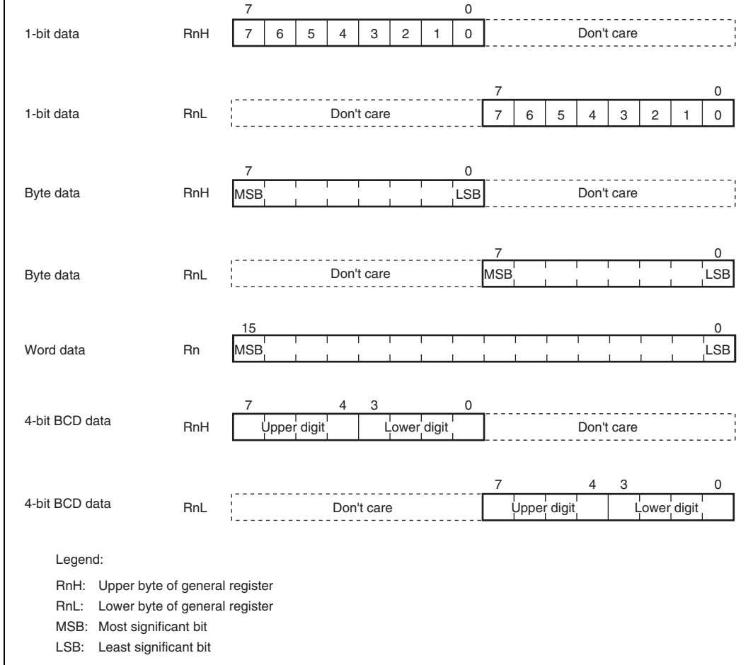
Figure 2.4 General Register Data Formats
