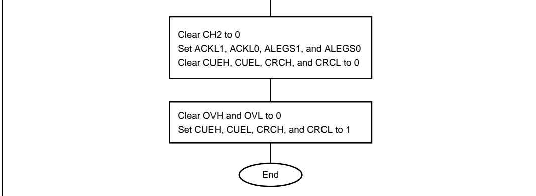
Figure 9.8 Example of Software Processing when Using ECH and ECL as 16-Bit Event Counter
