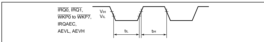
Figure 17.4 Input Timing
