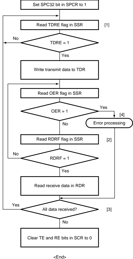
Figure 10.14 Sample Flowchart of Simultaneous Serial Transmit and Receive Operations (Clocked Synchronous Mode)
