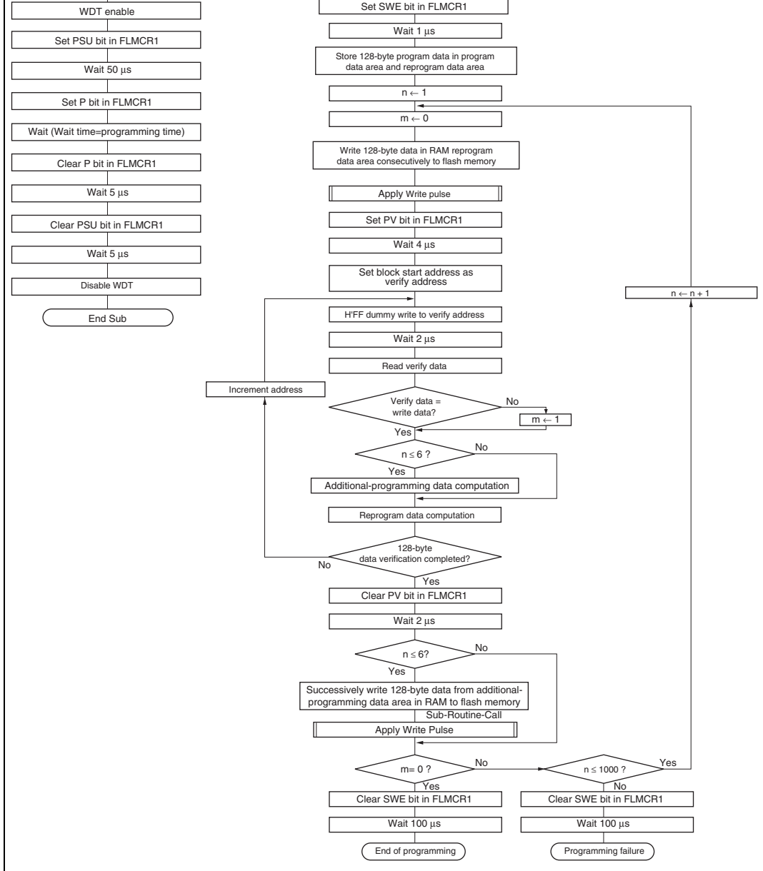
Figure 6.10 Program/Program-Verify Flowchart
