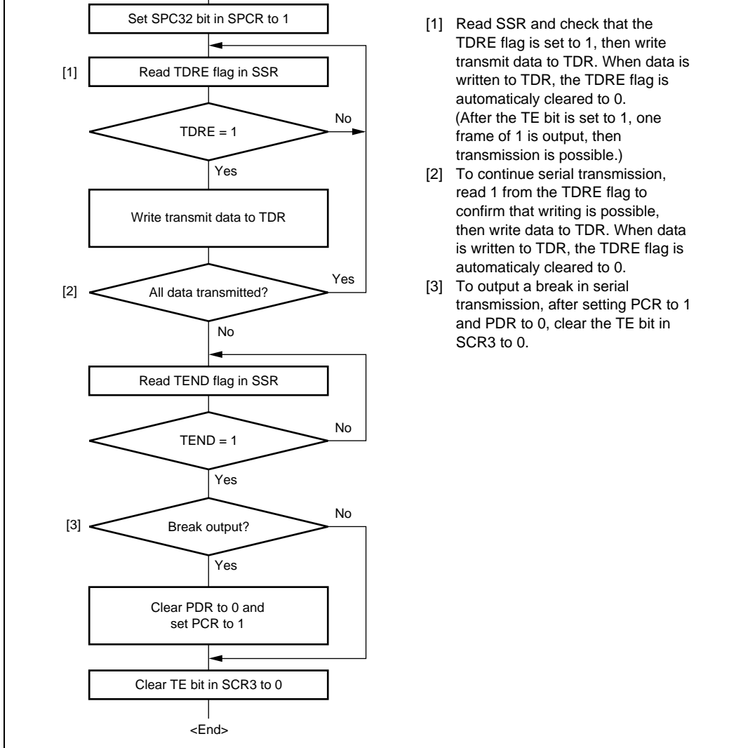
Figure 10.6 Sample Serial Transmission Flowchart (Asynchronous Mode)
