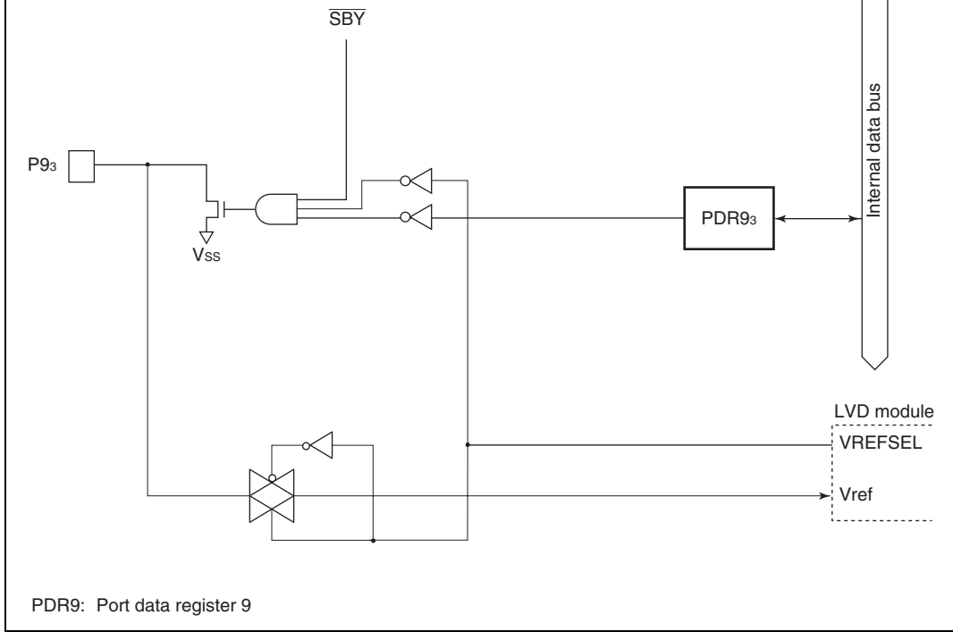
Figure B.7(c) Port 9 Block Diagram (Pin P93, H8/38104 Group Only)
