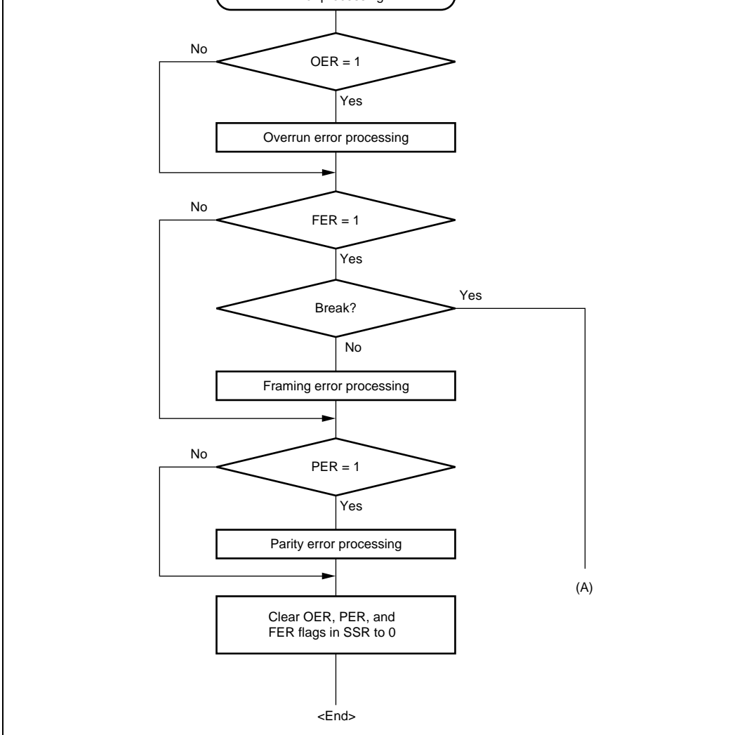
Figure 10.8 Sample Serial Data Reception Flowchart (Asynchronous Mode) (2)
