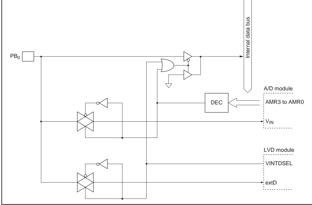
Figure B.9(b) Port B Block Diagram (Pin PB0, H8/38104 Group Only)
