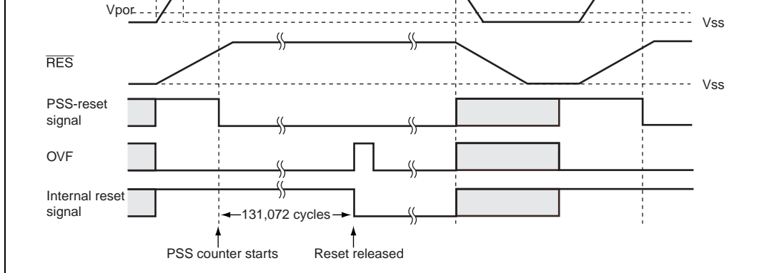
Figure 14.2 Operational Timing of Power-On Reset Circuit
