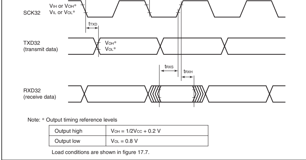
Figure 17.6 SCI3 Input/Output Timing in Clocked Synchronous Mode
