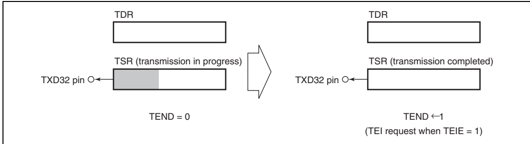
Figure 10.15(c) TEND Setting and TEI Interrupt
