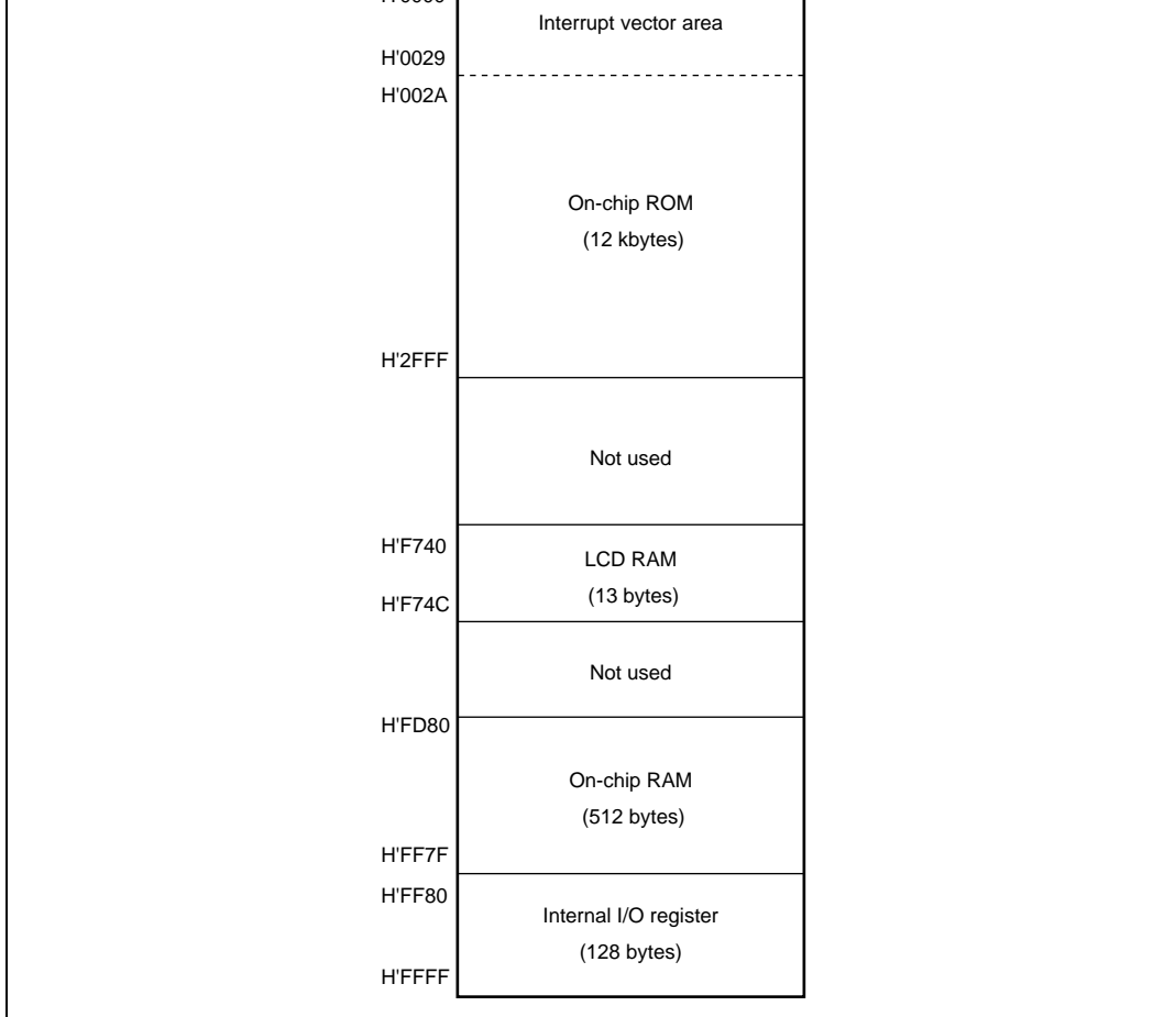
Figure 2.1(2) H8/3801 Memory Map
