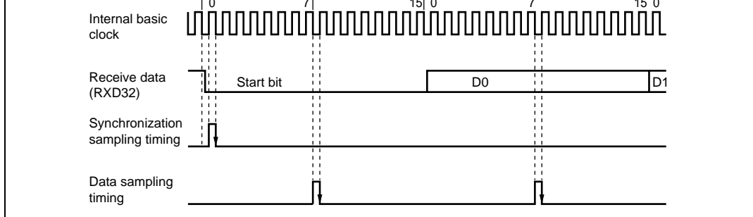
Figure 10.16 Receive Data Sampling Timing in Asynchronous Mode
