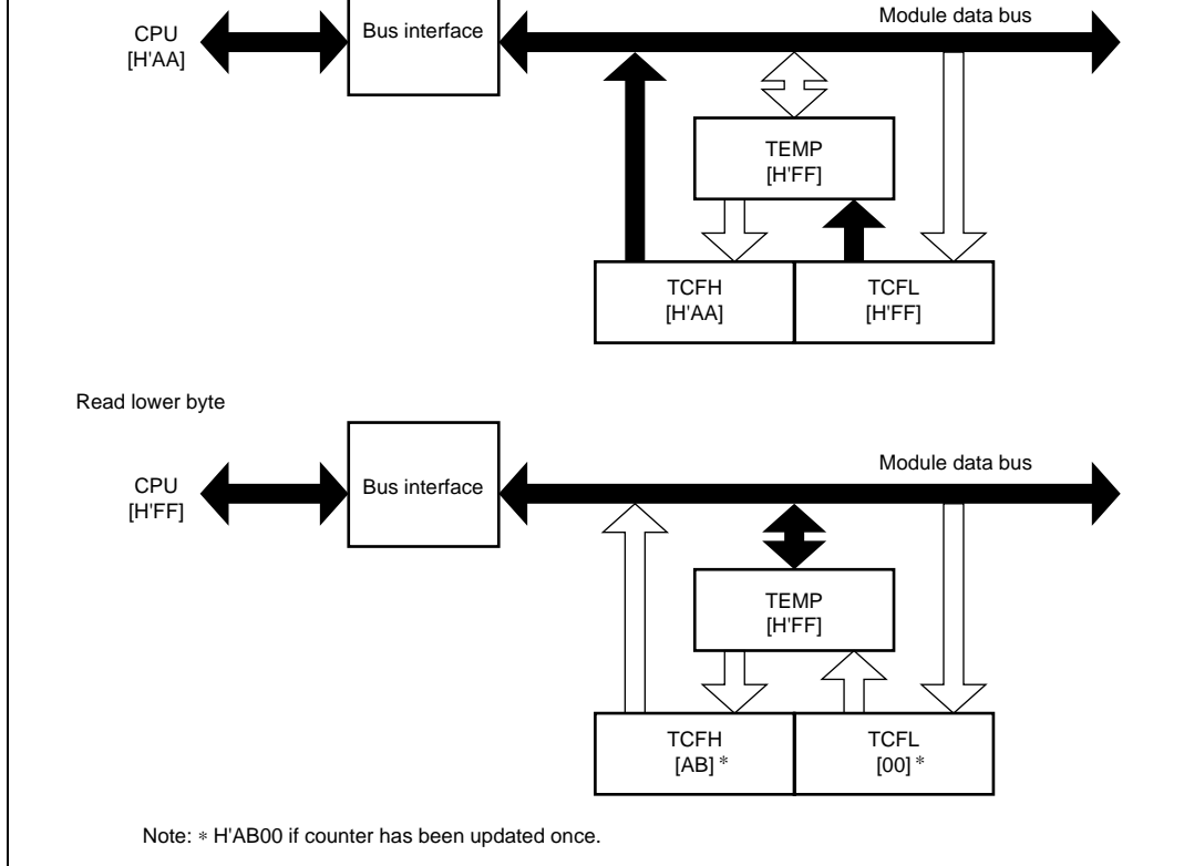
Figure 9.4 Read Access to TCF (TCF → CPU)
