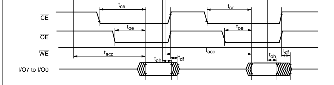
Figure 6.16 Timing Waveforms in \overline{\text{CE}} and \overline{\text{OE}} Clock System Read
