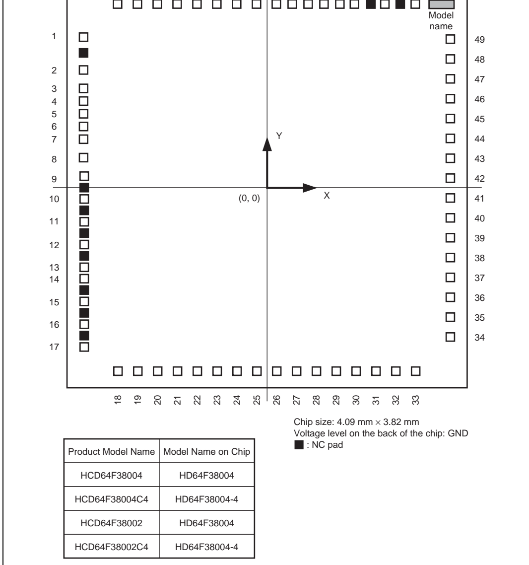
Figure 1.9 Pad Arrangement of HCD64F38004 and HCD64F38002 (Top View)
