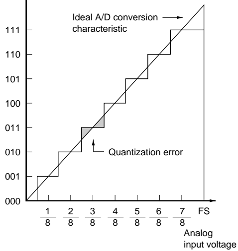
Figure 12.5 A/D Conversion Accuracy Definitions (1)
