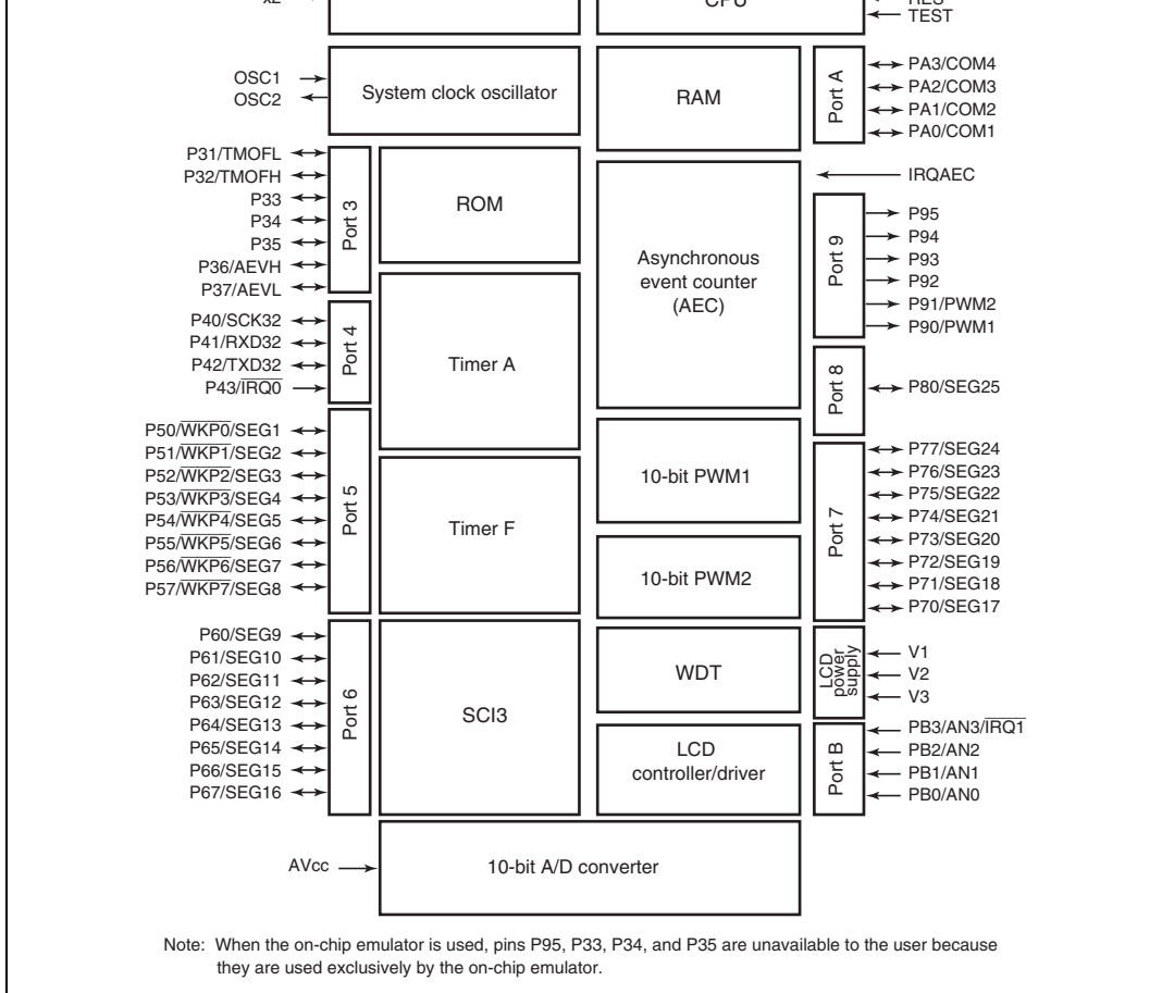
Figure 1.2 Internal Block Diagram of H8/38004 and H8/38002S Group
