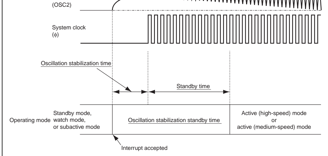
Figure 4.16 Oscillation Stabilization Standby Time
