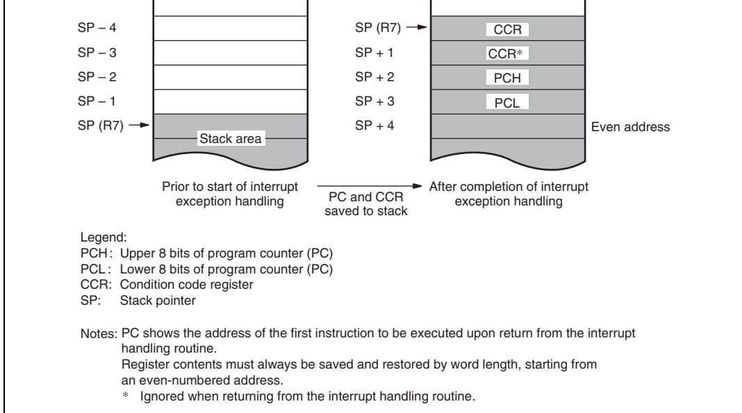
Figure 3.2 Stack Status after Exception Handling
