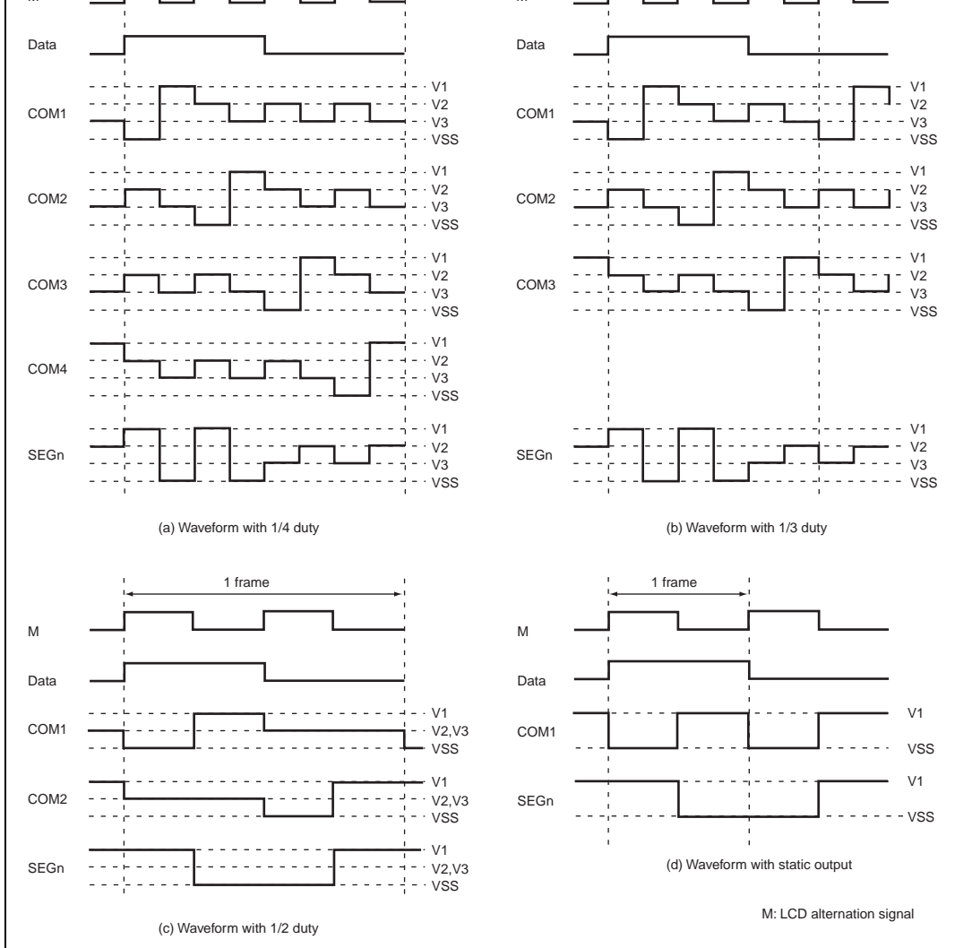
Figure 13.7 Output Waveforms for Each Duty Cycle (A Waveform)
