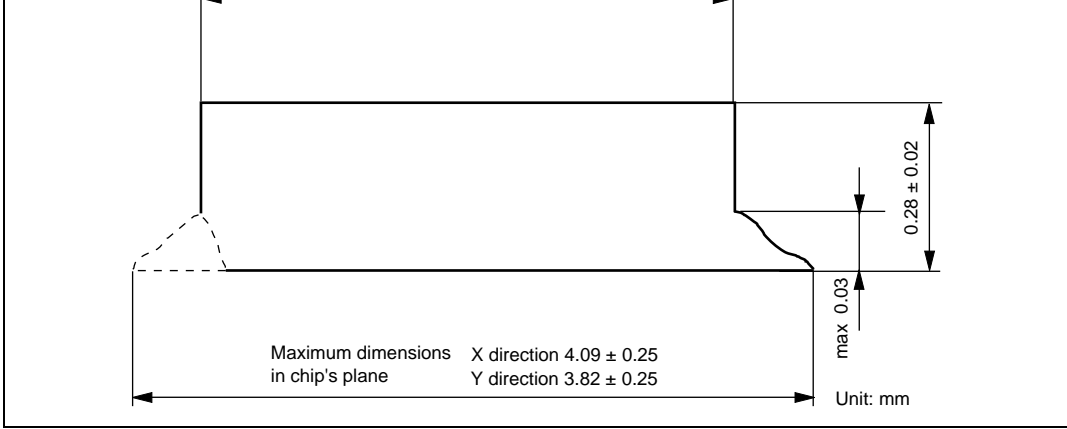
Figure F.3 Cross-Sectional View of Chip (HCD64F38004 and HCD64F38002)
