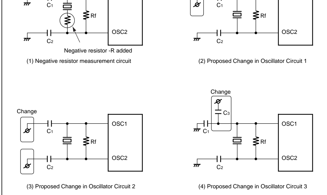
Figure 4.14 Negative Resistor Measurement and Proposed Changes in Circuit
