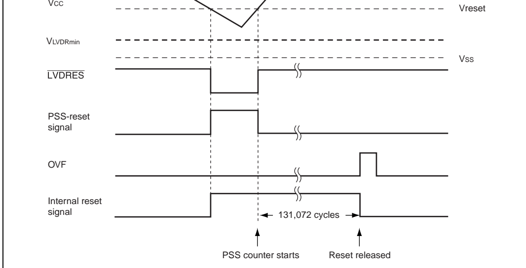
Figure 14.3 Operational Timing of LVDR Circuit
