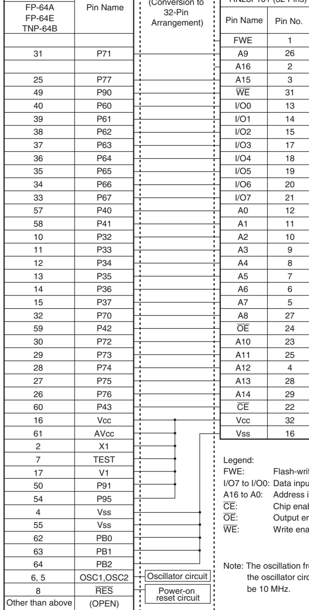
Figure 6.12(1) Socket Adapter Pin Correspondence Diagram (H8/38004F, H8/38002F)
