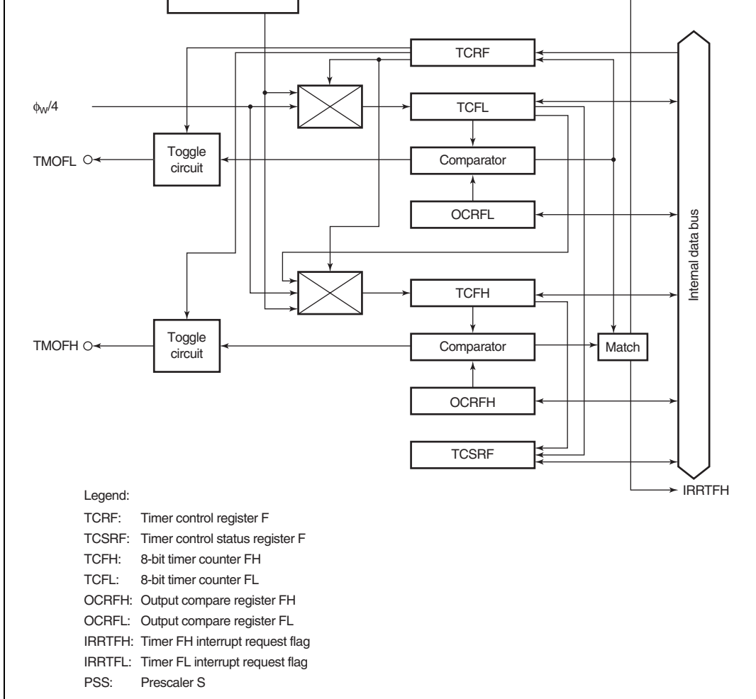
Figure 9.2 Block Diagram of Timer F
