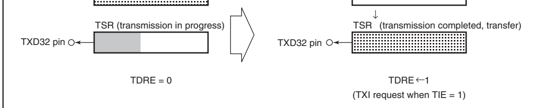
Figure 10.15(b) TDRE Setting and TXI Interrupt
