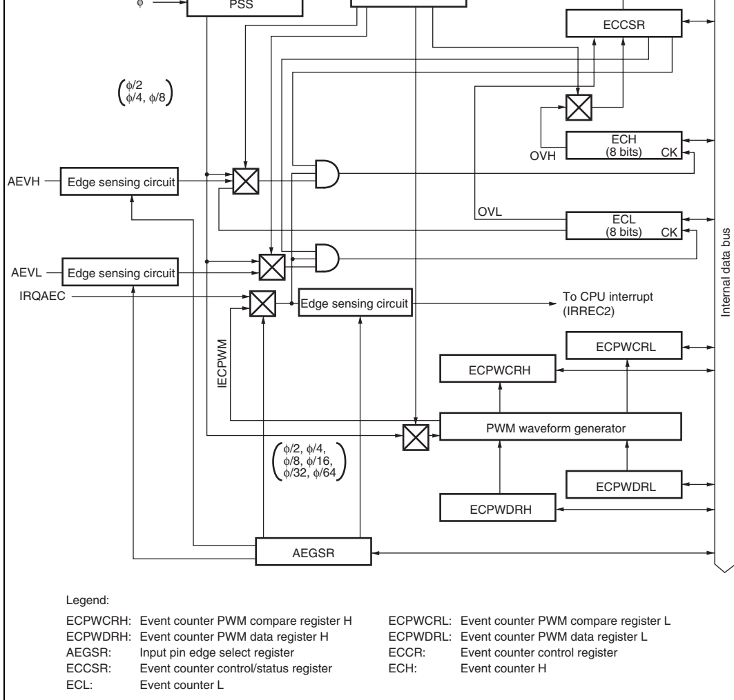
Figure 9.7 Block Diagram of Asynchronous Event Counter
