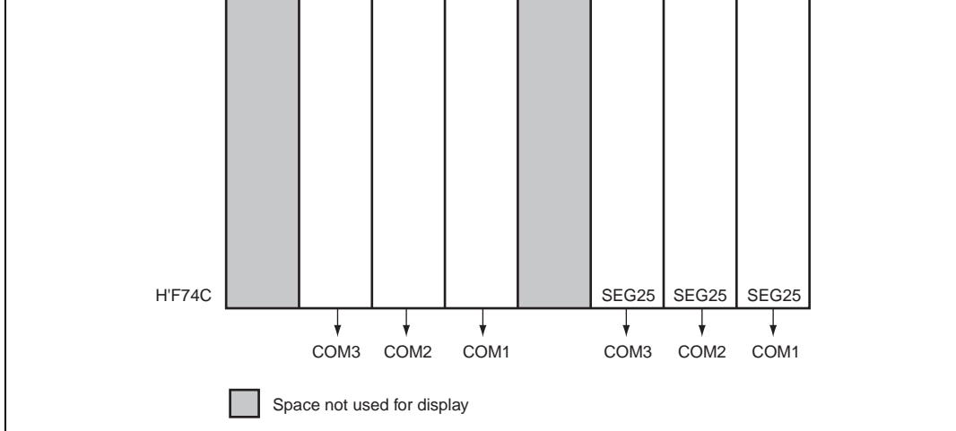
Figure 13.4 LCD RAM Map (1/3 Duty)
