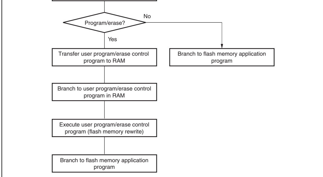
Figure 6.9 Programming/Erasing Flowchart Example in User Program Mode
