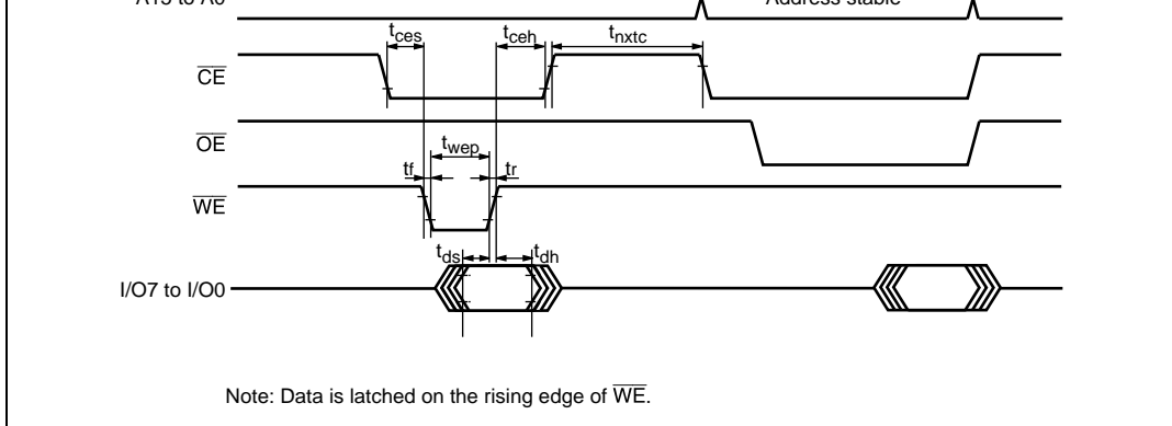
Figure 6.13 Timing Waveforms for Memory Read after Command Write
