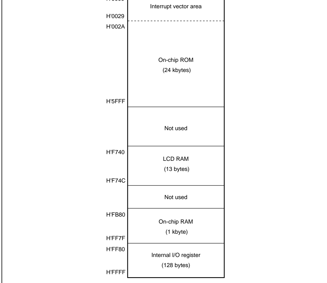
Figure 2.1(5) H8/38003, H8/38103 Memory Map
