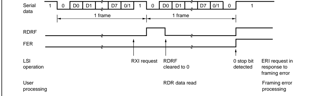
Figure 10.7 Example SCI3 Operation in Reception in Asynchronous Mode (8-Bit Data, Parity, One Stop Bit)
