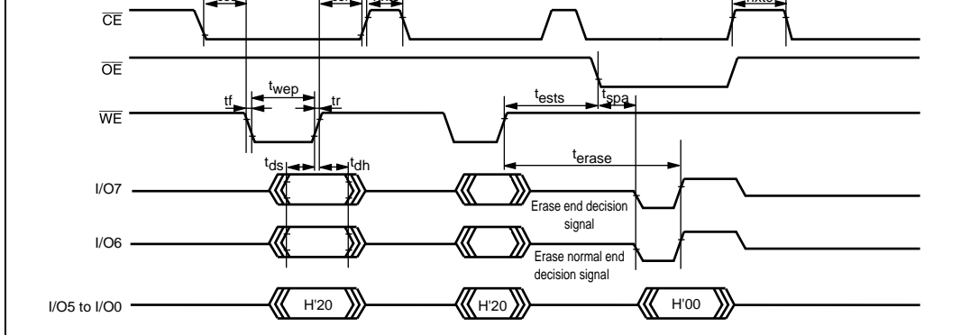
Figure 6.18 Timing Waveforms in Auto-Erase Mode
