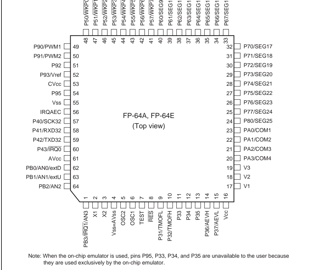
Figure 1.6 Pin Arrangement of H8/38104 Group (FP-64A, FP-64E)
