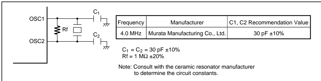
Figure 4.6(1) Typical Connection to Ceramic Resonator (H8/3802 Group)
