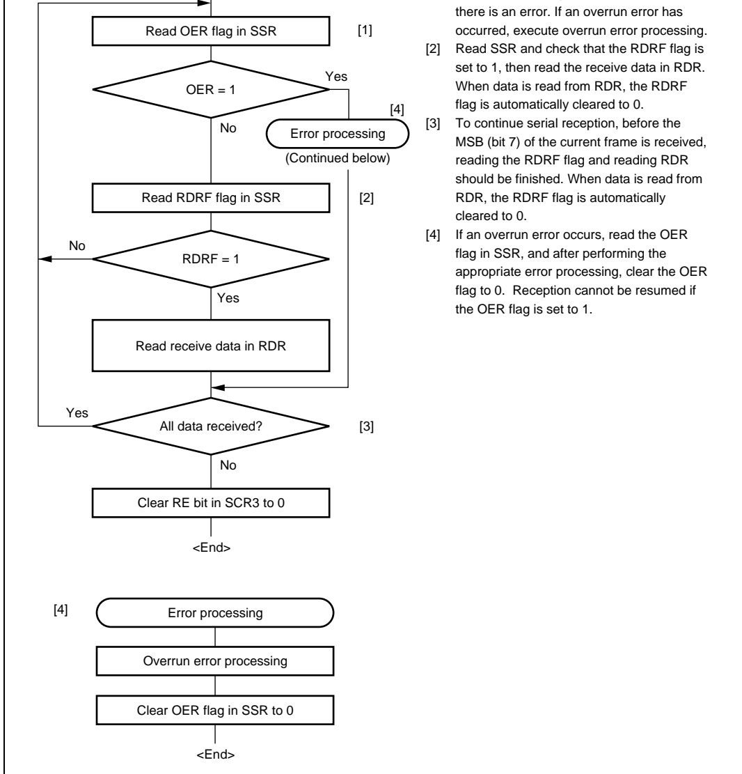
Figure 10.13 Sample Serial Reception Flowchart (Clocked Synchronous Mode)
