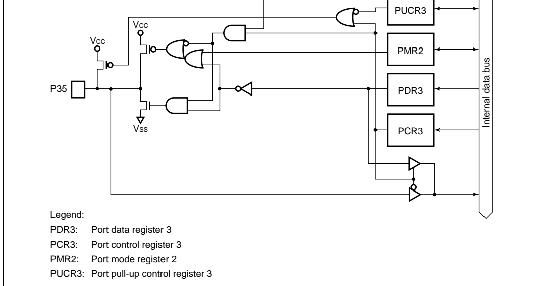
Figure B.1(b) Port 3 Block Diagram (Pin P35)
