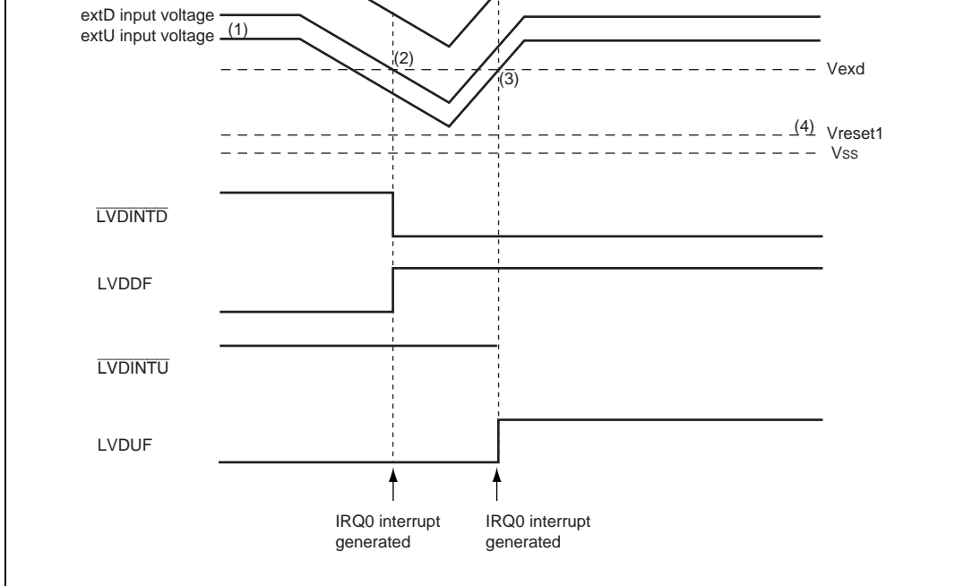
Figure 14.5 Operational Timing of Low-Voltage Detection Interrupt Circuit (Using Pins Vref, extD, and extU)
