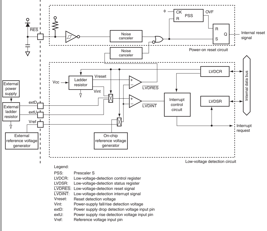
Figure 14.1 Block Diagram of Power-On Reset Circuit and Low-Voltage Detection Circuit
