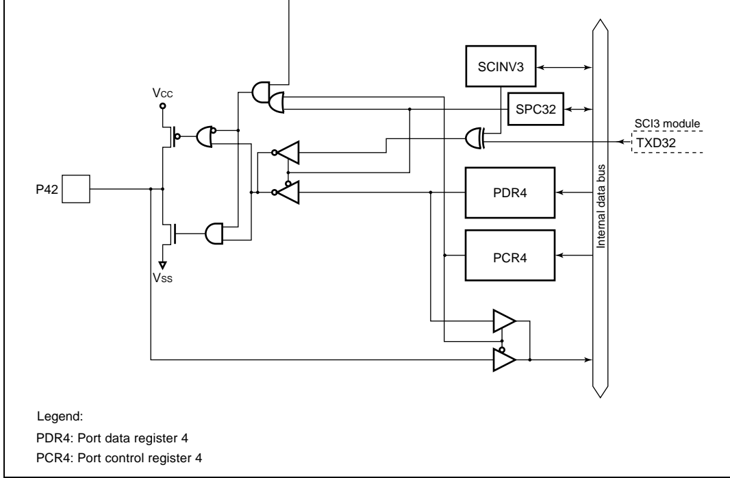
Figure B.2(b) Port 4 Block Diagram (Pin P42)
