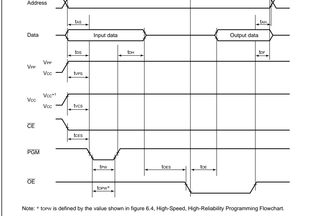
Figure 6.5 PROM Write/Verify Timing
