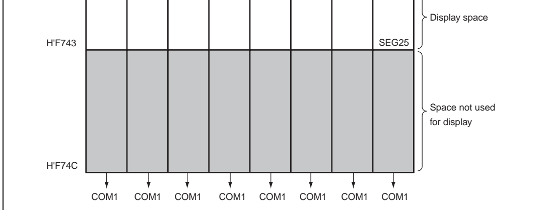
Figure 13.6 LCD RAM Map (Static Mode)
