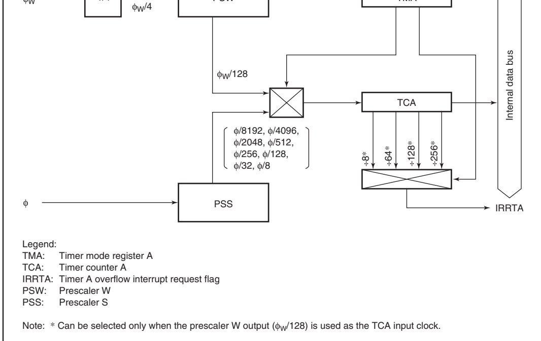
Figure 9.1 Block Diagram of Timer A
