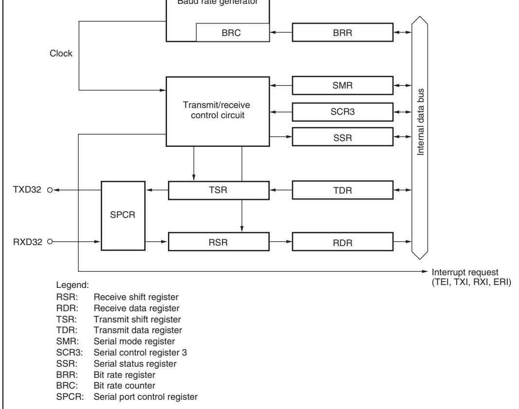
Figure 10.1 Block Diagram of SCI3
