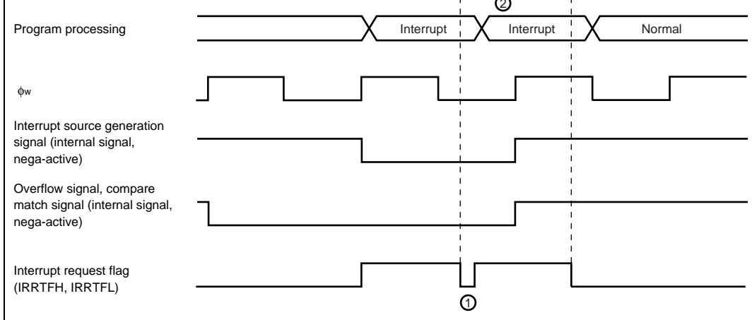
Figure 9.6 Clear Interrupt Request Flag when Interrupt Source Generation Signal Is Valid
