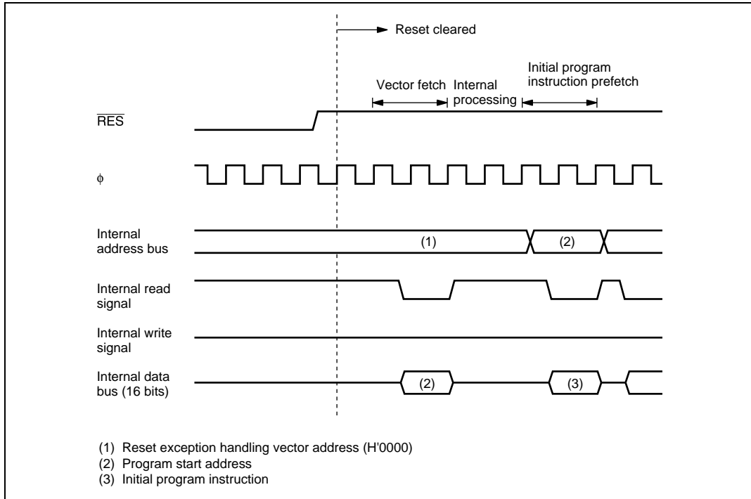
Figure 3.1 Reset Sequence
