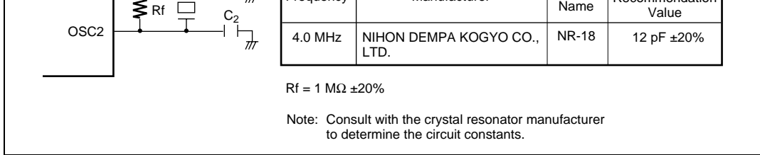
Figure 4.4(2) Typical Connection to Crystal Resonator (H8/38004, H8/38002S, H8/38104 Group)
