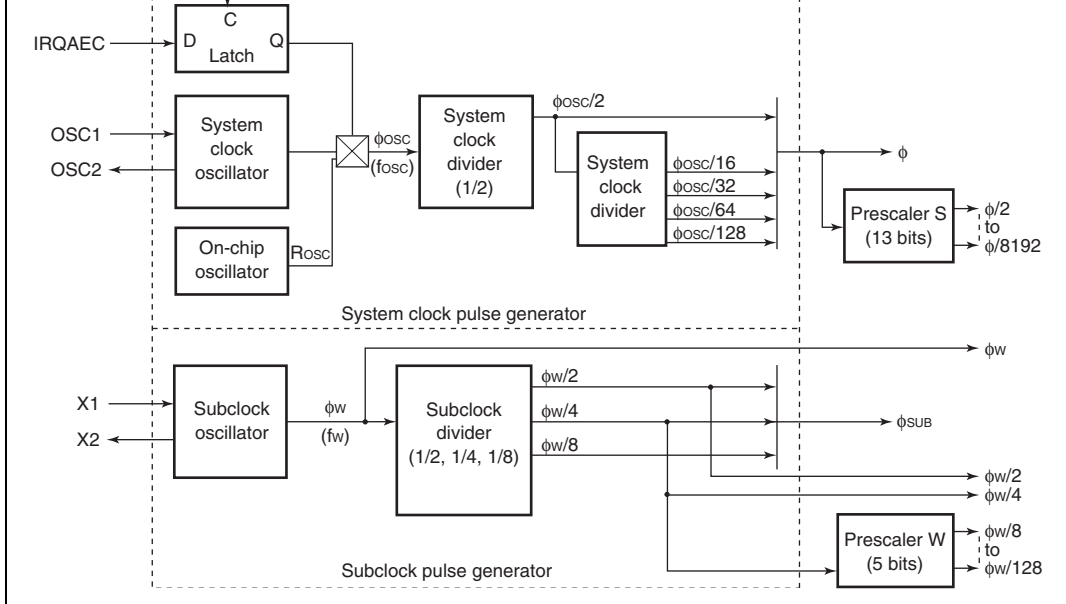
Figure 4.2 Block Diagram of Clock Pulse Generators (H8/38104 Group)
