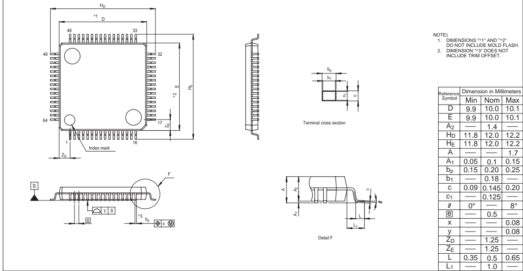
Figure E.3 Package Dimensions (FP-64K)
