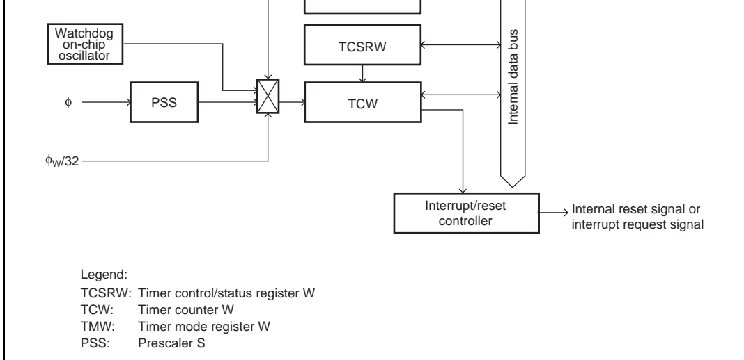
Figure 9.12(2) Block Diagram of Watchdog Timer (H8/38104 Group)
