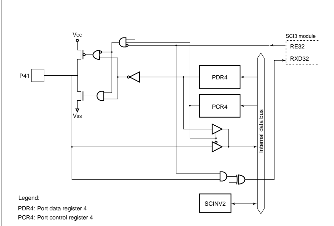
Figure B.2(c) Port 4 Block Diagram (Pin P41)
