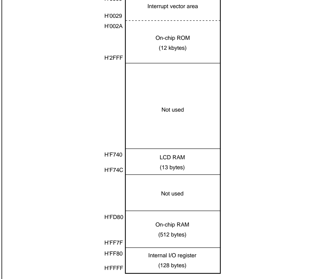
Figure 2.1(8) H8/38001, H8/38001S, H8/38101 Memory Map
