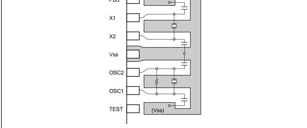
Figure 4.13 Example of Crystal and Ceramic Resonator Arrangement
