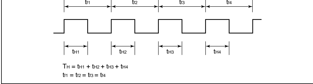
Figure 11.2 Waveform Output by 10-Bit PWM
