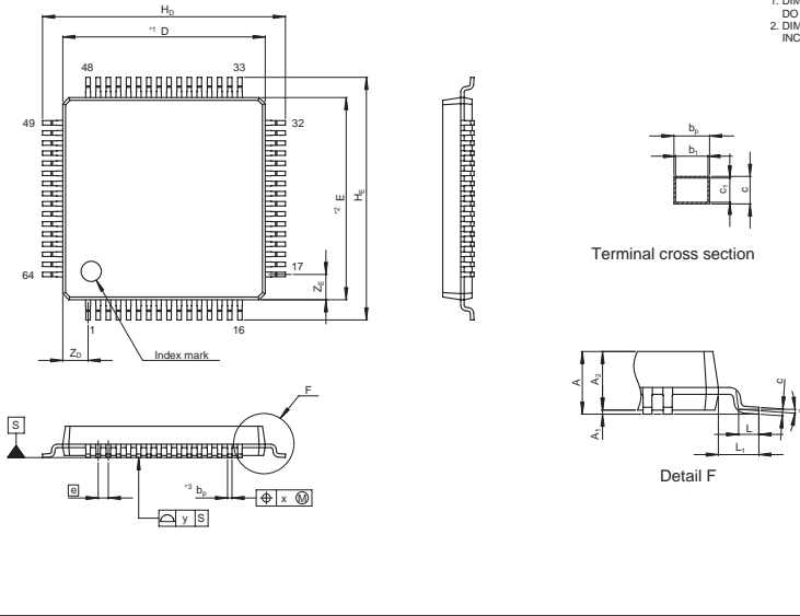
Figure E.2 Package Dimensions (FP-64E)
