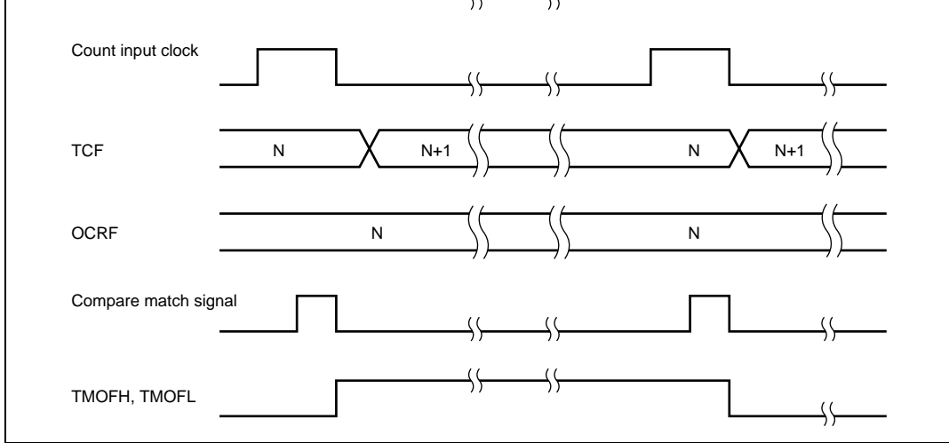
Figure 9.5 TMOFH/TMOFL Output Timing
