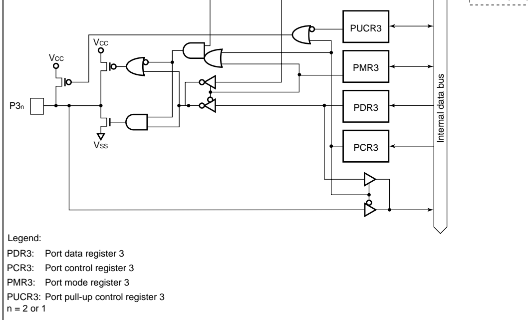
Figure B.1(d) Port 3 Block Diagram (Pins P32 and P31)
