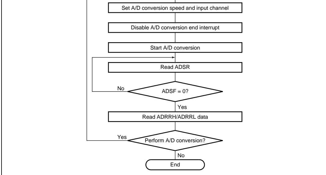
Figure 12.3 Flowchart of Procedure for Using A/D Converter (Polling by Software)
