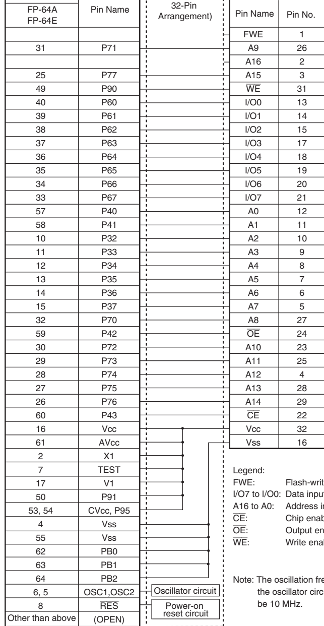
Figure 6.12(2) Socket Adapter Pin Correspondence Diagram (H8/38104F, H8/38102F)
