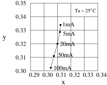
Forward Current vs. Chromaticity Coordinate ( \lambda D )
