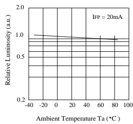
Ambient Temperature vs. Relative Luminosity
