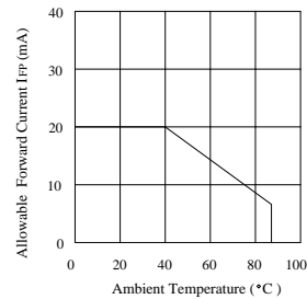
Ambient Temperature vs. Allowable Forward Current
