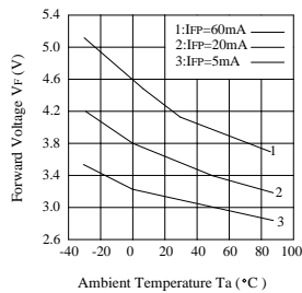
Ambient Temperature vs. Forward Voltage
