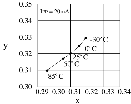
Ambient Temperature vs. Chromaticity Coordinate ( \lambda D )
