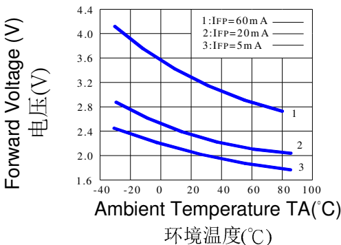
Forward Voltage Derating Curve 环境温度与电压的关系曲线图
