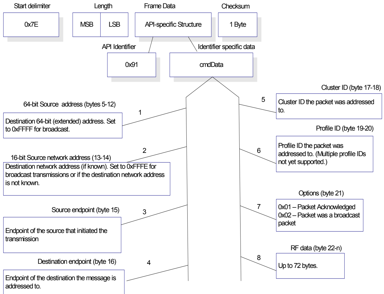
Figure 6-17. ZigBee Explicit Rx Indicators
