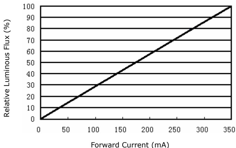
Luminous Flux VS Forward Current
