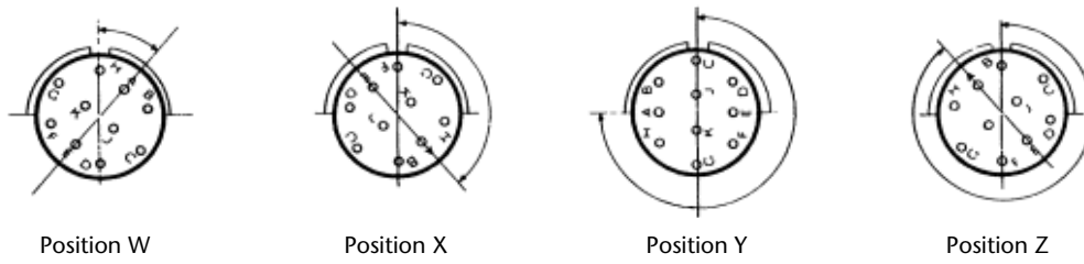
Views looking into front face of pin insert or rear of socket insert.
