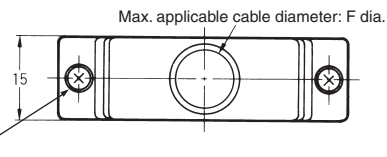
15, 25 and 37-Contact Hoods
