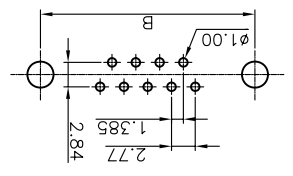
RECOMMEND PCB LAYOUT(TOLERANCE ±0.05) (VIEW FROM TOP SIDE)
