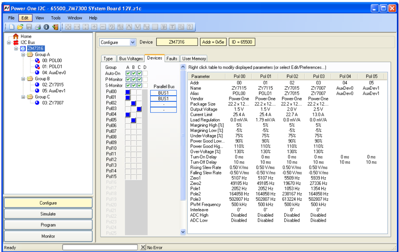
Figure 55. DPM Configure Devices Window
