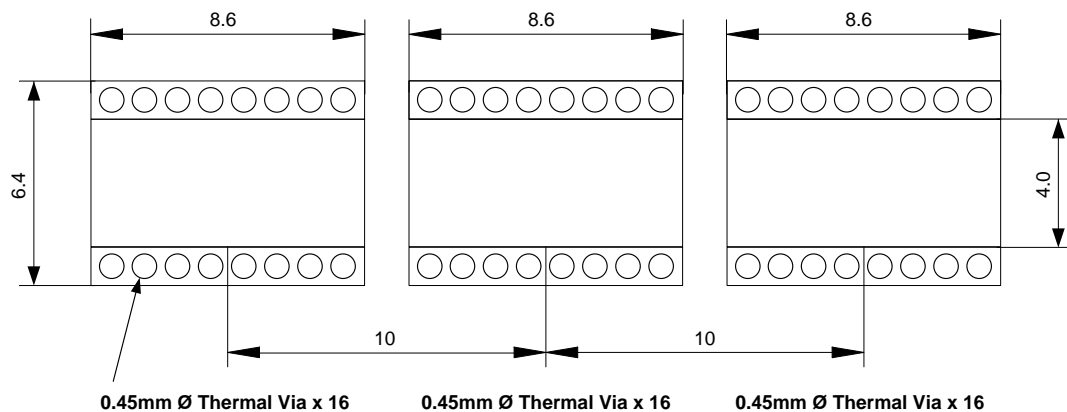
Figure 58. Recommended Pad Sizes
