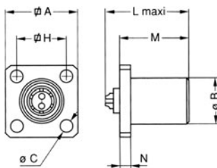
EBC Fixed socket with square flange, protruding shell and screw fixing
